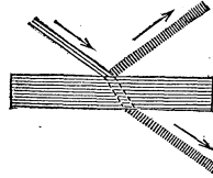
Polarized Rays.
