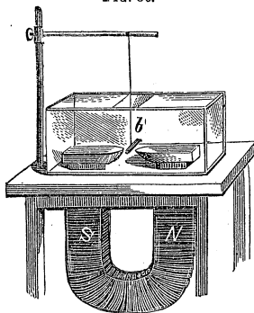
Diamagnetism.
