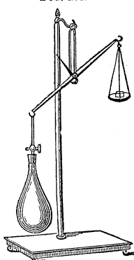
Weighing Air.
