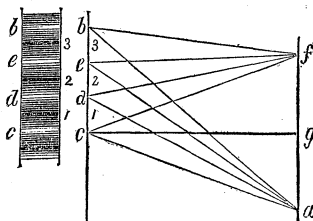
FIG. 143. Interference of Light.
