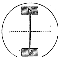
Magnetic field.
