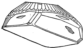
Koh-i-noor, before cutting ( side view ).
