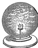
Combustion of Phosphorus.
