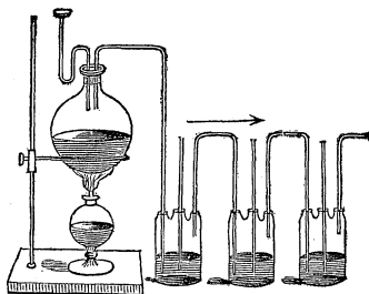
WOLFE'S BOTTLES.
