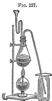
FIG. 227. Making Chlorine.
