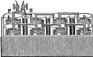
Grove's battery.
