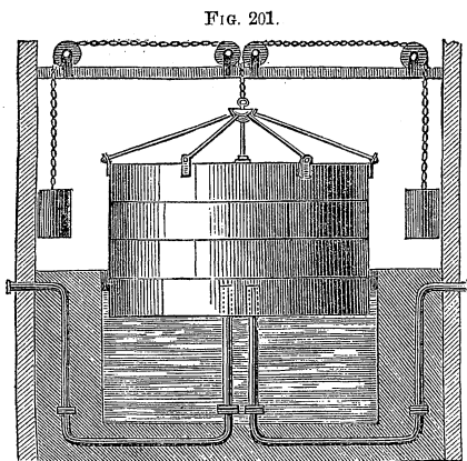
The Gasometer.
