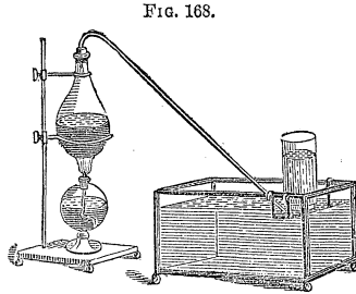
Fig. 168. Making Oxygen.
