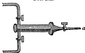
Blowpipe Jet.
