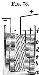
Grove's cell.
