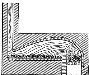
Reverberatory Furnace.
