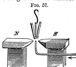
Diamagnetism of gases.
