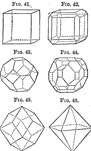
Transformations of the cube.
