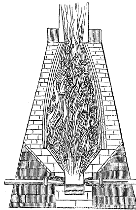
Smelting Furnace.
