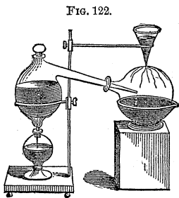
Distillation.
