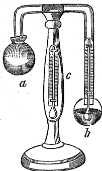
Daniell's Hygrometer.
