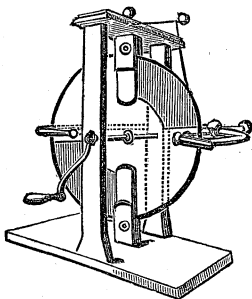
Electrical machine.
