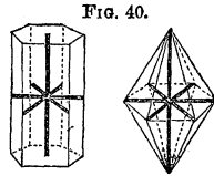
Rhombohedral system.
