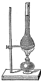
Expansion of a liquid.
