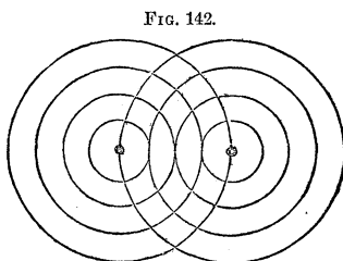
Interference of Water Waves.
