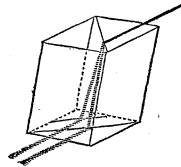
Double Refraction.
