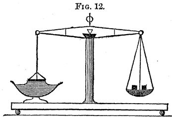
Attraction of glass and mercury.
