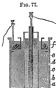
Daniell's cell.
