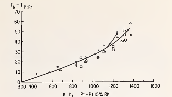
FIGURE 7. Thermal noise estimated temperature minus Pt-Pt 10 percent Rh indicated temperature, versus Pt-Rh indicated temperature at 40 kbar; falling T only.
