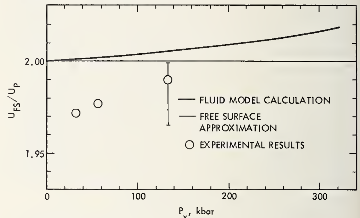
FIGURE 7. The ratio of free surface-to-particle velocity.
