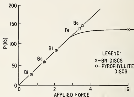
FIGURE 11. Cell pressure anomaly in Drickamer apparatus due to phase collapse of BN disks.
