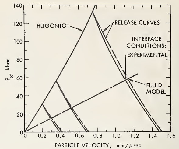
FIGURE 6. Hugoniot and release curves in the stress-versus-particle velocity plane showing the difference in the interface condition between the duraluminum sample holder and a sample with dynamic impedance \rho_0 U_s for isentropic and measured release curves.
