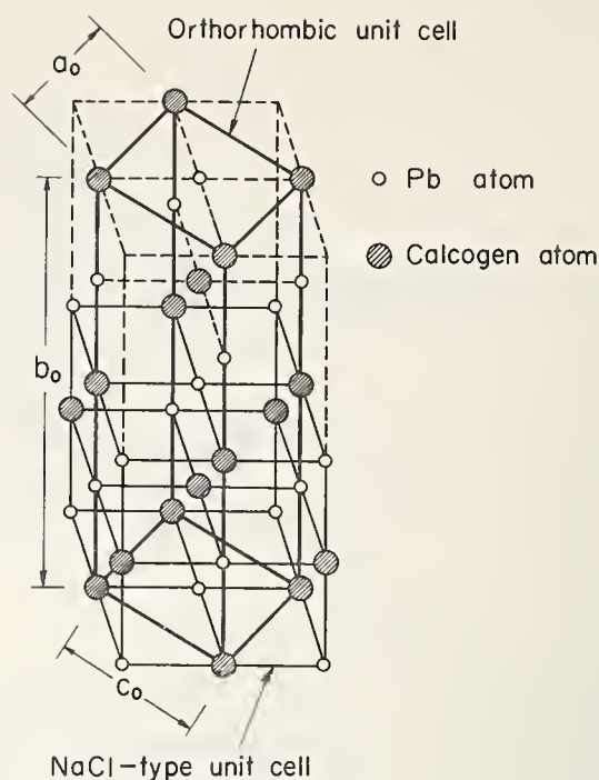
FIGURE 1. NaCl-type and orthorhombic unit cells.
