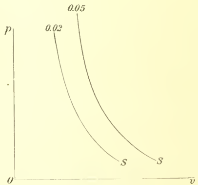
FIG. 4.—Dew-point curve.
