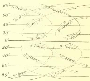
FIG. 1.—Wind currents.
