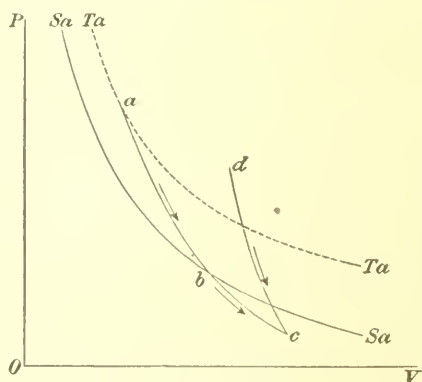
FIG. 5.—Adiabatics.
