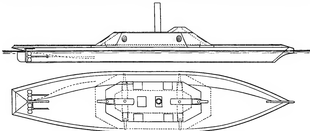
PLAN OF THE "ALBEMARLE."
