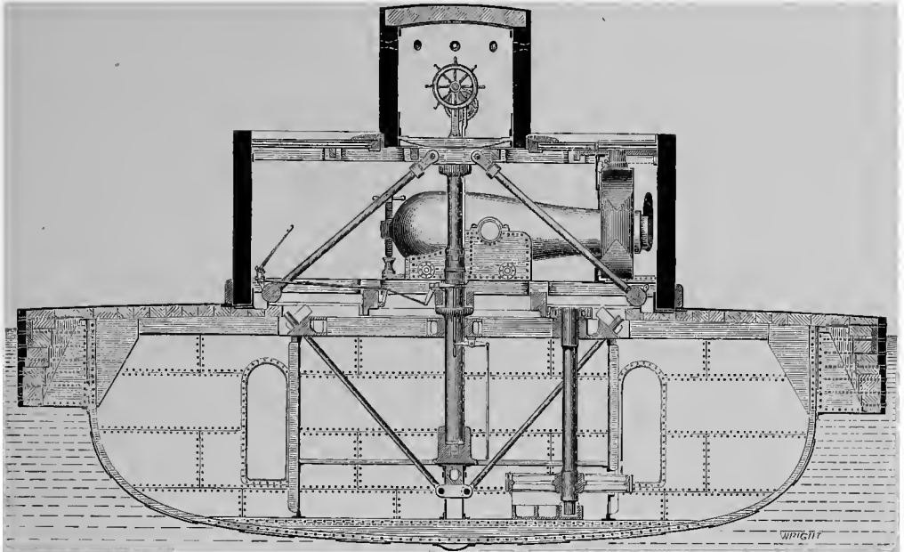
SECTION OF THE HULL OF A SEA-GOING MONITOR.
