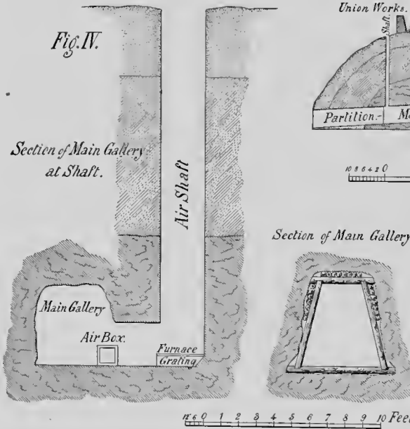
DETAILS OF THE MINE.
