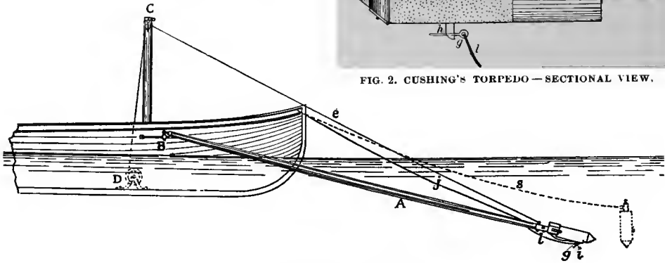
FIG. 1. CUSHING'S LAUNCH AND TORPEDO—SHOWING METHODS OF WORKING.
