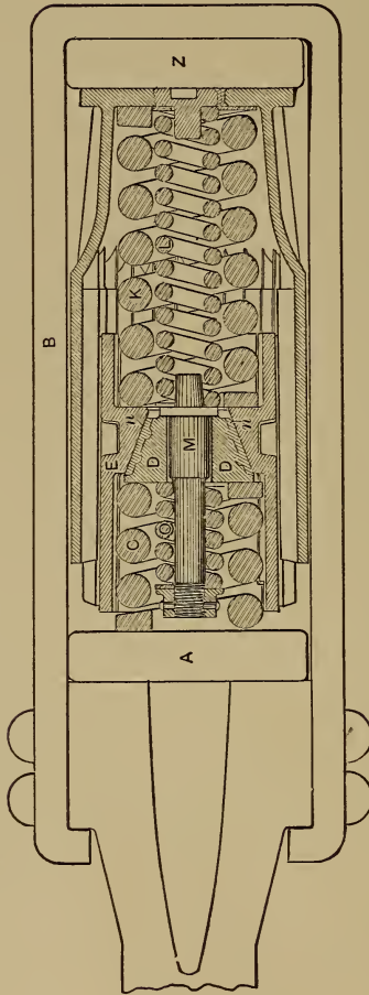
FIG. 8.—Longitudinal section of Westinghouse friction draft-gear.
