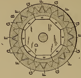
FIG. 9.—Cross-section.
