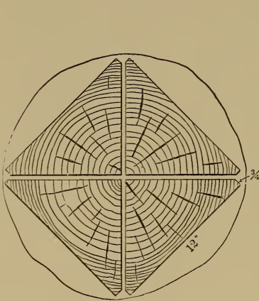
FIG. 18.—Method of cutting four triangular ties from one tree.
