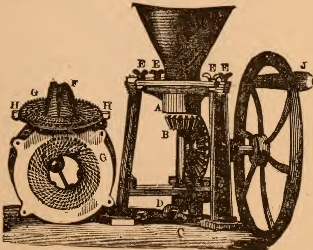
The New Style Drug Mill. Strong and effective, can be readily taken apart and cleaned.
