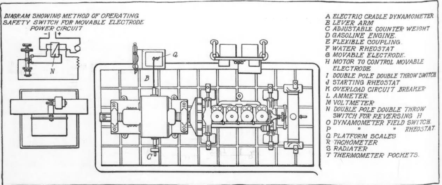
FIG. 1—PLAN DRAWING OF MOTOR YOKED TO AN ELECTRIC DYNAMOMETER
