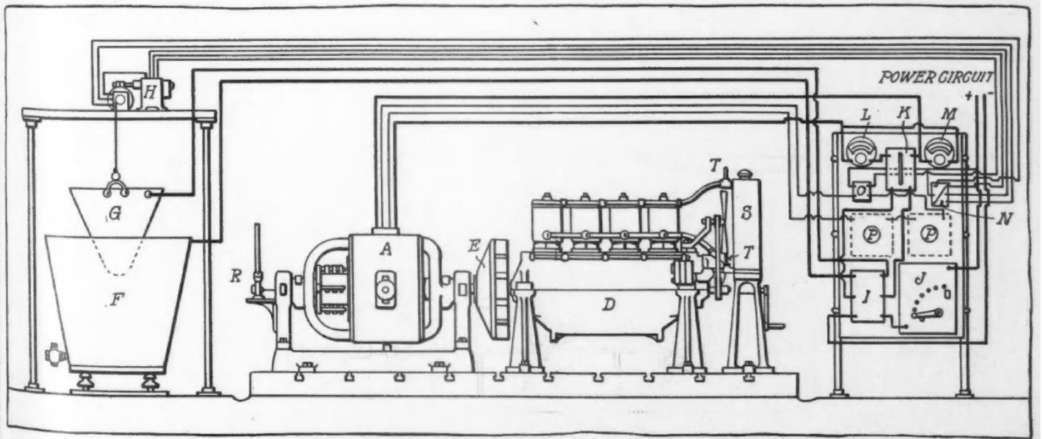
FIG. 1—ELEVATION DRAWING OF MOTOR YOKED TO AN ELECTRIC DYNAMOMETER
