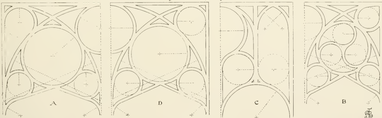
Centres of Tracery 1/4 full size
