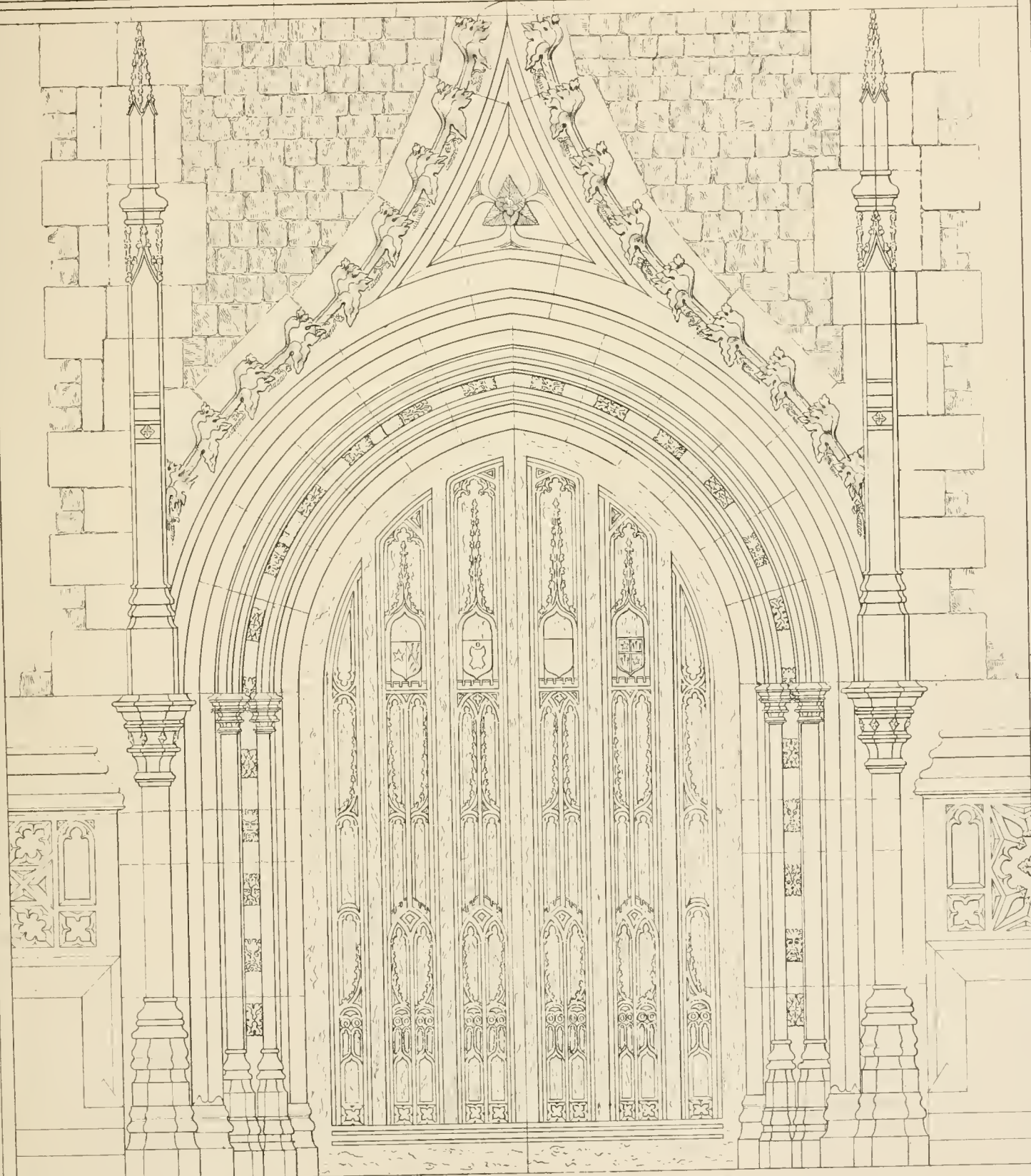
West Doorway in Tower Lavenham Church 5/11/16 22/2
