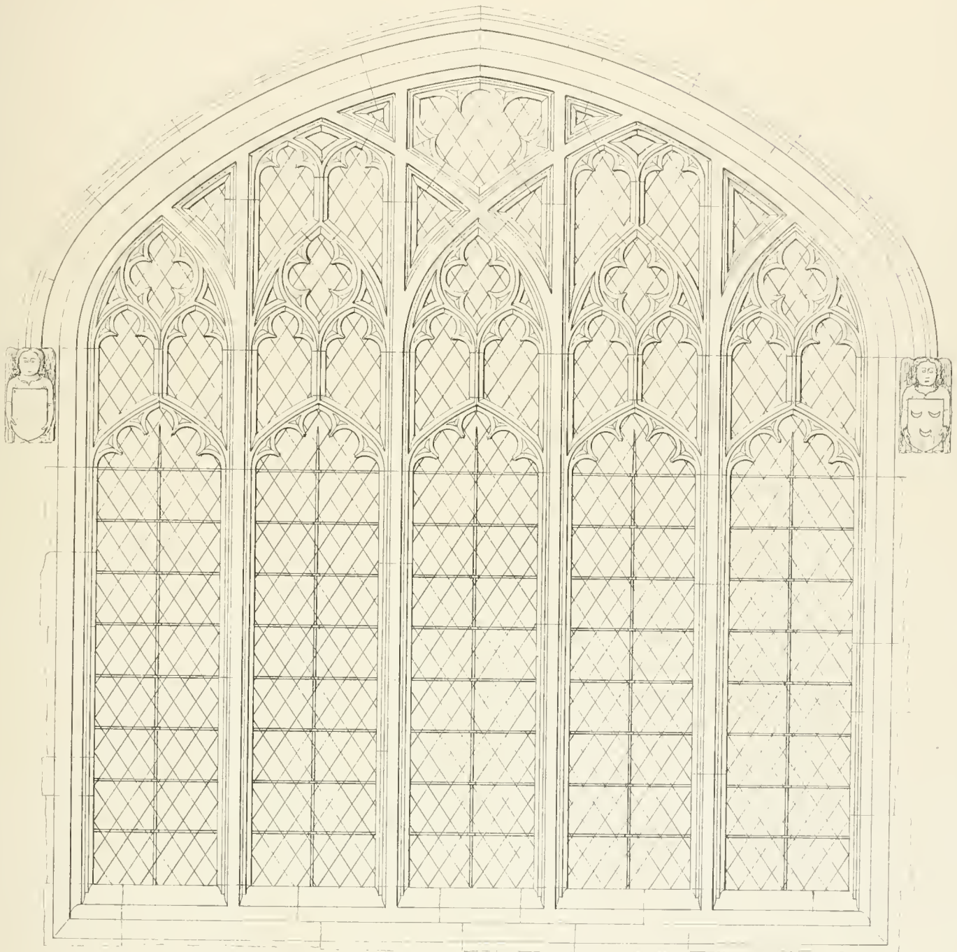
Window south of S Transept, Little Stelford Church, Cambridgeshire.
