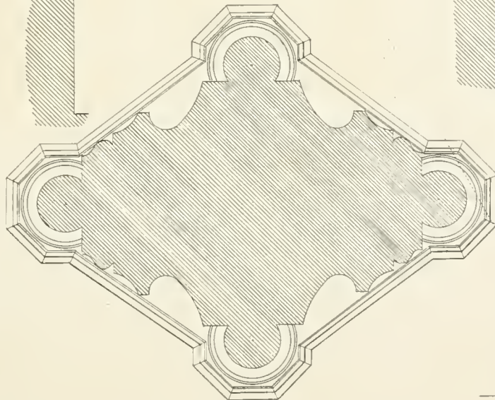
Plan of pier, inch scale
