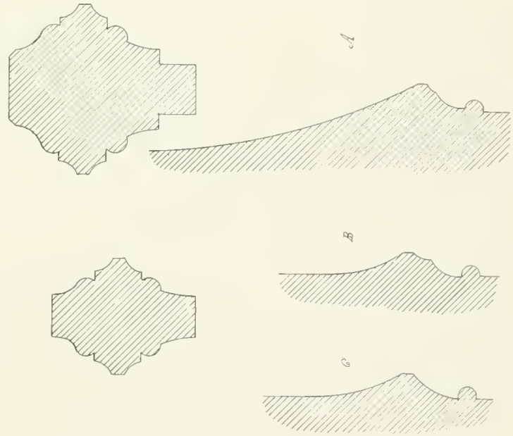
Section BC
