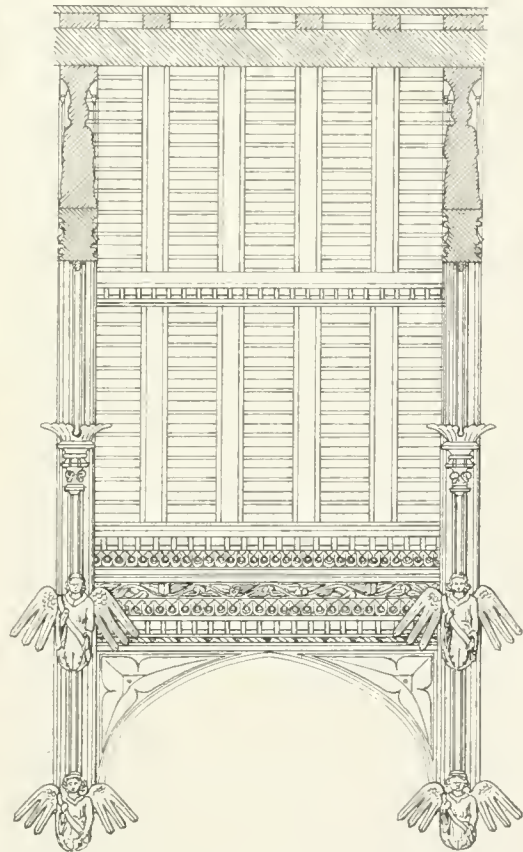
Roof over the nave of Grandisburg Ch Suffolk with details, 1 st scale. Scale of 0 1 2 3 4 5 6 7 8 9 feet
