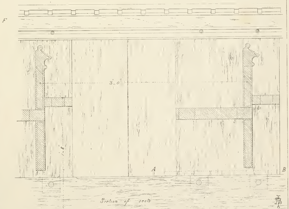
Section on line AB.
