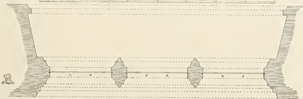
Window in North Aisle Northfleet Church Kent
