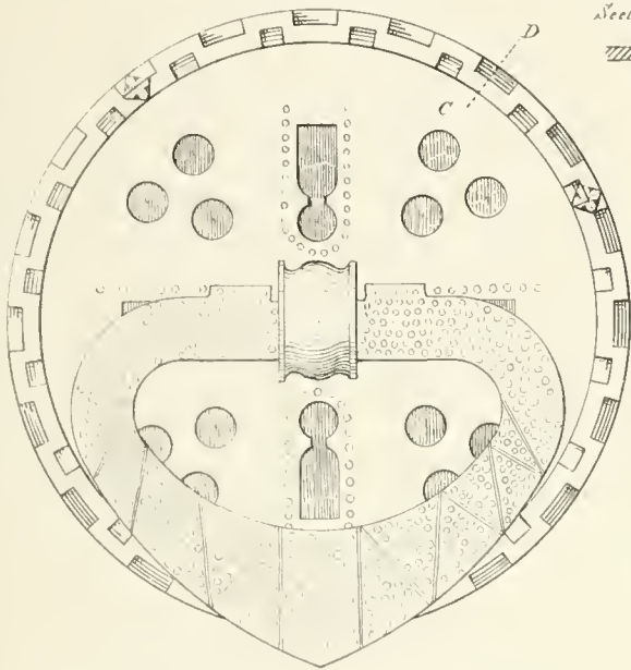
Gloucester Ch, Gloucestershire. 1/2 full size
