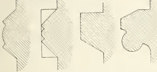
Lower basement moldings 1/2 full size
