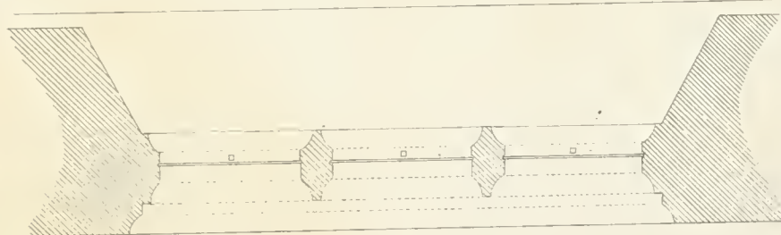
Window in S Aisle of Uffington Ch Lincolnshire
