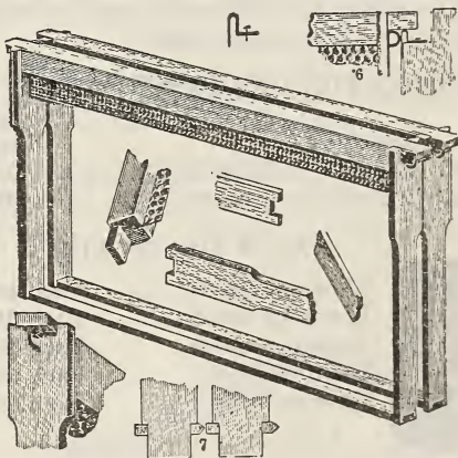
Hoffman Frames—Showing Foundation Starter
