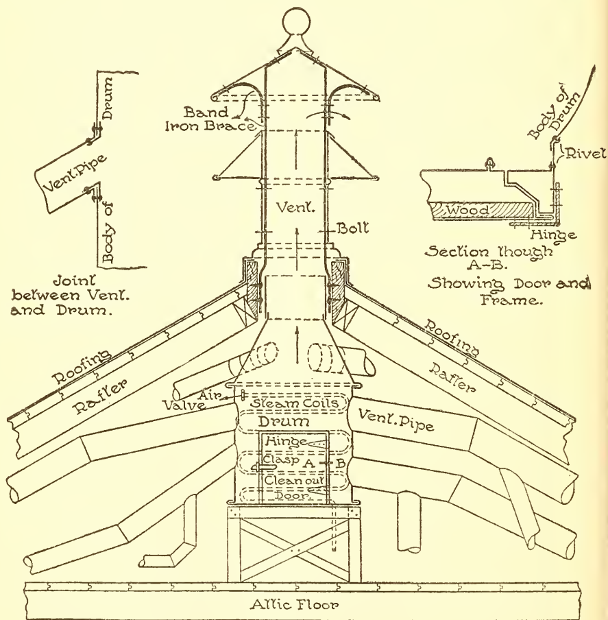
Sectional view showing ventila- tion pipes connected to drum in allie also steam coils in drum to create suction.
