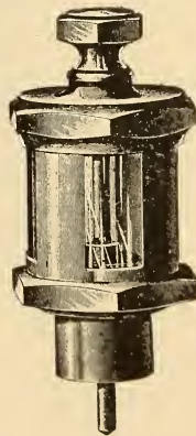
FIG. 4. Locomotive Bearing Cup for Connecting Rods.
