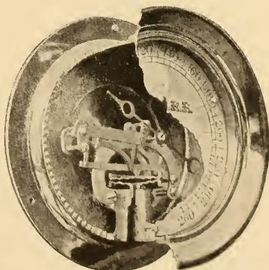
FIG. 23. Utica Locomotive Steam Gauge.
