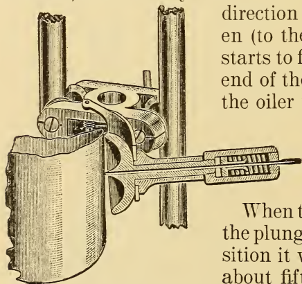
FIG. 5. Pencil Mechanism Boyer Speed Recorder.
