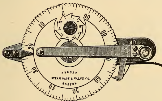
FIG. 1. Crosby Locomotive Counter.
