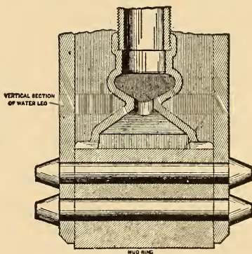
FIG. 3. Hornish Mechanical Boiler Cleaner. (Section Through Mud Ring.)
