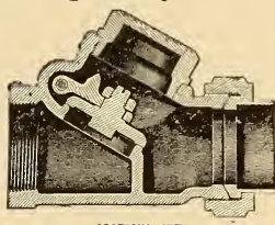
FIG. 1. Swing Intermediate or Line Check.
