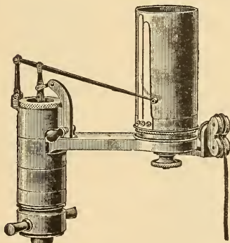
FIG. 1. The Crosby Indicator.
