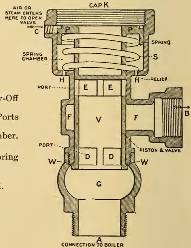
Climax Blow-Off Cock.
