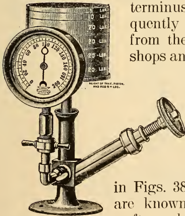
FIG. 38. Crosby Test Gauge.
