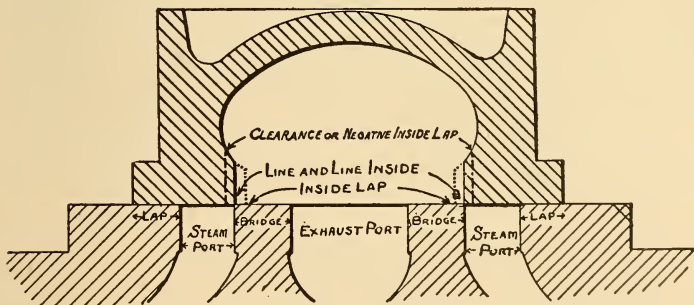
FIG. A. Graphic Definitions of Valve Dimensions. Plain Slide Valve.
