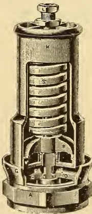
FIG. 7. Sectional View Crosby Locomotive Pop Safety Valve.
