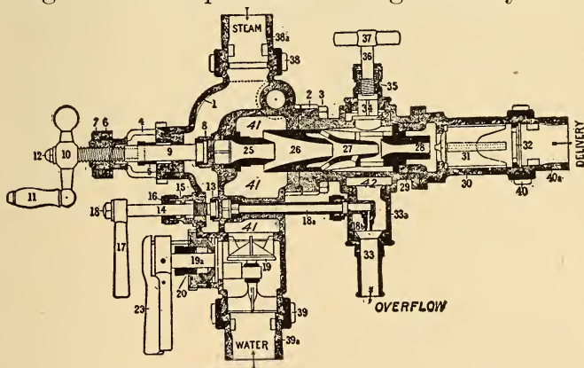
FIG. 6. Nathan "Monitor" Injector (Sectional View.)
