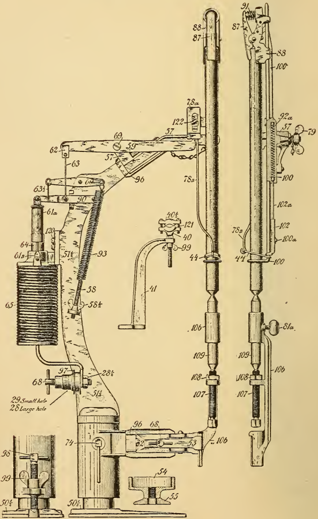
FIG. 4. Electric Headlight—Lamp "C."
