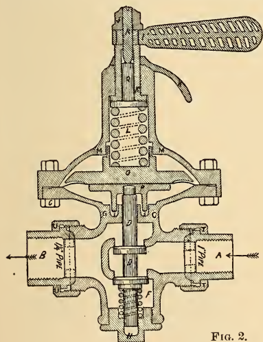
FIG. 2. Gold Pressure Regulator.
