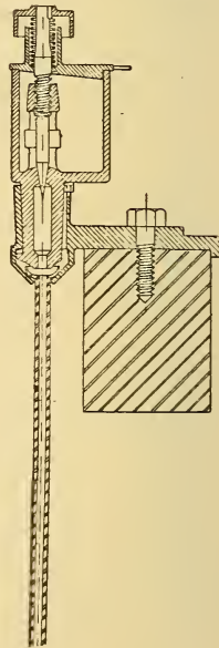
FIG. 4. Acmé Oil Cup. (Sectional View.)
