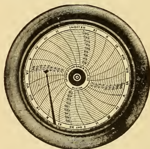
FIG. 33. Pressure Recording Gauge.
