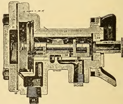
FIG. 1. Plain New York Triple Valve.
