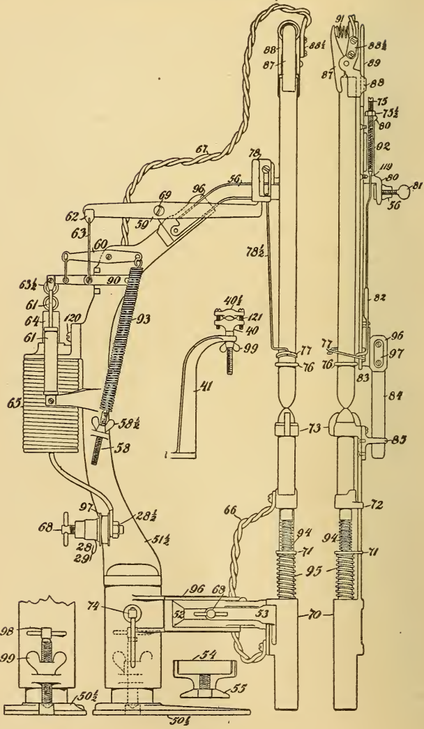
FIG. 3. Electric Headlight—Lamp "B."
