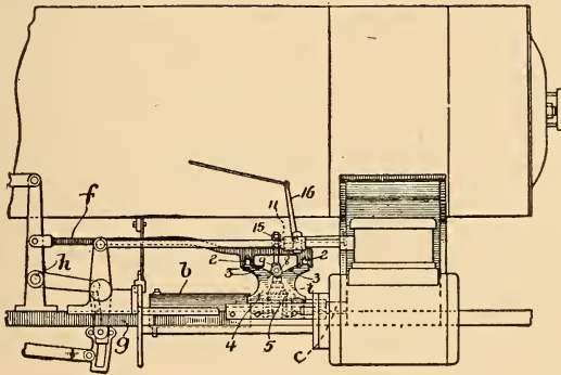
FIG 1. Huff Automatic Variable Exhaust. (Side View.)
