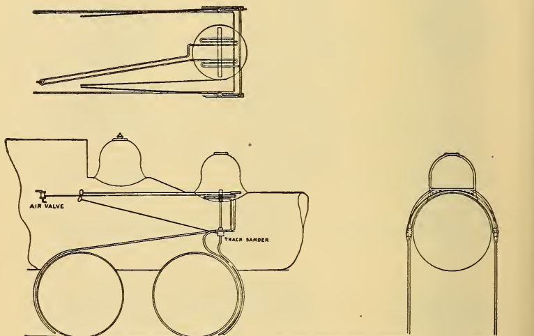
FIG. 3. Huff Pneumatic Track Sander. (Showing Application and Pipe Connections.)
