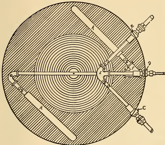
FIG. 2. The Mudd Track Sander. (Plan View.)
