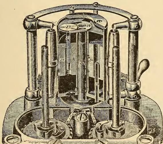
FIG. 4. Oiler—Boyer Speed Recorder.
