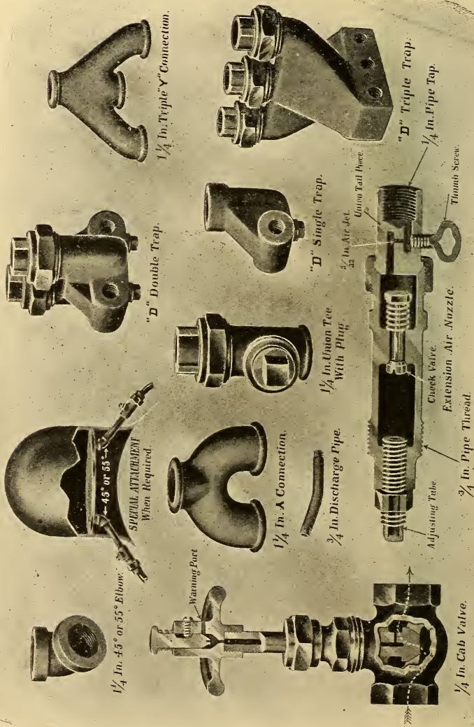
FIG. 4. Detail Parts Leach "D" Sanders.
