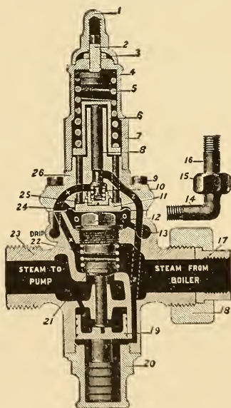
FIG. 1. Mason Air Brake Pump Regulator.
