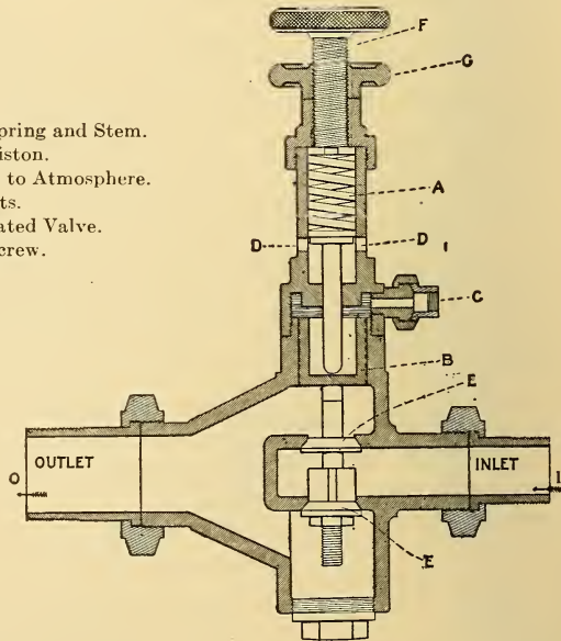
FIG. 4. Eclipse Reducing Valve.
