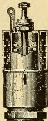
FIG. 12. Flat Top Muffler Valve with Lever.
