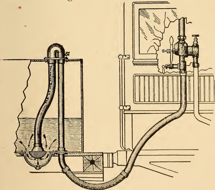
FIG. 1. Linstrom Non-Freezing Syphon Pipe.
