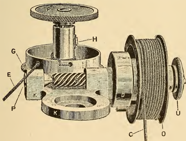
FIG. 2. Ashcroft Reducing Wheel.
