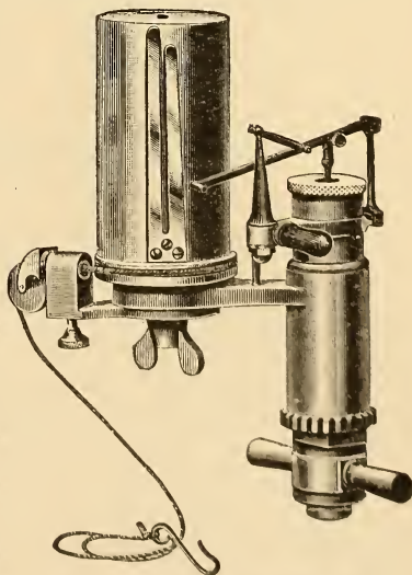
FIG. 1. The Thompson Indicator.
