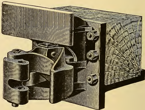
FIG. 1. Talbot Automatic Coupler for Tenders.
