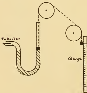
FIG. A. Mercury Column and Gauge.
