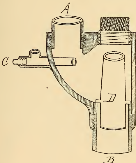
FIG. 1. A-B-C Track Sander.
