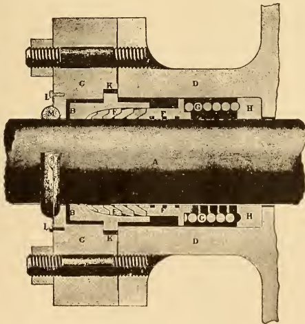
FIG. 1. Jerome Piston Rod Packing.
