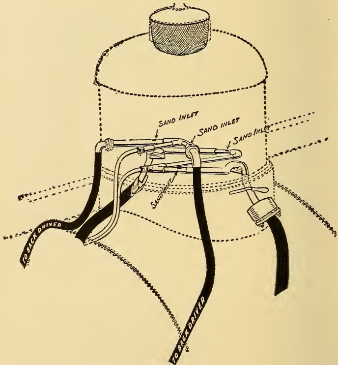
FIG. 1. The Mudd Track Sander.
