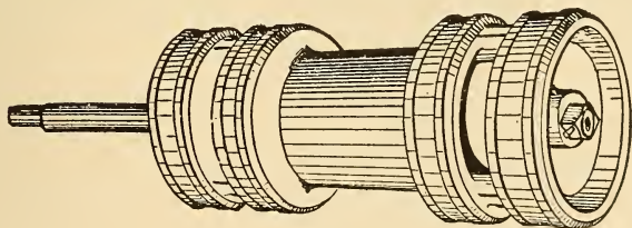
FIG. 1. Piston Valve for Baldwin Four-Cylinder Compound Locomotives.
