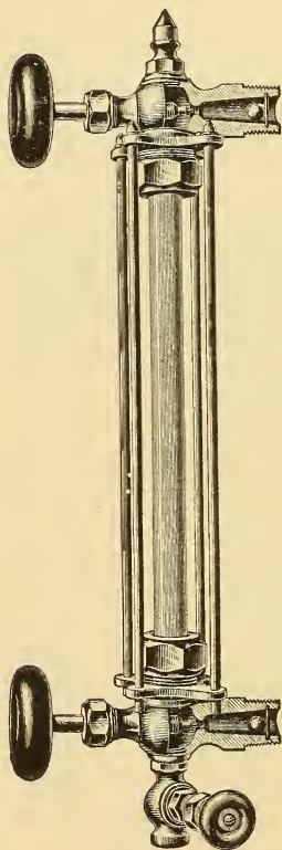
FIG. 2. Star Self-Closing Water Gauge.
