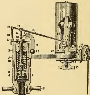
FIG. 2. The Crosby Indicator. (Sectional View.)
