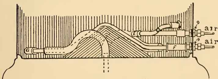
FIG. 3. The Mudd Track Sander. (Side View.)
