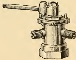
FIG. 4. Engineer's Valve—Huff Pneumatic Track Sander.
