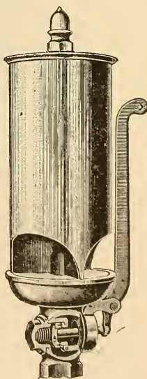
FIG. 3. Crosby Chime Whistle, Slide Valve Type.
