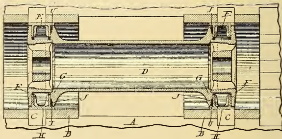
FIG. 2. Locomotive Piston Valve.
