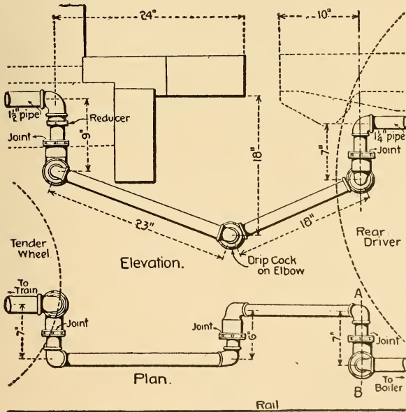
FIG. 2. Plan and Elevation of Steam Heat Conduit as applied between Locomotive and Tender.
