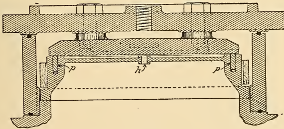
FIG. 2. Richardson Balanced Slide Valve. Transverse Section.
