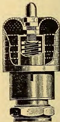
FIG. 13. Round Top Muffler Valve without Lever.
