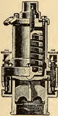
FIG. 15. Ashton Open Pop Safety Valve.
