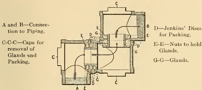
FIG. 2. Climax Flexible Metallic Joint—Double Joint.
