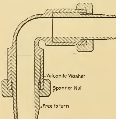
FIG. 1. Section of Swivel Joint.
