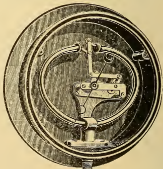
FIG. 14. Star Double-Spring Gauge—Bourdon Style.
