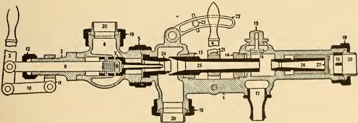
FIG. 14. Little Giant Locomotive Injector. (Sectional View.)
