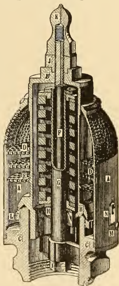
FIG. 6. Meady Muffled Locomotive Pop Safety Valve.
