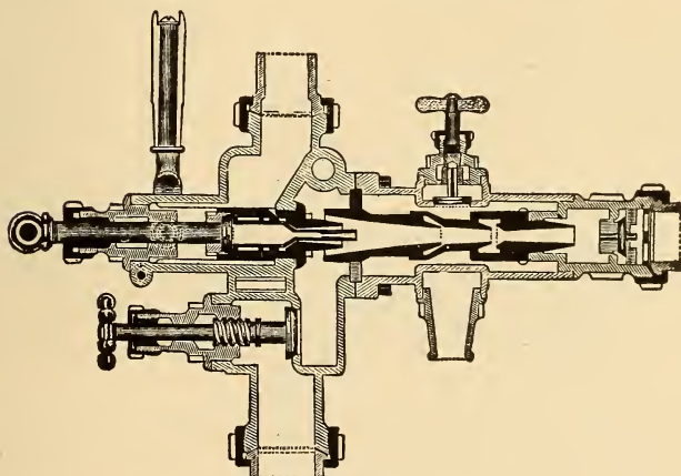
FIG. 12. The Ohio Locomotive Injector. (Sectional View).
