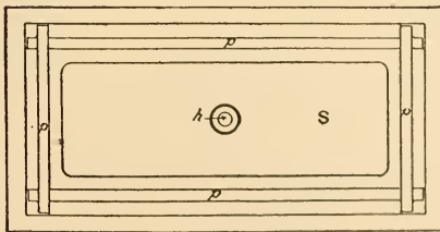
FIG. 3. Plan. Richardson Balanced Slide Valve.
