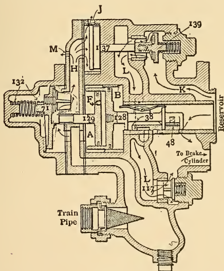
FIG. 5. Illustrative Model of New York Quick Action Triple Valve. (Valves in emergency position.)
