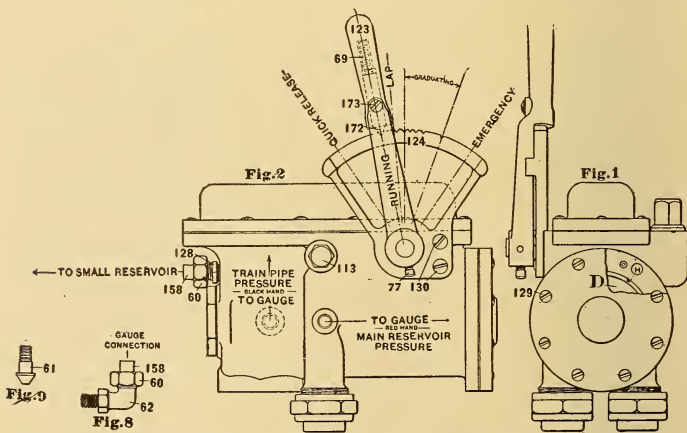
Positive Discharge Engineer's Brake Valve. New York Air Brake Co.
