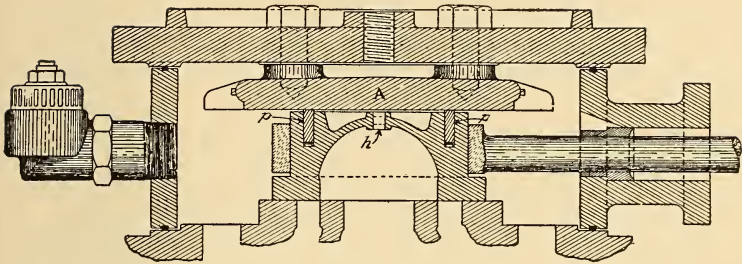
FIG. 1. Richardson Balanced Slide Valve. Longitudinal Section.
