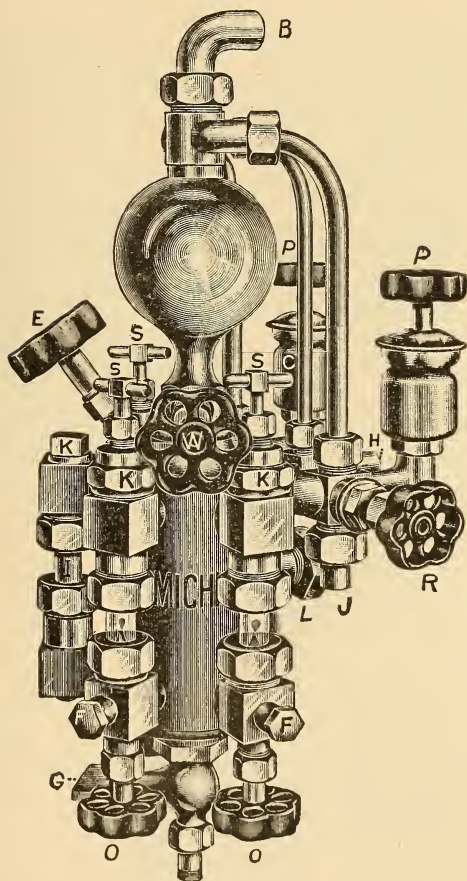
FIG. 1. Michigan Sight Feed Lubricator.
