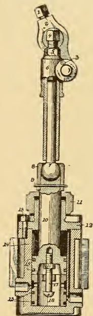
FIG. 3. Gollmar Bell Ringer. (Sectional View.)
