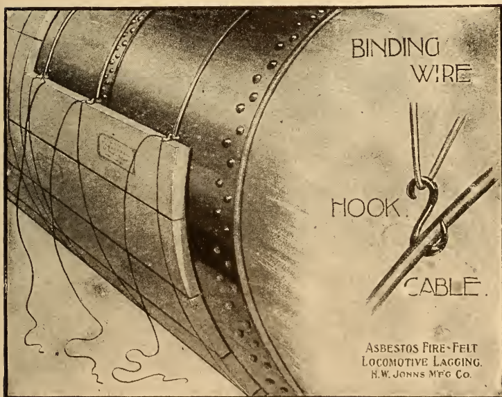
FIG. 2. Method of Securing Sectional Lagging to the Boiler.
