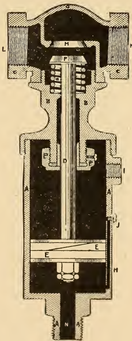
FIG. 2. Huff Automatic Steam Blower. (Sectional View.)
