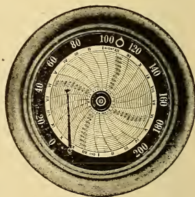
FIG. 34. Star Pressure Recording Gauge.
