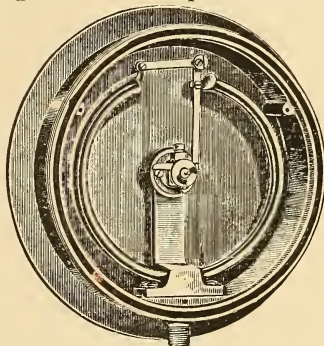
FIG. 15. Star Double-Spring Gauge—Lane Style.
