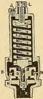
FIG. 7. Special Automatic Relief Valve.
