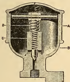
FIG. 6. Valve Stem Oil Cup.
