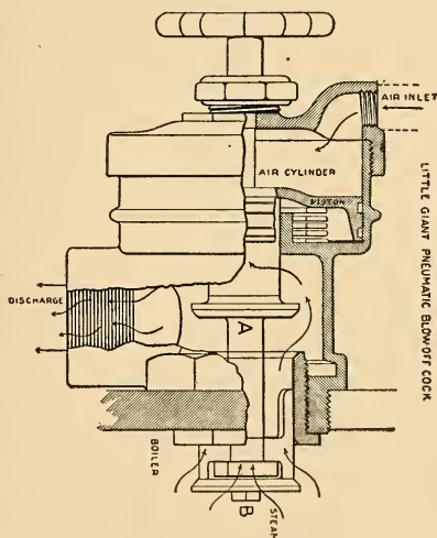
Little Giant Blow-Off Cock.
