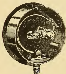
FIG. 18. Ashcroft Auxiliary Spring Locomotive Steam Gauge.
