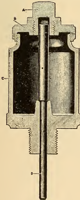
FIG. 3. Spindle Feed Rod Cup.
