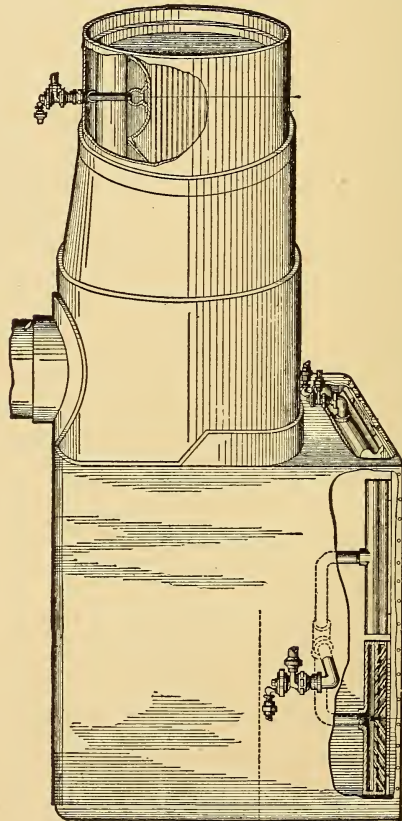
Fig. 1. Hornish Mechanical Boiler Cleaner.
