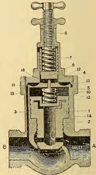
FIG. 3. Climax Steam Pressure Regulating Valve.
