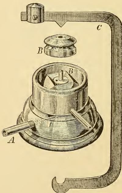
FIG. 42. The Utica Gauge Tester.
