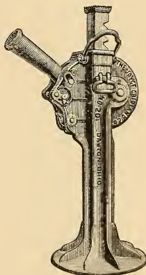
FIG. 5. Joyce Geared Locomotive Jack.
