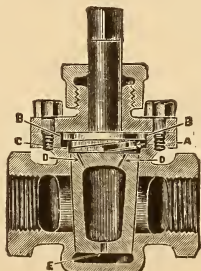
FIG 3 Homestead Straight-Way Valve.
