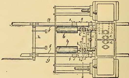
FIG. 2. Huff Automatic Variable Exhaust. (Plan View.)
