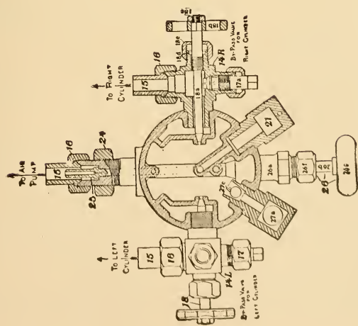
Fig. 3. Detroit Triple Feed Locomotive Lubricator. (Plan View.)
