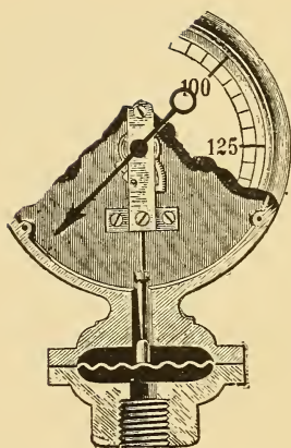
FIG. 4. Early Form of Diaphragm Gauge.
