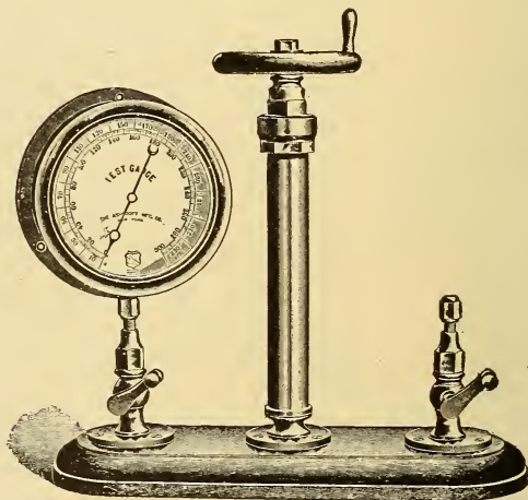
FIG. 39. Ashcroft Test Gauge.
