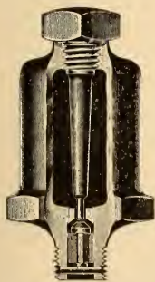
FIG. 1. Injector Oil Cup. (Sectional View.)
