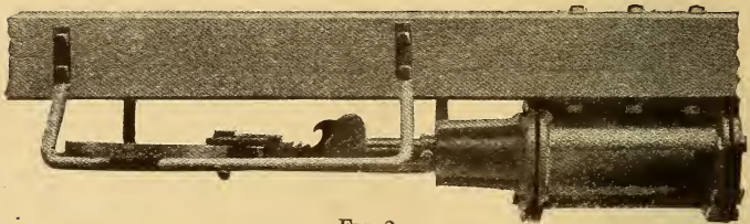
FIG. 2. Gould Brake-Slack Adjuster.
