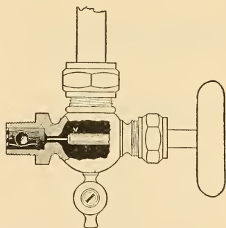
FIG. 3. Crosby Safe Water Gauge.
