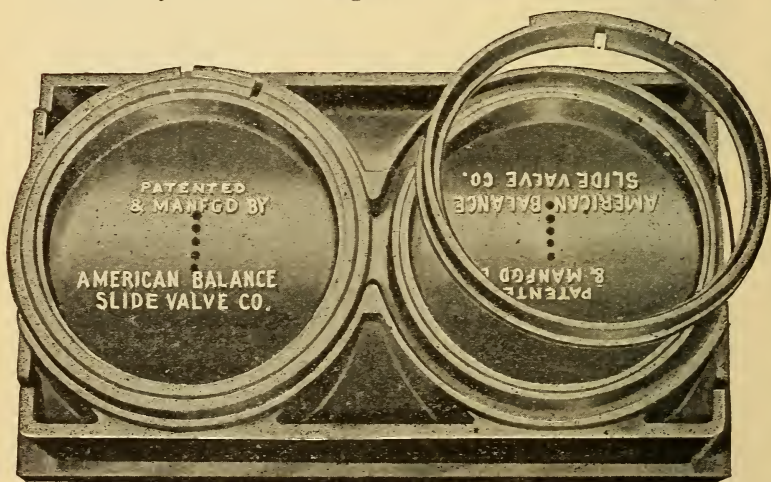
FIG. 3. Double Cone American Balance Valve.
