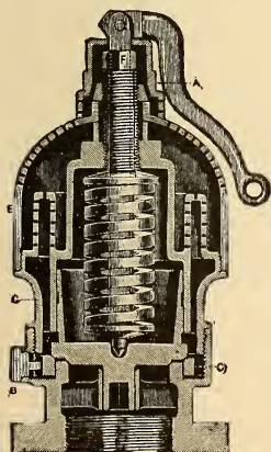
FIG. 1. The Coale Pop Safety Valve and Muffler.
