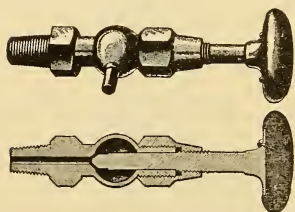
FIG. 4. Regrinding Locomotive Gauge Cock.
