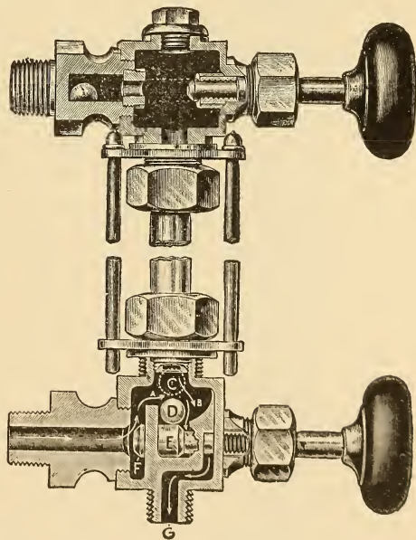
FIG. 1. Pemberthy Automatic Water Gauge.
