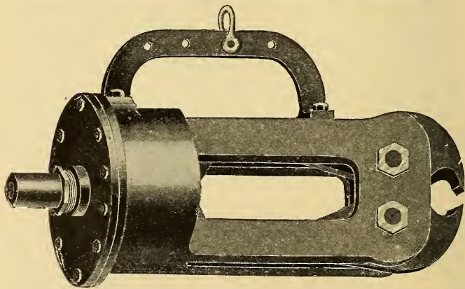
FIG. 7. "Little Giant" Stay Bolt Nipper—The stay bolt may be cut off at any length desired, as the bolt passes through the cylinder. Will cut stay bolts up to 1\frac{1}{4} inches in diameter.
