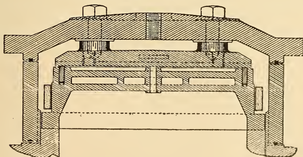
FIG. 6. Allen-Richardson Balanced Slide Valve. Transverse Section.
