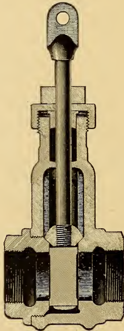
Johnstone Blow-Off Valve.
