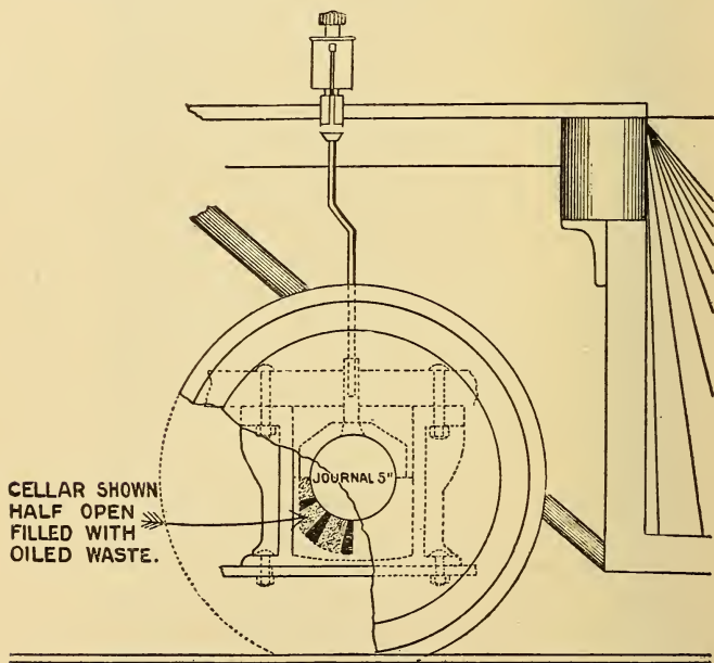
FIG. 1. Acme Engine Truck Cellar and Oil Cup.
