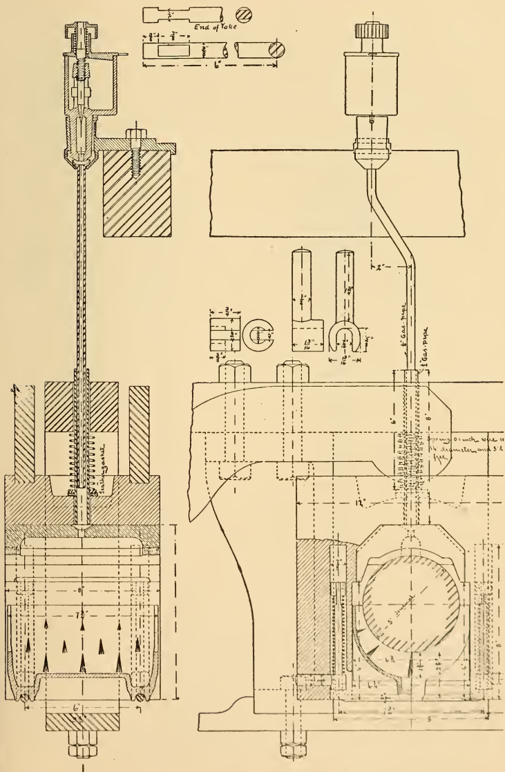
FIG. 2. Acme Automatic Engine Truck Cellar with Acme Sight-Feed Cup.
