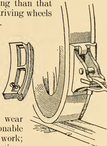
FIG. 1. Brake Shoe and Its Application to the Driver.
