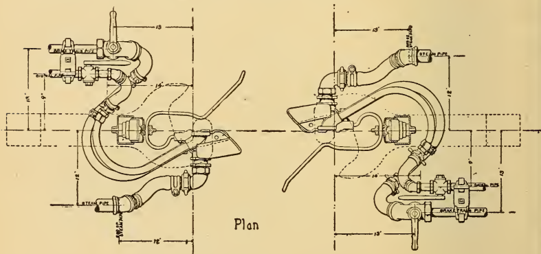
FIG. 1. Automatic Air and Steam Coupler.
