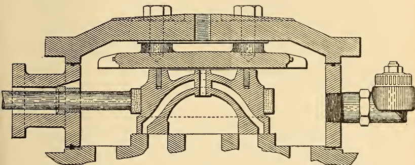
FIG. 5. Allen-Richardson Balanced Slide Valve. Longitudinal Section.
