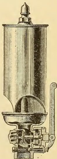
FIG. 4. Crosby Single Bell Chime Whistle.
