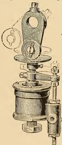
FIG. 1. Chicago Locomotive Bell Ringer.
