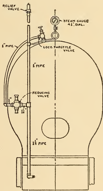
FIG. 8. Location of Steam Heating Cab Attachments.
