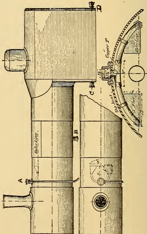
FIG. 3. McIntosh Pneumatic Blow-Off Cock, Showing Arrangement of Blow-Off Cocks on a Boiler.
