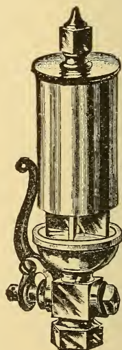
FIG. 5. Ashcroft's Four-Tone Chime Whistle.
