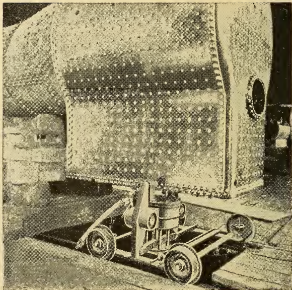
FIG. 6. Chicago Pneumatic Mud Ring Riveter Mounted on Truck.
