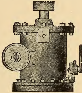
FIG. 9. Portable Air Jack.
