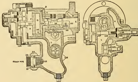
FIG. 2. New York Quick Action Triple Valve.
