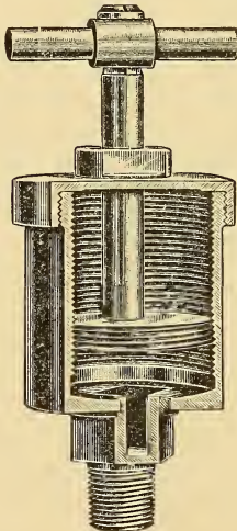
Fig. 10. Grease Cup for Rods.
