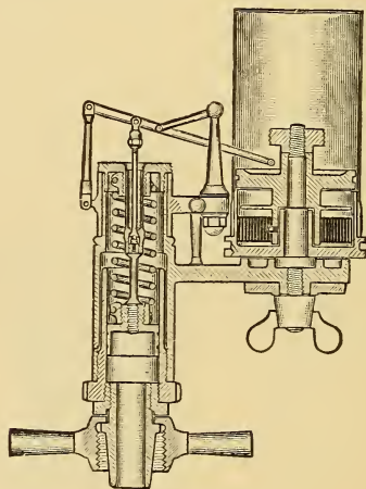
FIG. 2. The Thompson Indicator. (Sectional View.)
