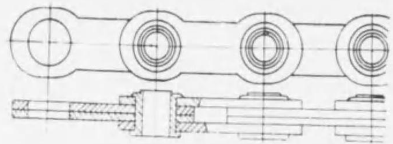
1×2 Balance Weight Chains
