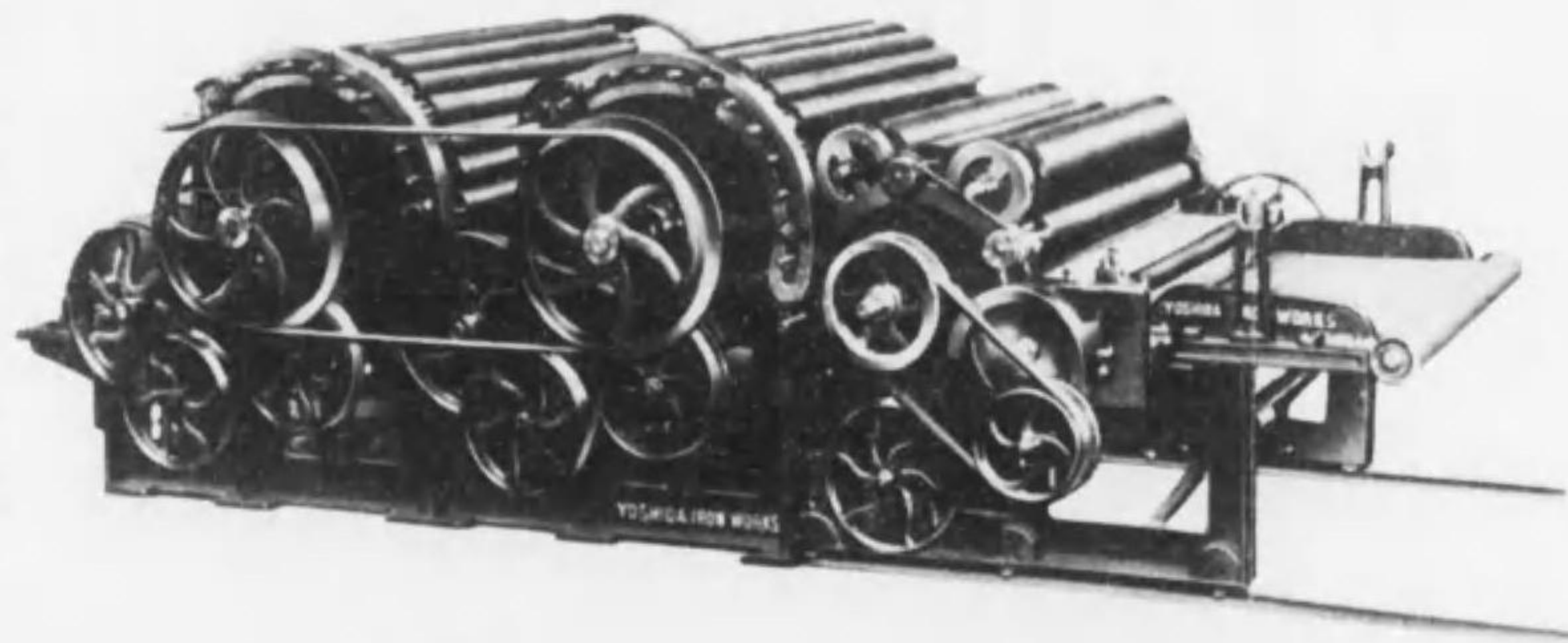
↓ GARNETT MACHINE ↑ FLY COMB
