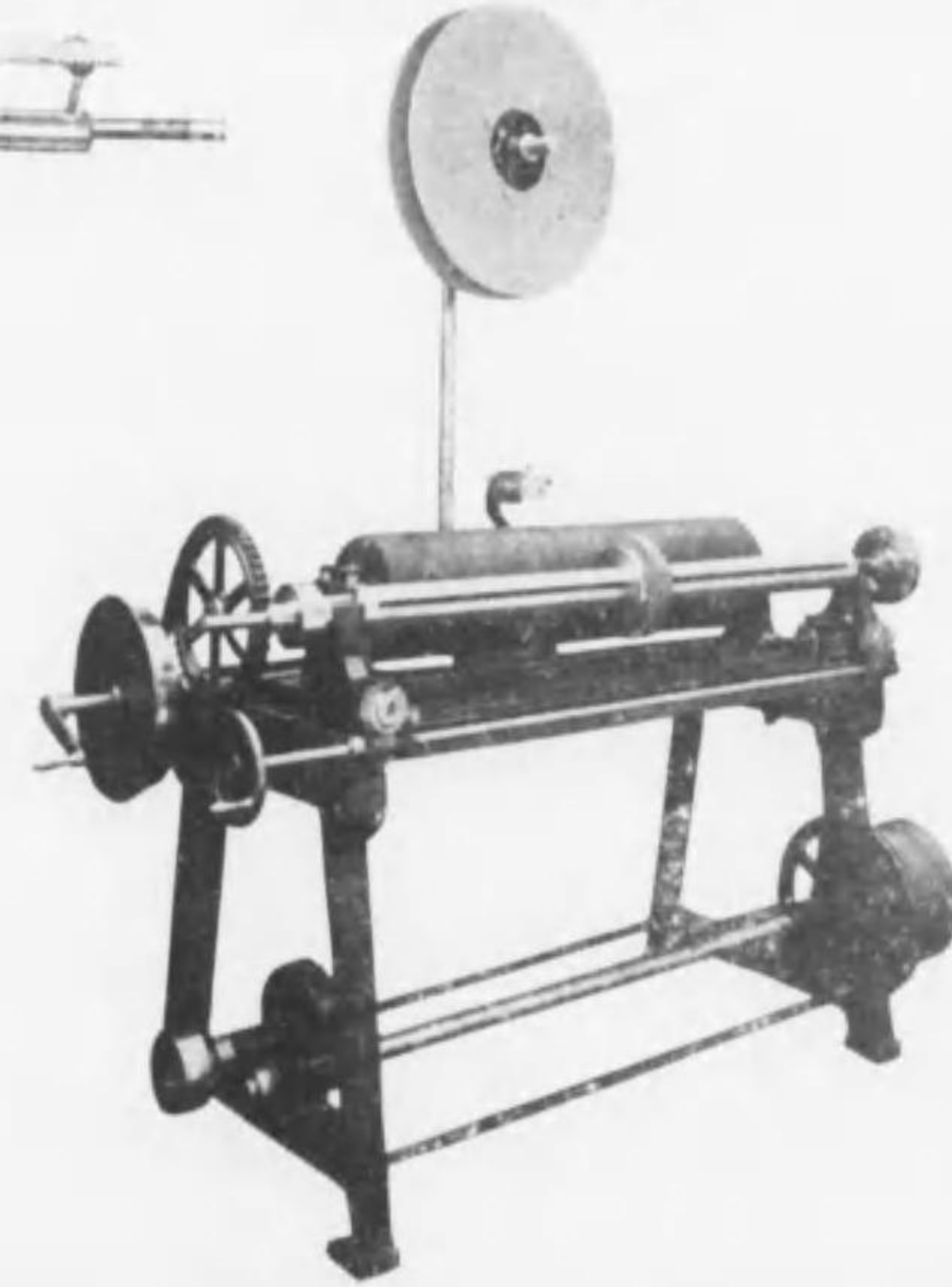
TAKER-IN MOUNTING MACHINE WITH TRAVERSE WHEEL GRINDER
