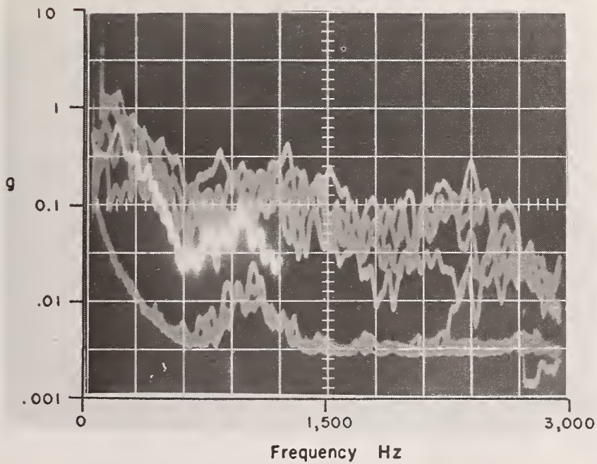
Figure 180. Multiple Sweeps of Vibrational Disturbances Produced by Abrasive Wheel Saw; Test F2 145
