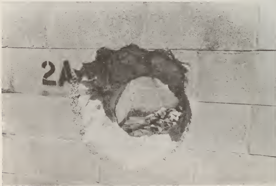
Figure 15. Attack 2A. Exterior View, Final Opening 20
