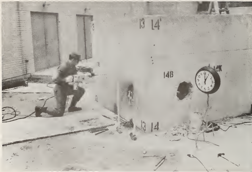
Figure 107. Test 13B. Rotohammer Drilling
