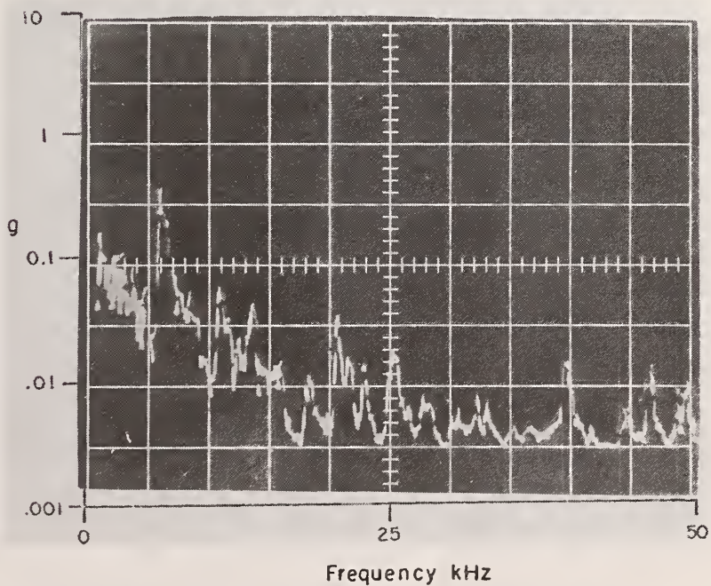
Figure 46. Vibrational Disturbances Produced by Rotohammer and 3/4" Drill; Test 6B
