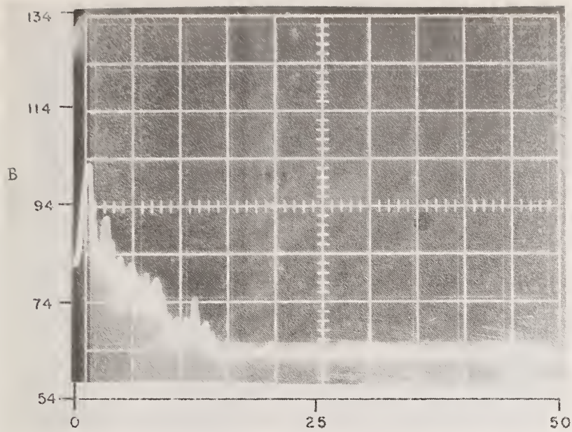
Figure 77. Acoustical Disturbances Produced by Saw; Test 9N
