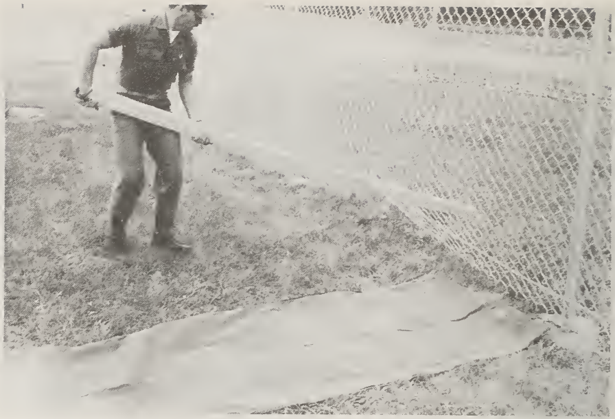
Figure 157. Fence Lifted 12" Using 2" X 4" Timber as Lever; Test F1
