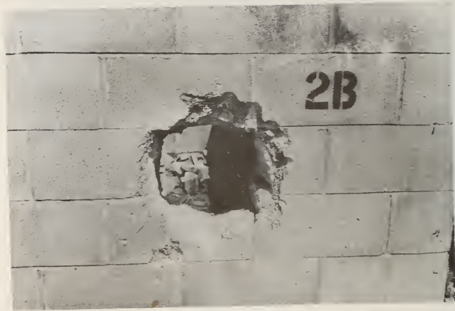
Figure 23. Exterior View, Final Enlarged Breakthrough; Test 2B
