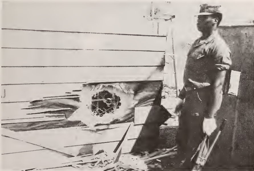
Figure 89. Test 11U. Ferro-cement Reinforcing Wire Exposed
