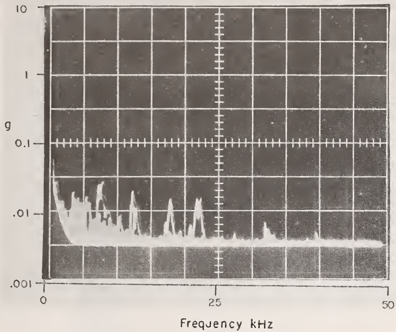
Figure 57. Vibrational Disturbances Produced by No. 14 Bolt Cutters; Test 7A
