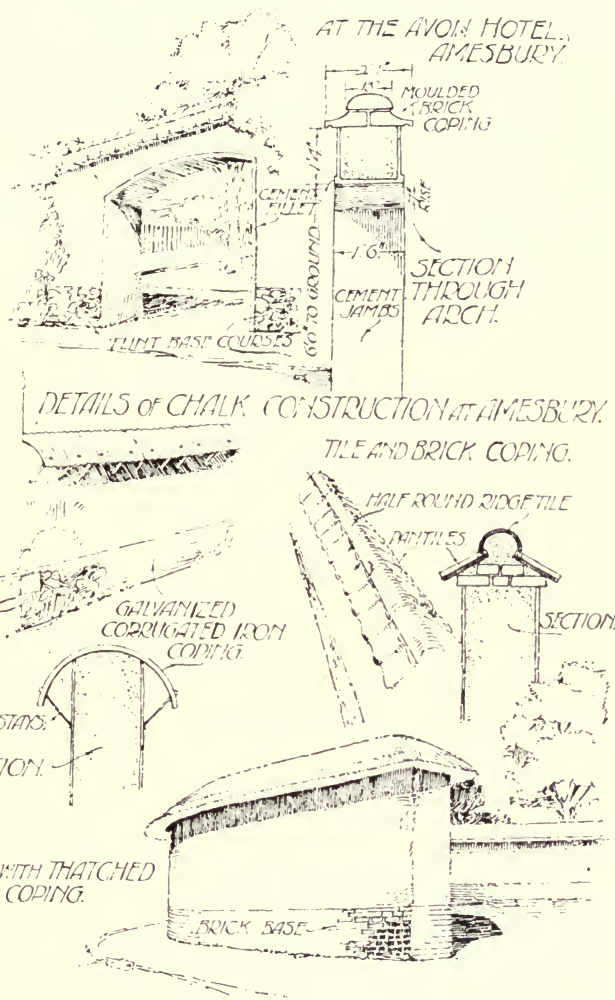
DETAILS OF CHALK CONSTRUCTION AT AMESBURY.
