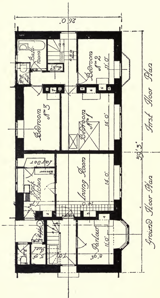
Scale of \frac{1}{4} " = 1' 0" Feet.
