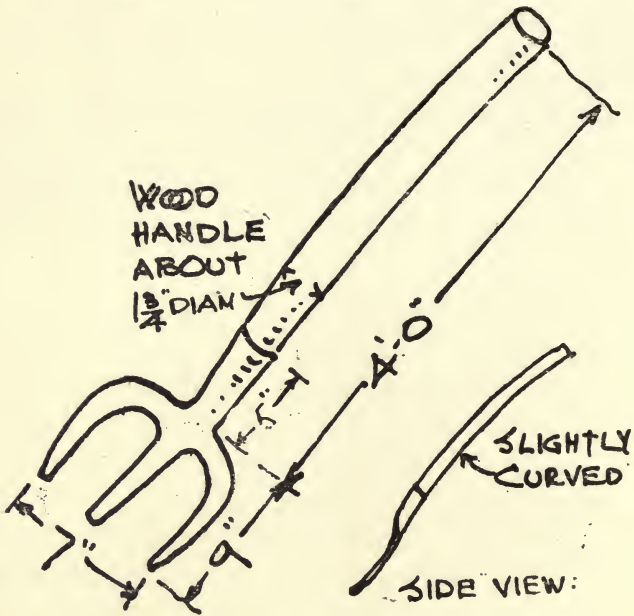
COB PICK (Measured from example at Great Fulford).
