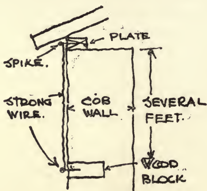
WALL COPINGS.
