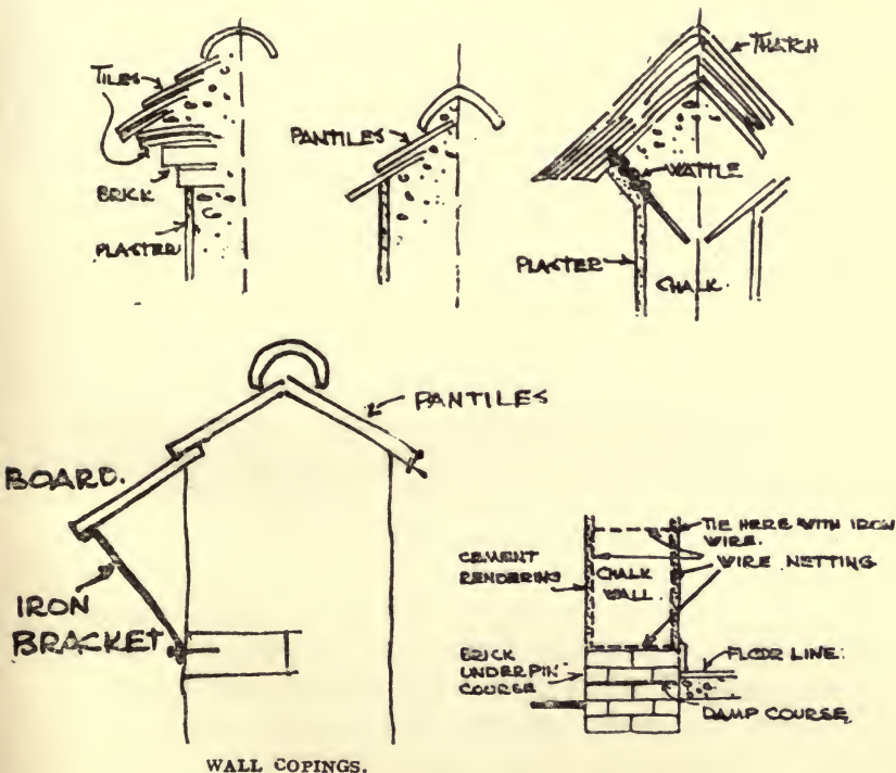
WALL COPINGS.
