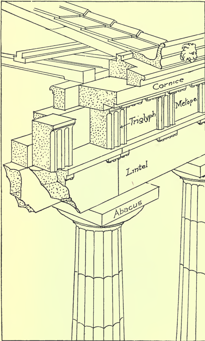
FIG. 8—GREEK STONE CONSTRUCTION
