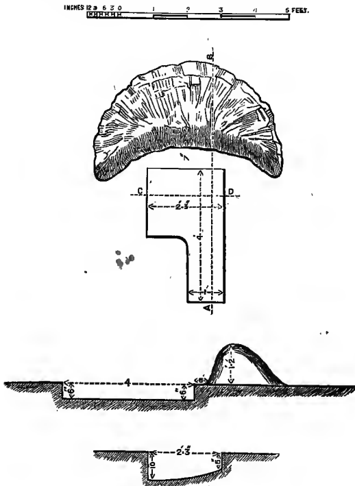
SHELTER-PIT FOR SKIRMISHERS.
