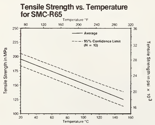
Fig. 7 - Tensile strength versus temperature for SMC-R65
