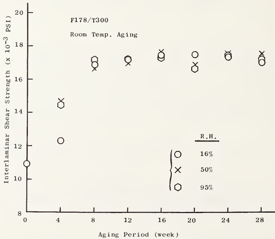
Figure 2. Interlaminar shear strength of aged samples.
