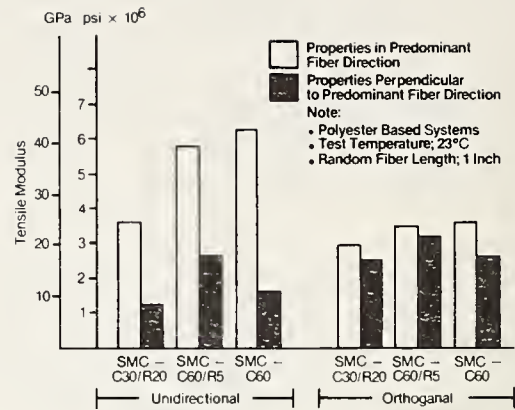
Fig. 24 - Tensile modulus values as effected by different types of SMCs, laminate construction, and fiber orientation
