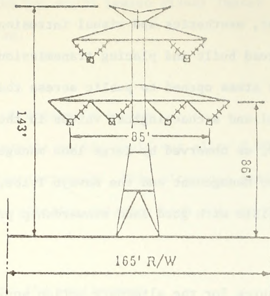
Tower 3 Double Circuit Delta Configuration
