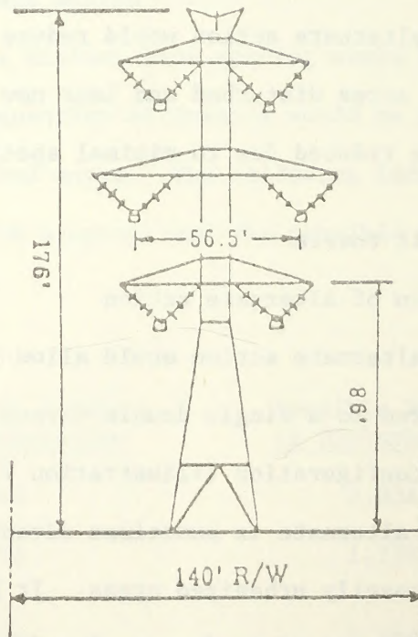
Tower 4 Double Circuit Stack Configuration
