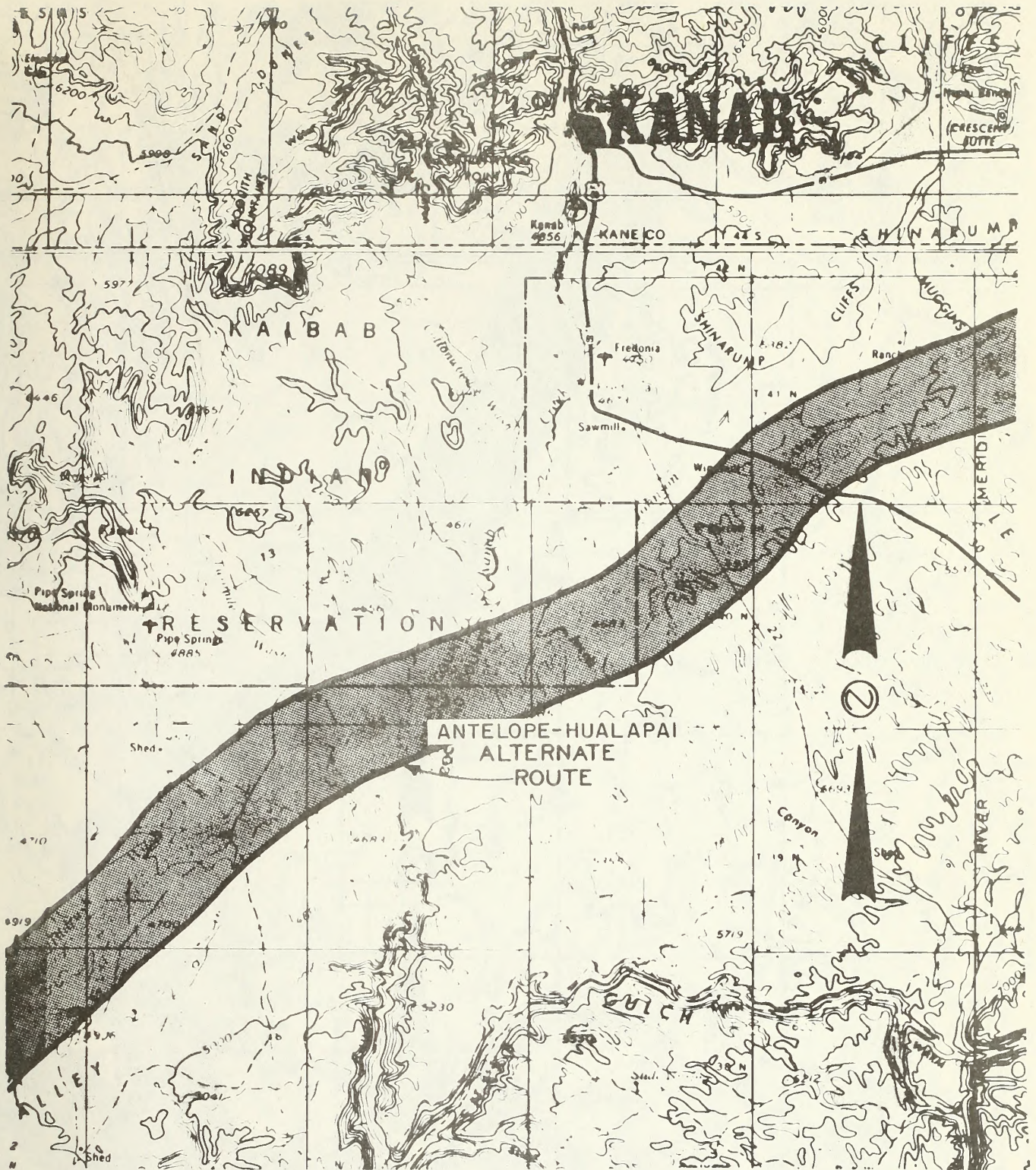
ILLUSTRATION VIII-49 Proposed Kaiparowits Transmission System Kaiparowits to Phoenix Alternate Routes (Sheet 16 of 23)
