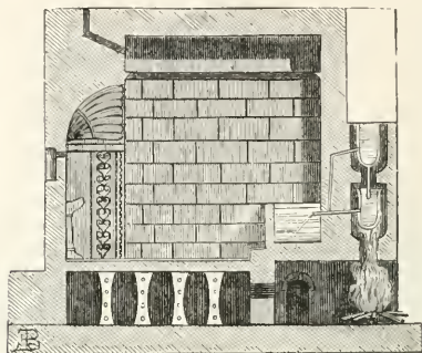
Fig. 393. Hypocaustus of a Roman villa at Tusculum.
