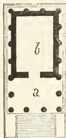
Fig. 535. Ground-plan of a pseudo-peripteral temple.
