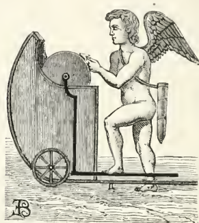
Fig. 200. Cos—a Roman Grindstone.
