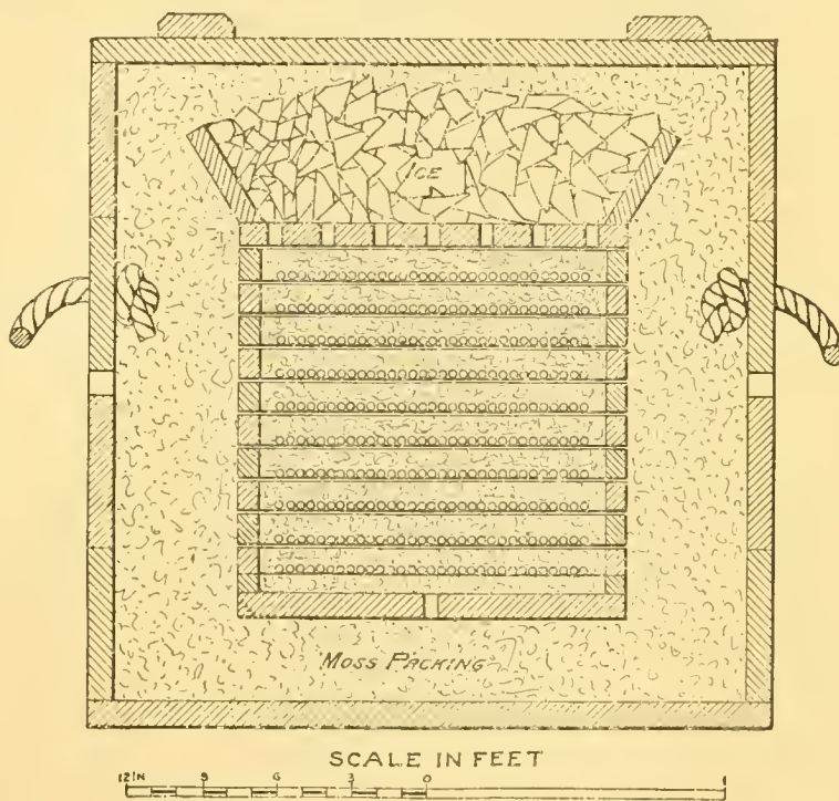
FIG. 1. Cross section through box after it has been packed and closed.
