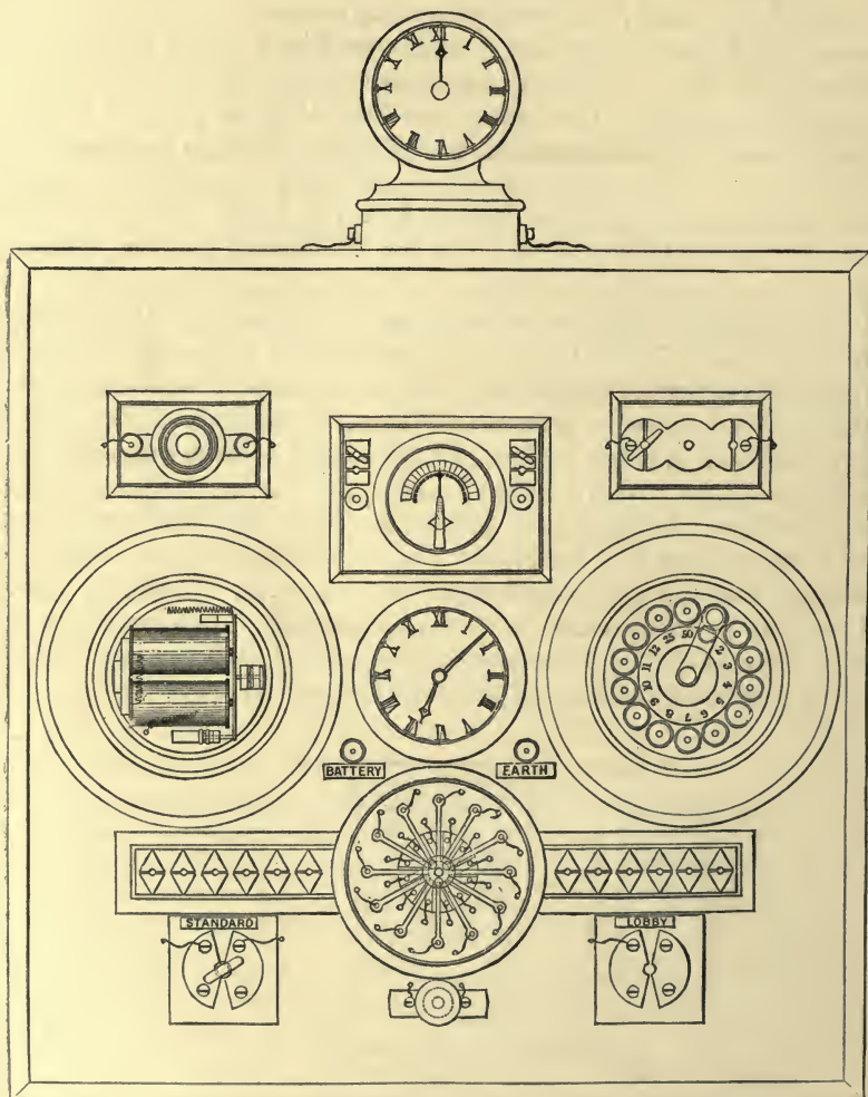
FIG. 11. —TEST-BOX.
