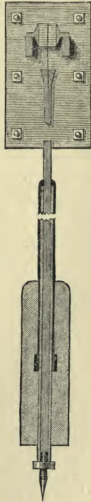
FIG. 3.—GREENWICH PENDULUM. SECTION.
