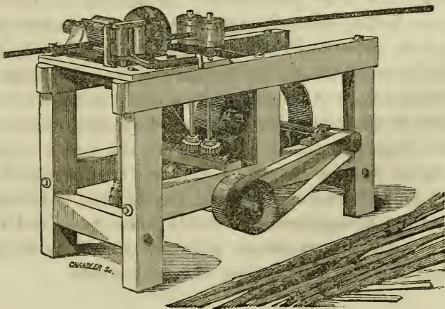
SHAVING MACHINE.
