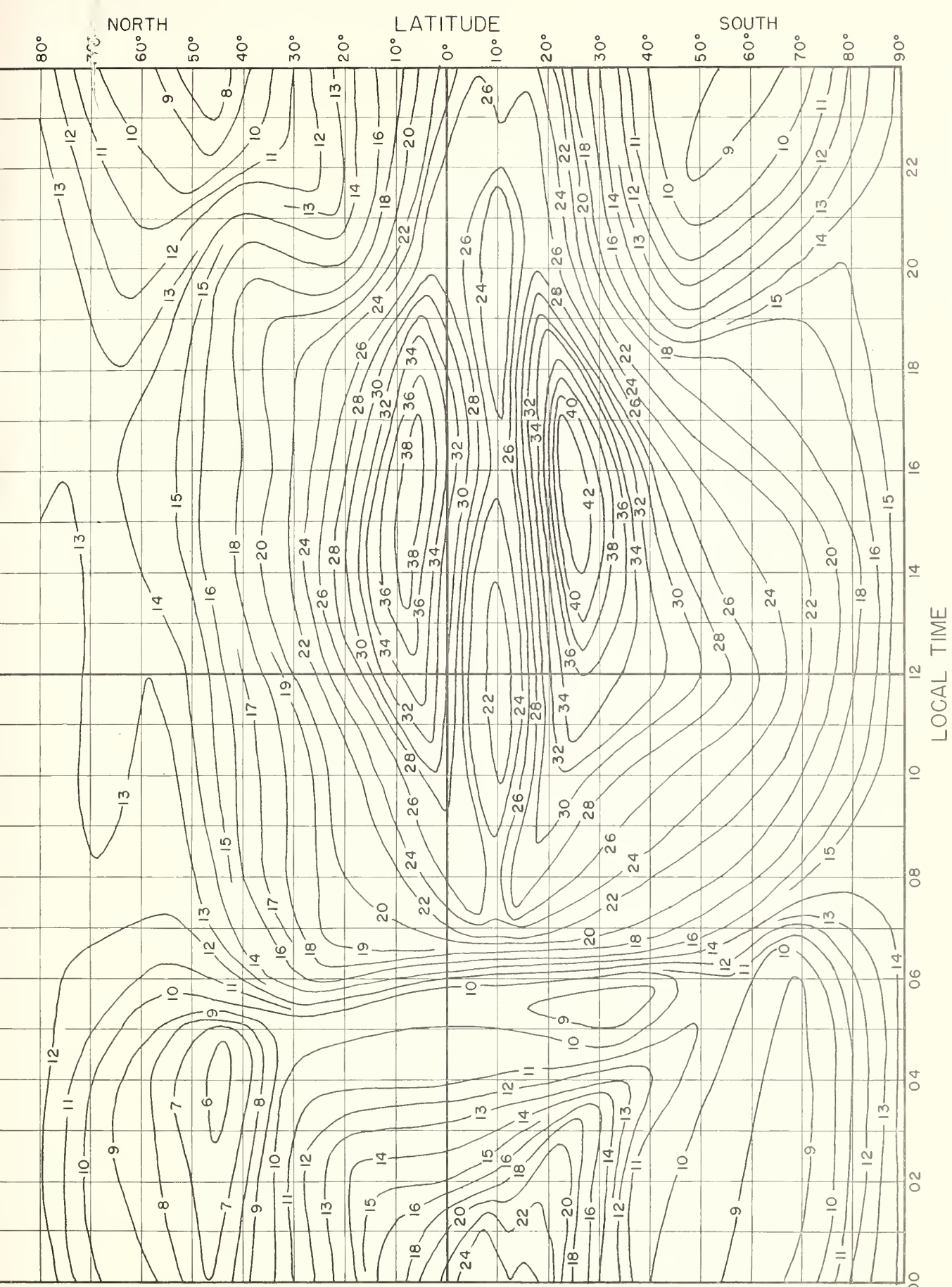
FIG. 2. MEDIAN F2-4000-MUF, IN Mc, W ZONE, PREDICTED FOR APRIL 1955
