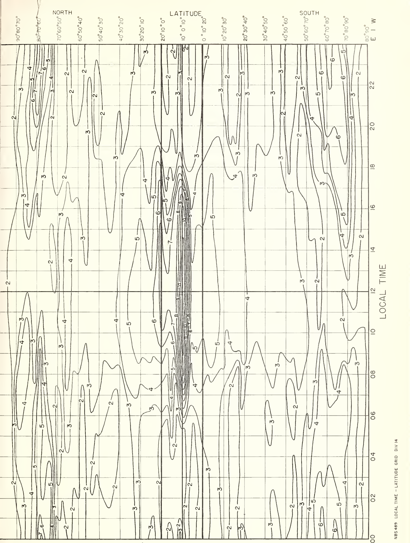
FIG. 8 MEDIAN f_{Es} , IN Mc, PREDICTED FOR APRIL 1955
