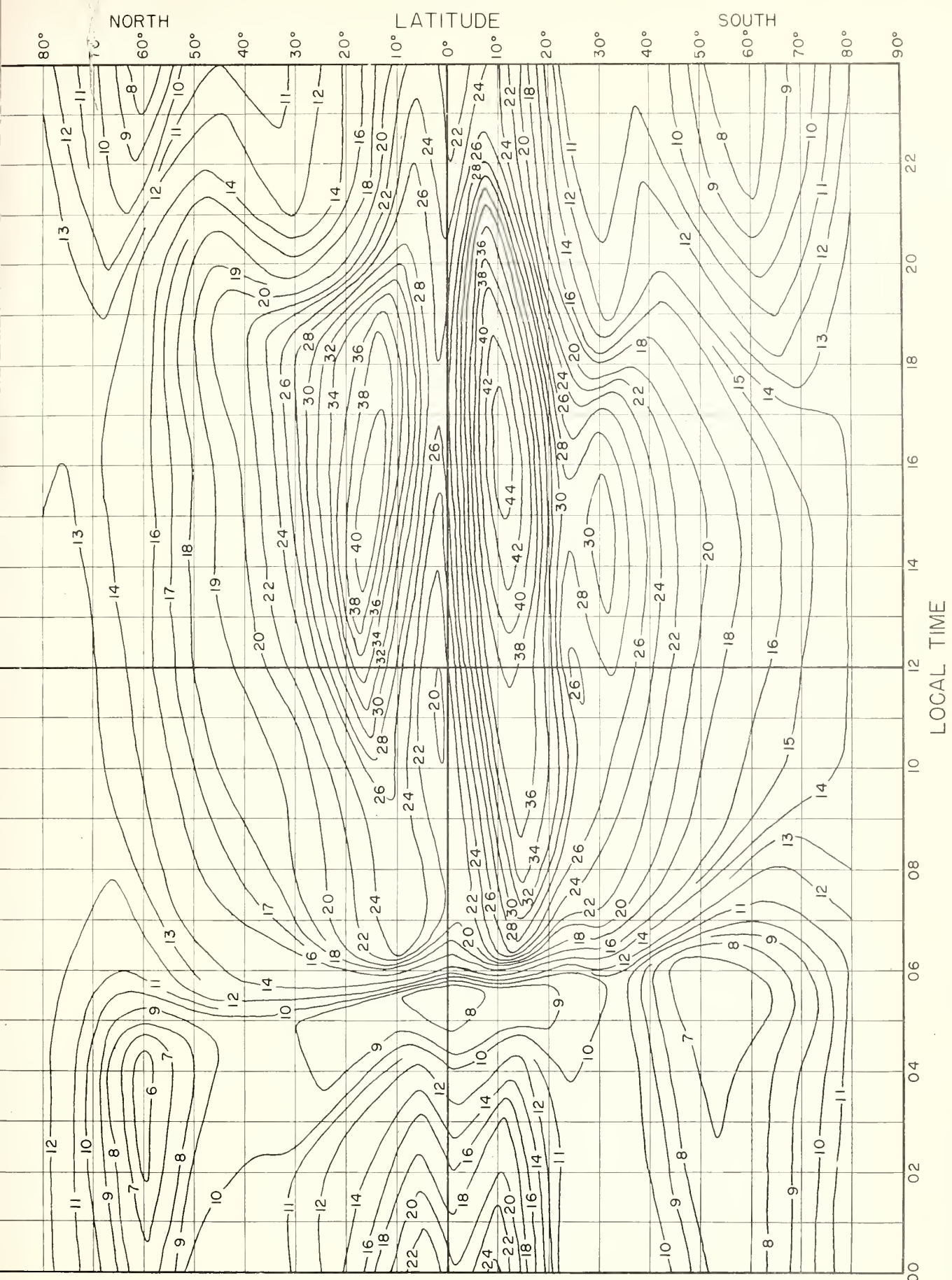
FIG 4 MEDIAN F2-4000-MUF, IN Mc, I ZONE, PREDICTED FOR APRIL 1955
