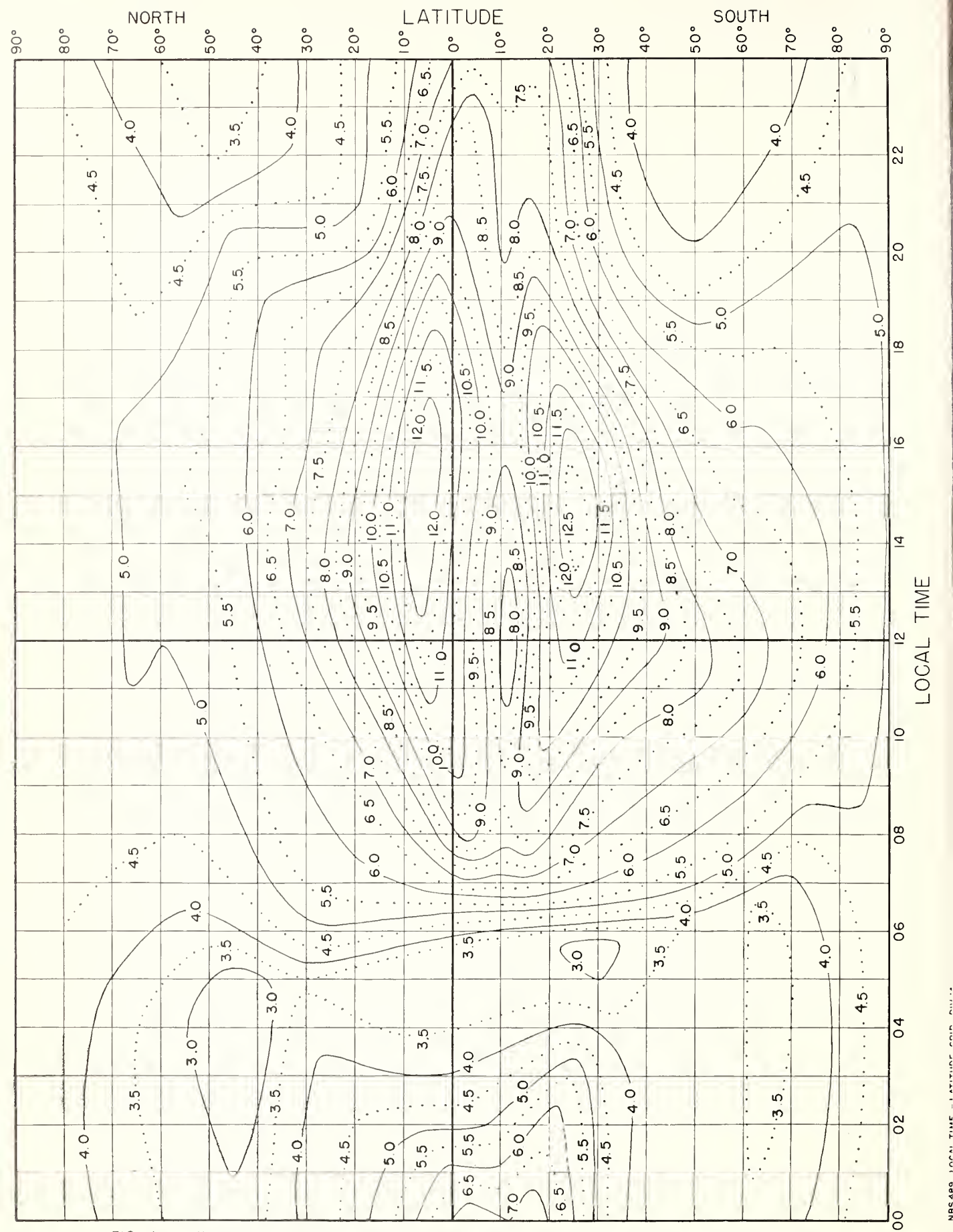
FIG. 1 MEDIAN F2-ZERO-MUF, IN Mc, W ZONE, PREDICTED FOR APRIL 1955
