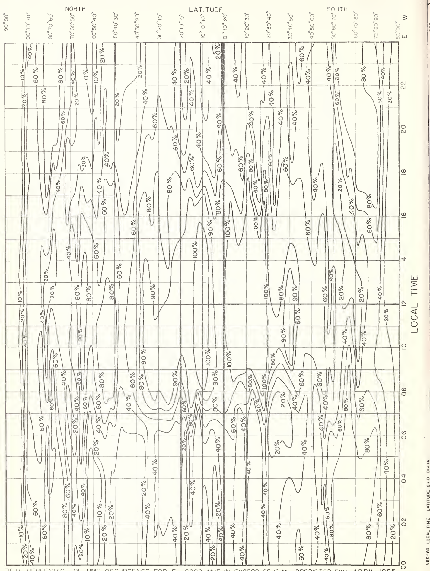
FIG. 9. PERCENTAGE OF TIME OCCURRENCE FOR E_s -2000-MUF IN EXCESS OF 15 Mc, PREDICTED FOR APRIL 1955
