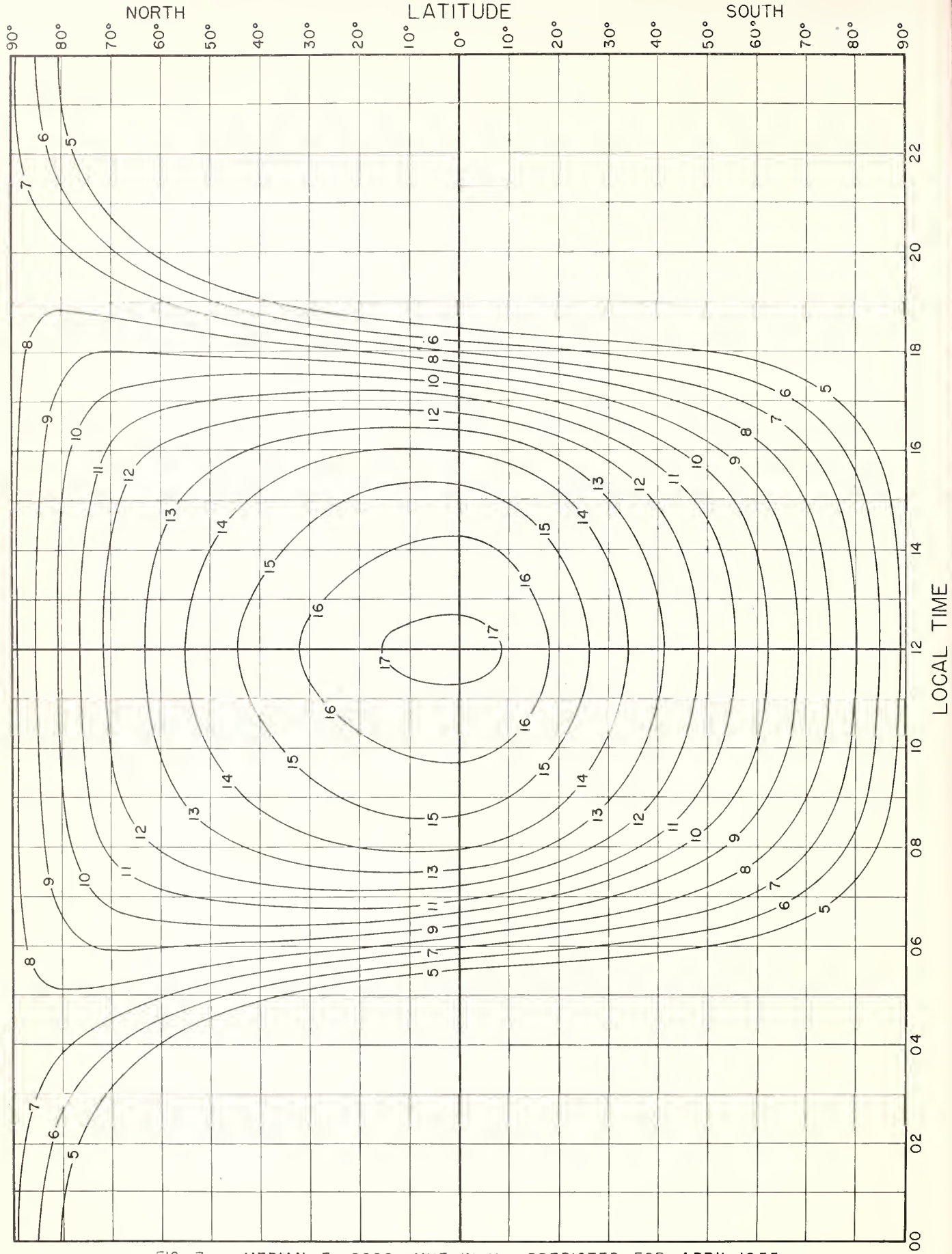
FIG. 7 MEDIAN E-2000-MUF, IN Mc, PREDICTED FOR APRIL 1955
