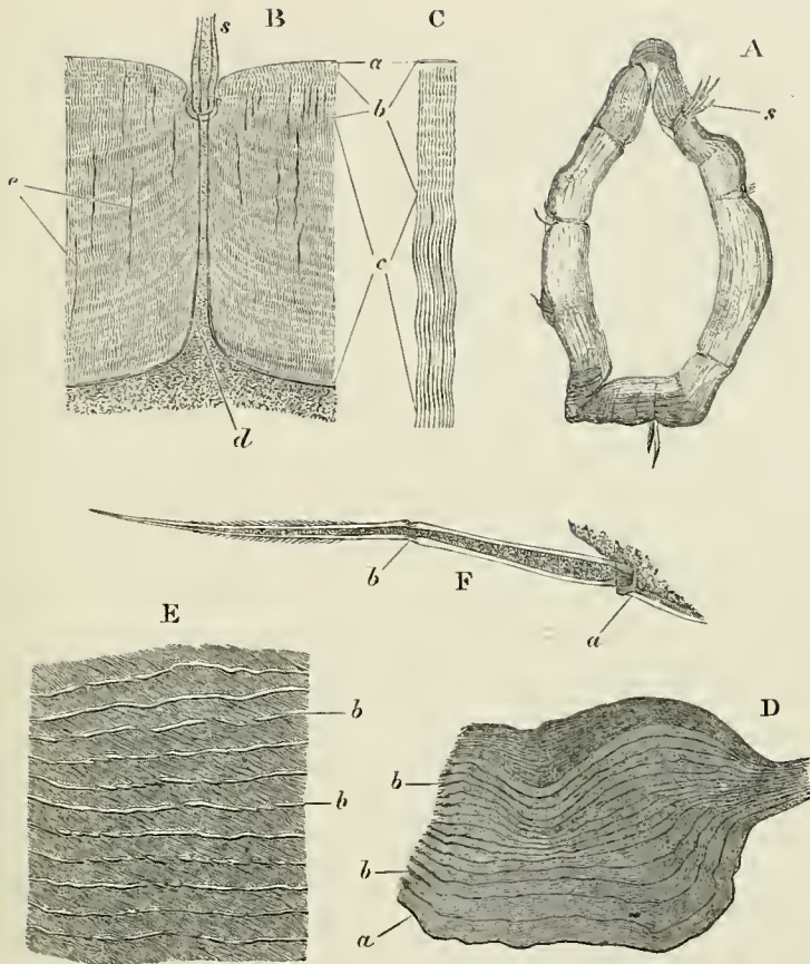
FIG. 56.— Astacus fluviatilis .—The structure of the cuticle. A , transverse section of a joint of the forceps ( \times 4 ); s , setæ; B , a portion of the same ( \times 30 ); C , a portion of B more highly magnified. a , epiostracum; b , ectostracum; c , endostracum; d , canal of seta; c , canals filled with air; s , seta. D , section of an intersternal membrane of the abdomen, the portion to the right in the natural condition, the remainder pulled apart with needles ( \times 20 ); E , small portion of the same, highly magnified; a , intermediate substance; b , laminae. F , a seta, highly magnified; a and b , joints.
