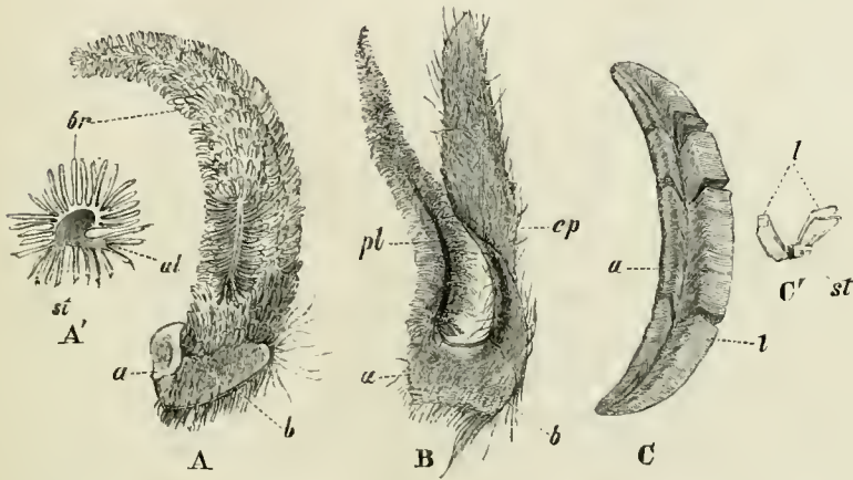
FIG. 68. Podobranchiæ of A, Parastacus ; B, Nephrops ; C, Palaemon . A', C', transverse sections of A and C respectively. a , point of attachment; al , wing-like expansion of the stem; b , base; br , branchial filaments; ep , epipodite; l , branchial lamina; pl , plume; st , stem.
