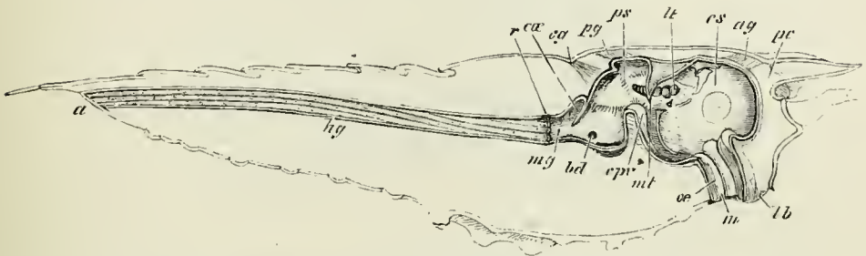
FIG. 6.— Astacus fluviatilis .—A longitudinal vertical section of the alimentary canal, with the outline of the body (nat. size) :— a , vent; ag , anterior gastric muscle; bd , entrance of left bile duct; cg , cervical groove; ca , caecum; cpv , cardio-pyloric valve; cs , cardiac portion of stomach; the circular area immediately below the end of the line from cs marks the position of the gastrolith of the left side; hg , hind-gut; lb , labrum; lt , lateral tooth of stomach; m , mouth; mg , mid-gut; mt , median tooth; w , oesophagus; pc , procephalic process; pg , posterior gastric muscle; ps , pyloric portion of stomach; r , annular ridge, marking the commencement of the hind-gut.
