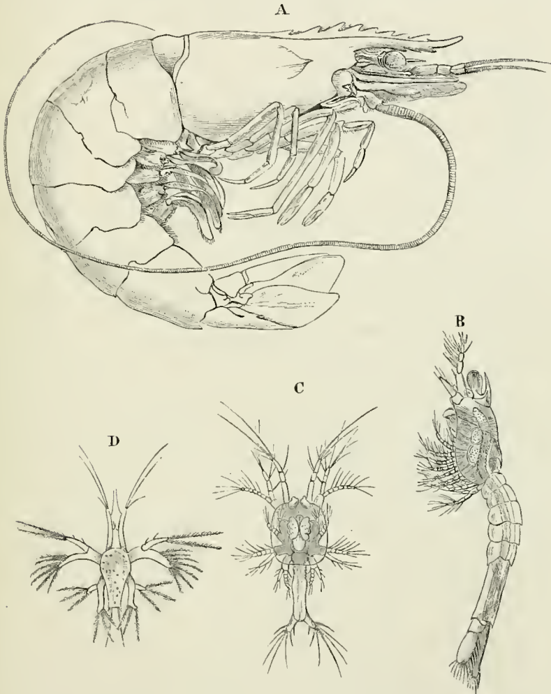
FIG. 73. Penaeus semisulcatus . A, adult (after de Haan. \frac{1}{2} nat. size); B, Zoaea, and C, less advanced Zoaea of a species of Penaeus . D, Nauplius. (B, C, and D, after Fritz Müller.)
