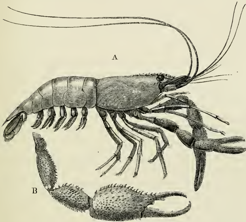
FIG. 71. Palaemon jamaicensis (about \frac{5}{7} nat. size). A, female; B, fifth thoracic appendage of male.
