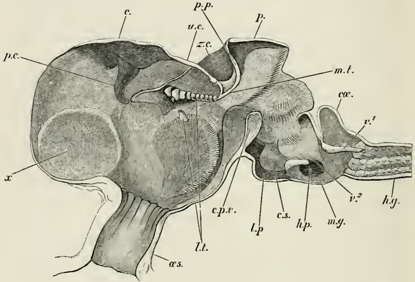
FIG. 10.— Astacus fluvialilis .—Longitudinal section of the stomach ( \times 4 ), c , cardiac ossicle; cæ , cæcum; c.p.v. , cardio-pyloric valve; cs. , cushion-shaped surface; hg. , hind-gut; hp. , aperture of right bile duct; lp. , lateral pouch; lt. , lateral teeth; mg. , mid-gut; mt. , median tooth; æs. , œsophagus; p. , pyloric ossicle; pc. , pterocardiac ossicles; pp. , prepyloric ossicle; uc. , urocardiac process; v¹ , median pyloric valve; v² , lateral pyloric valve; x , position of gastrolith; zc. , zyocardiac ossicle.
