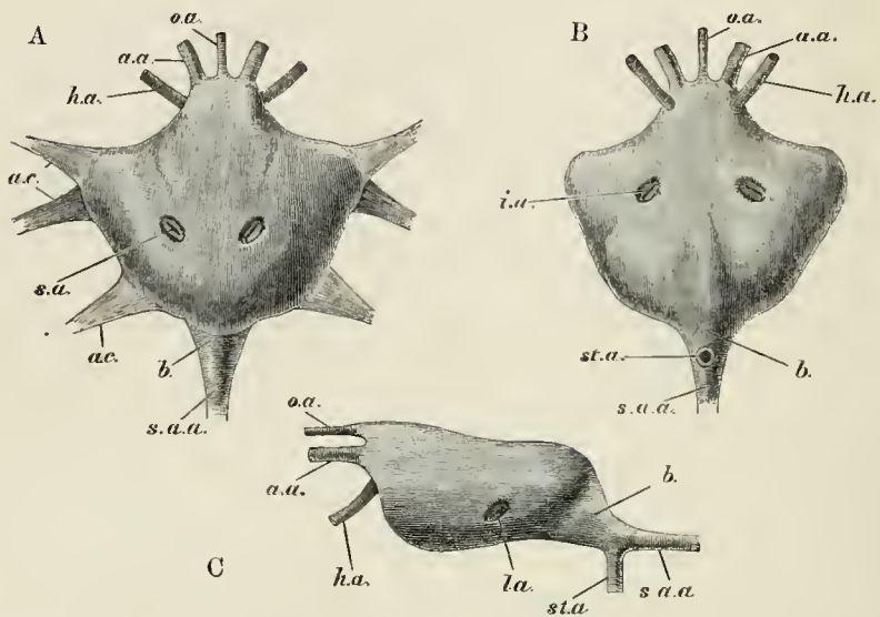
FIG. 16.— Astacus fluviatilis .—The heart ( \times 4 ). A, from above ; B, from below ; C, from the left side. aa , antennary artery ; ac , alae cordis, or fibrous bands connecting the heart with the walls of the pericardial sinus ; b , bulbous dilatation at the origin of the sternal artery ; ha , hepatic artery ; la , lateral valvular apertures ; oa , ophthalmic artery ; sa , superior valvular apertures ; saa , superior abdominal artery ; sta , sternal artery, in B cut off close to its origin.
