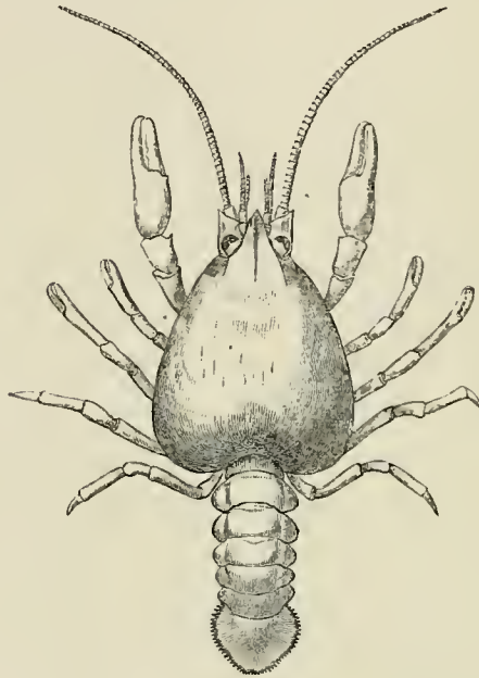
FIG. 60.— Astacus fluviatilis .—Newly-hatched young ( \times 6 ).
