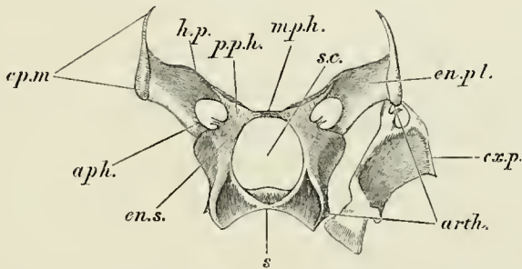
FIG. 42.— Astacus fluviatilis .—A segment of the endophragmal system ( \times 3 ). aph. arthrophragm; arth. arthrodial or articular cavity; exp. coxopodite of the ambulatory leg; enpl. endopleurite; ens. endosternite; epm. epimeron; hp. horizontal process of endopleurite; mph. mesophragm; pph. paraphragm; s. sternum of somite; sc. sternal canal.
