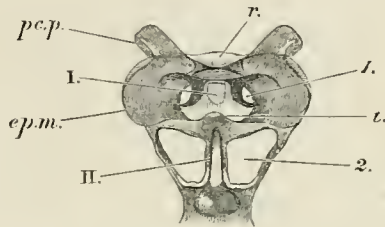
FIG. 40.— Astacus fluviatilis .—The ophthalmic and antennular somites ( \times 3 ). I. , ophthalmic, and II. , antennular sternum; 1. , articular surface for eyestalk; 2. , for antennule; ep.m. , epimeral plate; p.c.p. , procephalic process; r. , base of rostrum; t. , tubercle.
