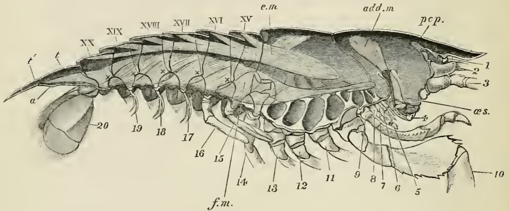
FIG. 22.— Astacus fluvialtilis .—A longitudinal section of the body to show the principal muscles and their relations to the exoskeleton (nat. size). a , the vent; add.m. , adductor muscle of mandible; e.m. , extensor, and f.m. , flexor muscle of abdomen; αs. , oesophagus; pcp. , procephalic process; t, t' , the two segments of the telson; XV—XX, the abdominal somites; 1—20, the appendages; x, x, hinges between the successive abdominal somites.
