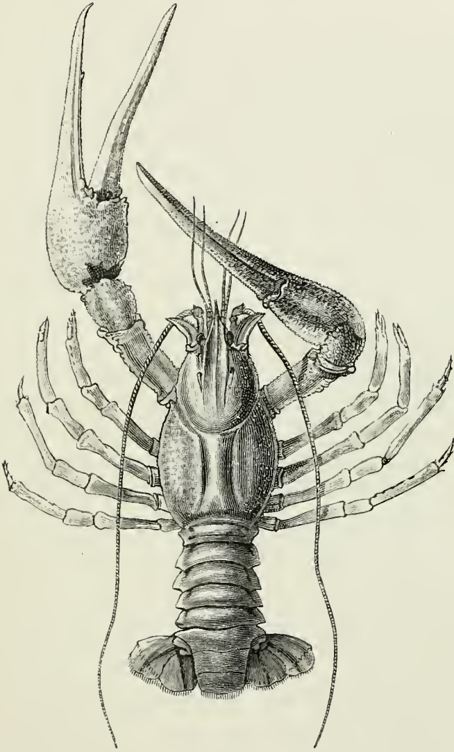
FIG. 75.— Astacus leptodactylus (after Rathke, \frac{1}{3} nat. size).
