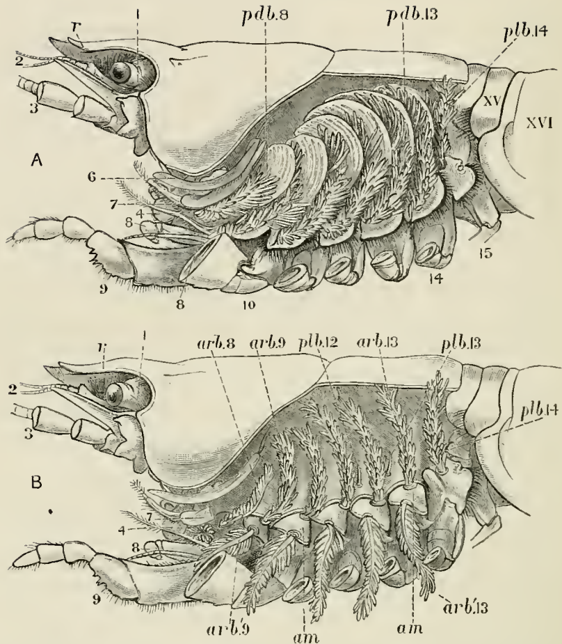
FIG. 4.— Astacus fluviatilis .—In A, the gills, exposed by the removal of the branchiostegite, are seen in their natural position; in B, the podobranchiae (see p. 75) are removed, and the anterior set of arthrobranchiae turned downwards ( \times 2 ): 1, eye-stalk; 2, antennule; 3, antenna; 4, mandible; 6, scaphognathite; 7, first maxillipede, in B the epipodite, to which the line points, is partly removed; 8, second maxillipede; 9, third maxillipede; 10, forceps; 14, fourth ambulatory leg; 15, first abdominal appendage; xv, first, and xvi, second abdominal somite; arb. 8, arb. 9, arb. 13, the posterior arthrobranchiae of the second and third maxillipedes and of the third ambulatory leg; arb. 9, arb. 13, the anterior arthrobranchiae of the third maxillipede and of the third ambulatory leg; pdb. 8, podobranchiae of the second maxillipede; pdb. 13, that of the third ambulatory leg; plb. 12, plb. 13, the two rudimentary pleurobranchiae; plb. 14, the functional pleurobranchia; r, rostrum.
