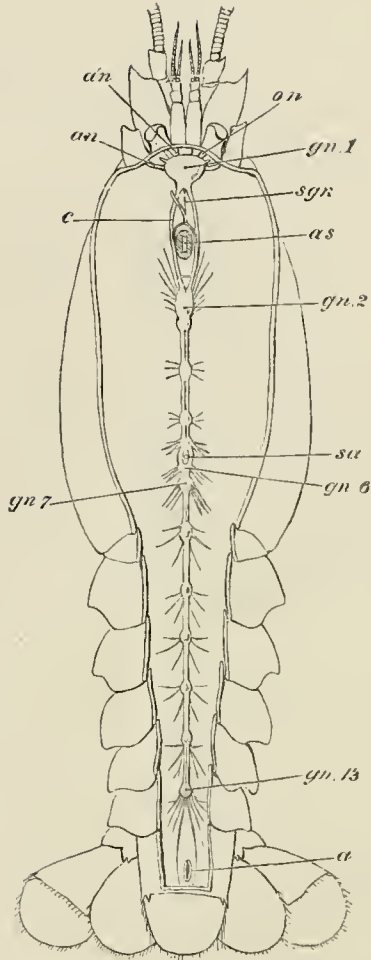
FIG. 25.— Astacus fluviatilis .—The central nervous system seen from above (nat. size). a , vent; an , antennary nerve; a'n , antennular nerve; c , circumoesophageal commissures; gn. 1 , supræoesophageal ganglion; gn. 2 , infraoesophageal ganglion; gn. 6 , fifth thoracic ganglion; gn. 7 , last thoracic ganglion; gn. 13 , last abdominal ganglion; as , œsophagus in cross section; an , optic nerve; sa , sternal artery in cross section; sgn , stomatogastric nerve.
