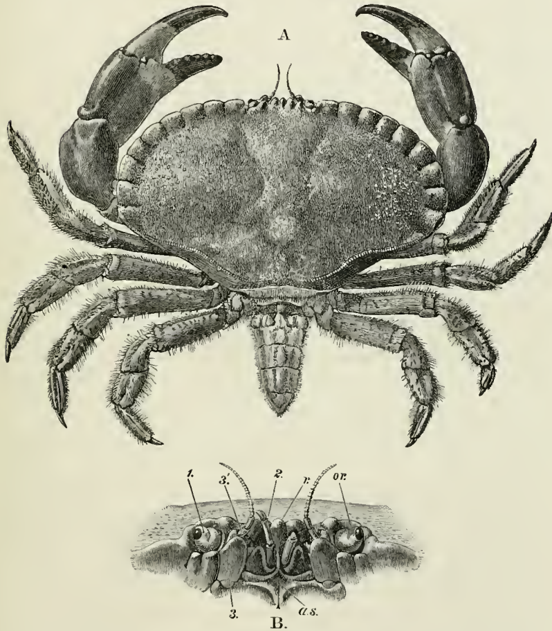
FIG. 72. Cancer pagurus , male ( \frac{1}{3} nat. size). A, dorsal view, with the abdomen extended; B, front view of "face." as. , antennary sternum; or. , orbit; r. , rostrum; 1. eyestalk; 2. antennule; 3. base of antenna; 3', free portion of antenna.
