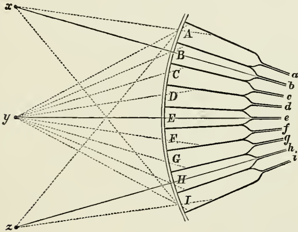
FIG. 29.—Diagram showing the course of rays of light from three points x, y, z , through the nine visual rods (supposed to be empty tubes) A-I of a compound eye; a-i , the nerve fibres connected with the visual rods.
