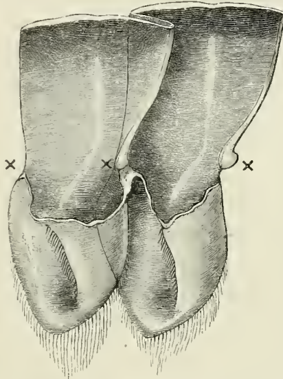
FIG. 21.— Astacus fluvialtilis .—Two of the abdominal somites, in vertical section, seen from the inner side, to show x, x, the hinges by which they are articulated with one another ( \times 3 ). The anterior of the two somites is that to the right of the figure.
