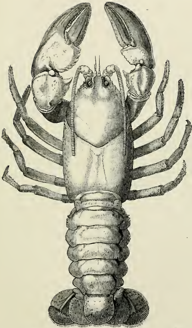
FIG. 65.— Astacoides madagascarensis ( \frac{2}{3} nat. size). From Madagascar.
