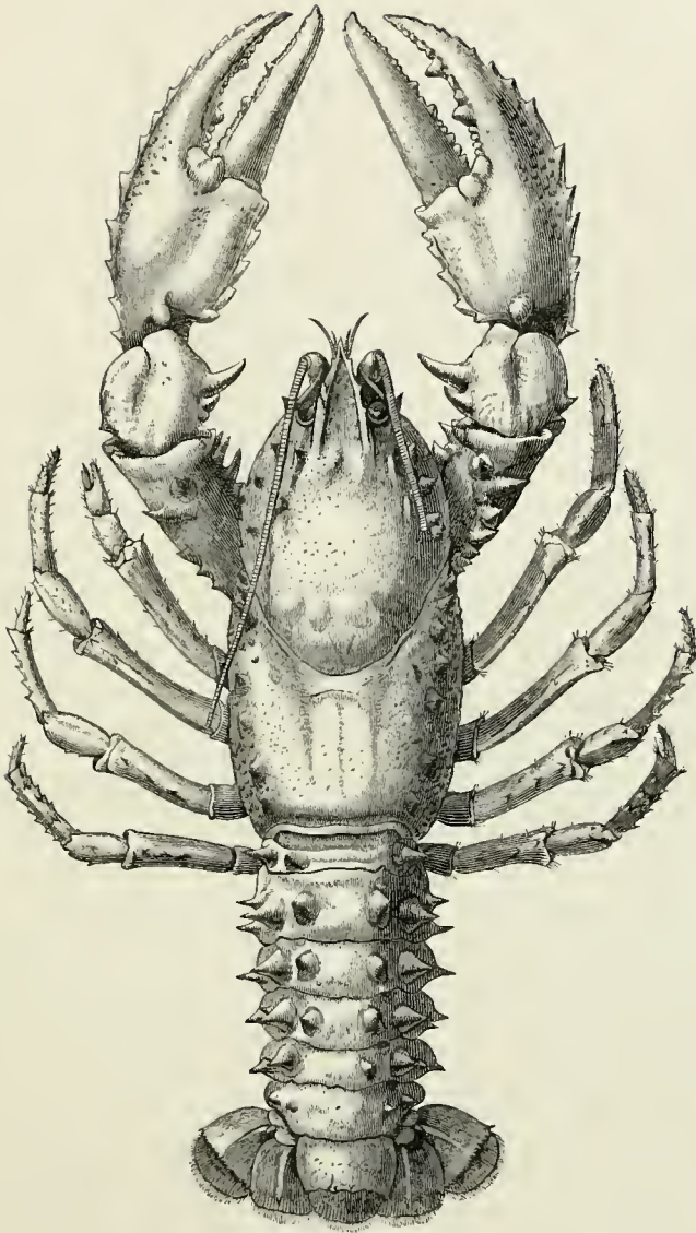
FIG. 76.—Australian Crayfish ( \frac{1}{3} nat. size).*
