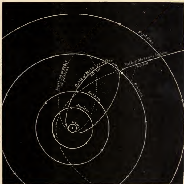
Fig. 78.—The History of the Leonids.
