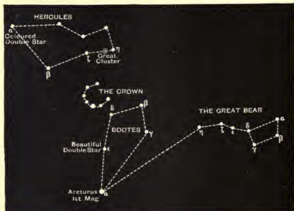
Fig. 83.—Boötes and the Crown.
