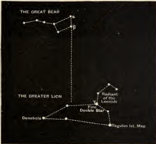
Fig. 87.—The Great Bear and the Lion.
