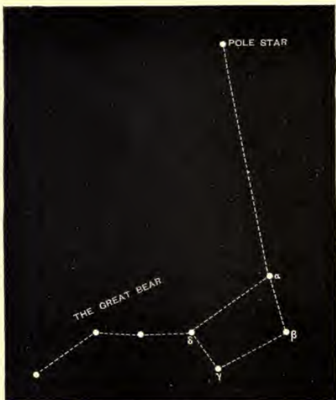
Fig. 80.—The Great Bear and Pole Star.
