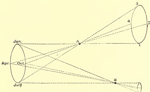
Fig. 93.—The Parallaxic Ellipse.
