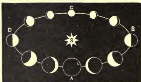
Fig. 41.—The Movement of Mercury, showing the Variations in Phase and in apparent size.
