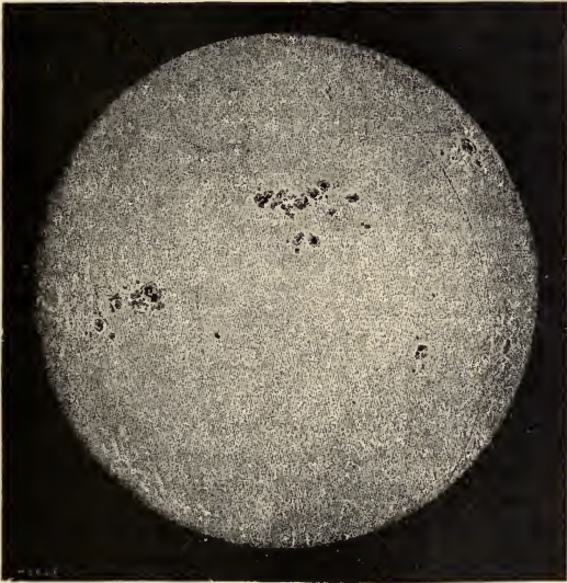
Fig. 11.—The Sun, photographed on September 22, 1870.
