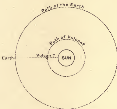
Fig. 40.—The Transit of the Planet of Romance.
