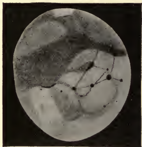
Fig. 51.—Drawing of Mars (July 30th, 1894).
