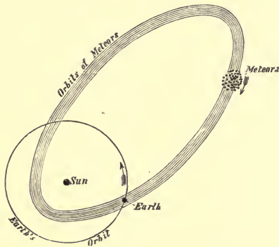
Fig. 76.—The Orbit of a Shoal of Meteors.
