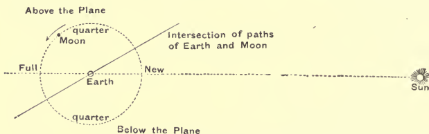
Fig. 24.—The Moon's Path around the Sun.
