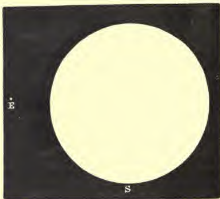
Fig. 10.—Comparative Sizes of the Earth and the Sun.
