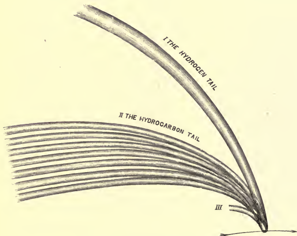
Fig. 72.—Bredichin's Theory of Comets' Tails.
