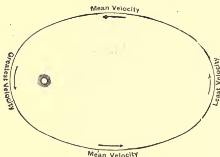
Fig. 38.—Varying Velocity of Elliptic Motion.
