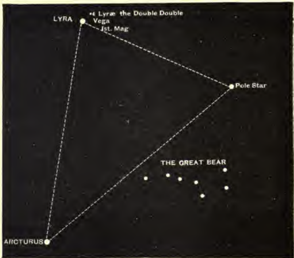
Fig. 90.—The Constellation of Lyra.
