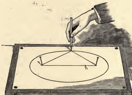
Fig. 37.—Drawing an Ellipse.
