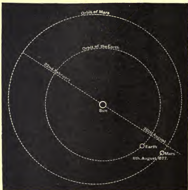
Fig. 48.—The Orbits of the Earth and of Mars, showing the Favourable Opposition of 1877.
