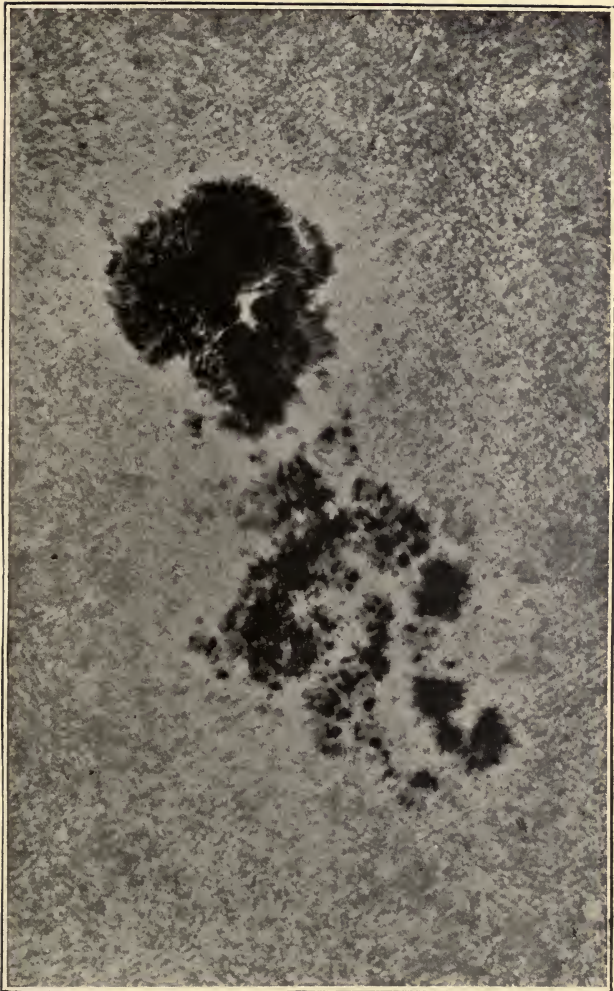
Fig. 12.—Photograph of the Solar Surface. ( By Janssen. )
