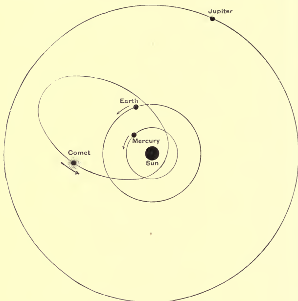
Fig. 70.—The Orbit of Encke's Comet.
