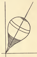
Fig. 101.—Illustration of the Motion of Precession.
