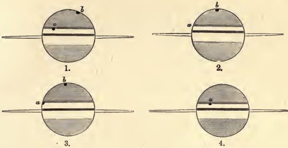
Fig. 68.—Transit of Titan and its Shadow, by F. Terby Louvain, 12th April, 1892.
