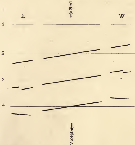
Fig. 67.—Prof. Keeler's Method of Measuring the Rotation of Saturn's Ring.
