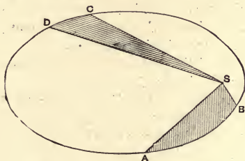
Fig. 39.—Equal Areas in Equal Times.
