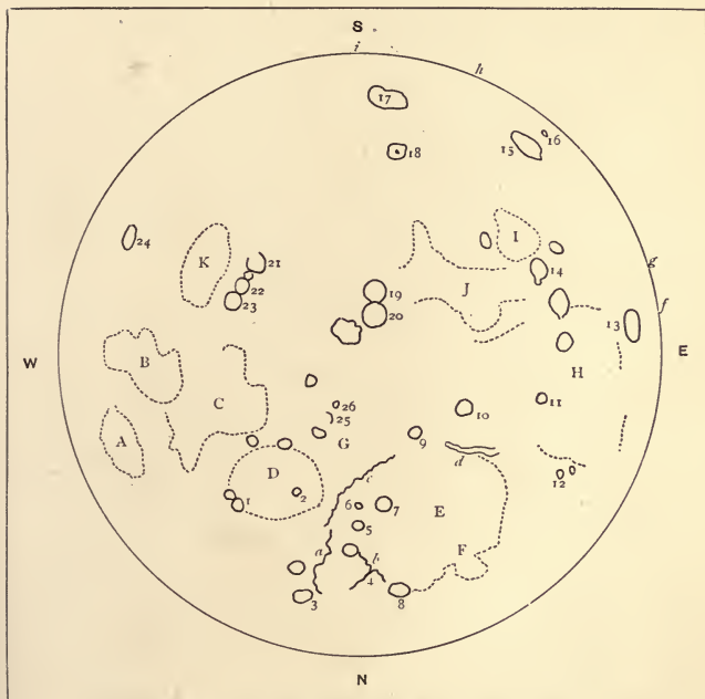
Fig. 27.—Key to Chart of the Moon (Plate VI.).
