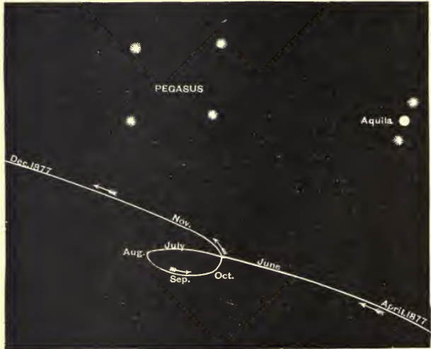
Fig. 49.—The Apparent Movements of Mars in 1877.
