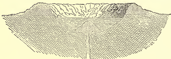
Fig. 20.—Formation of the Level Floor by Lava.
