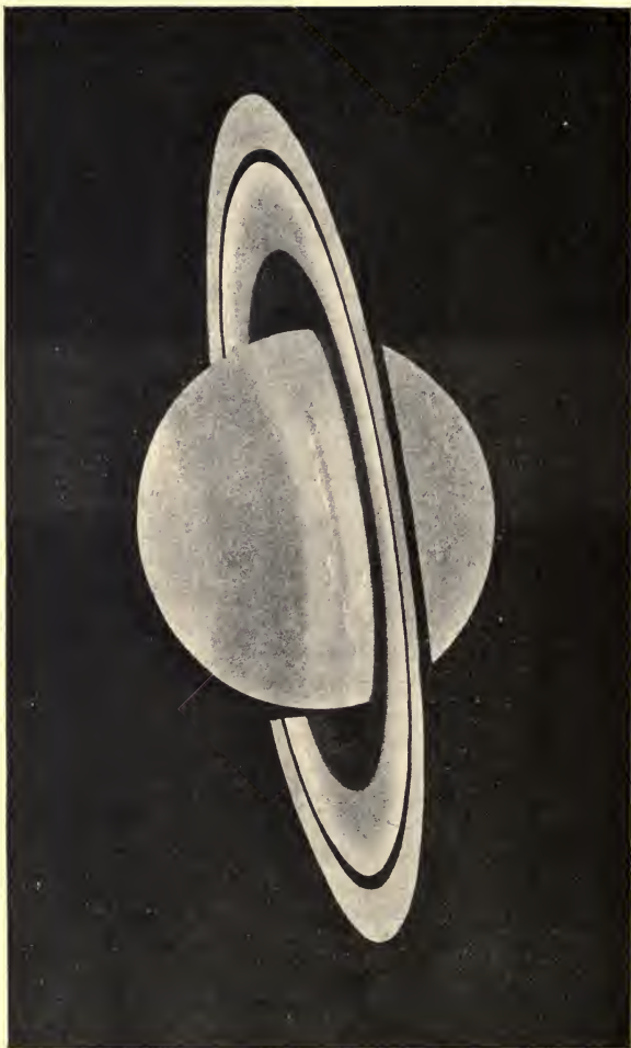
Fig. 64.—Saturn, (July 2nd, 1894, 36-in. equatorial.) (Prof. E. E. Barnard.)
