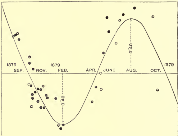
Fig. 95.—Parallax in Declination of 61 Cygni.
