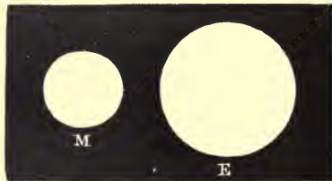
Fig 50.—Relative Sizes of Mars and the Earth.
