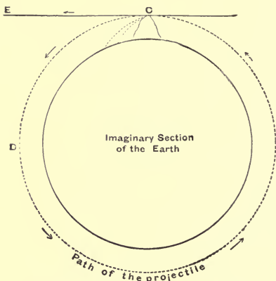
Fig. 36.—Illustration of the Moon's Motion.
