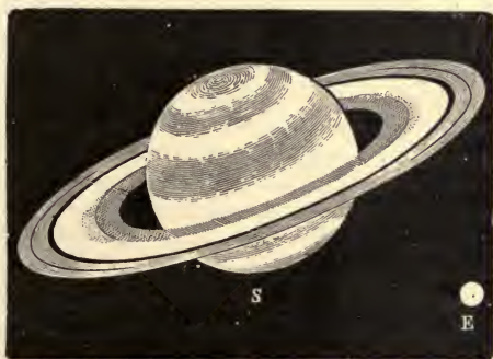
Fig. 65.—Relative Sizes of Saturn and the Earth.
