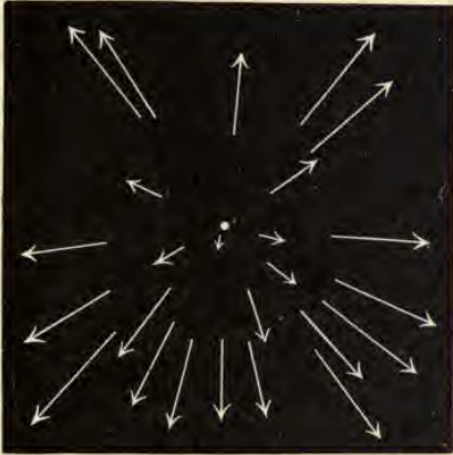
Fig. 77.—The Radiant Point of Shooting Stars.
