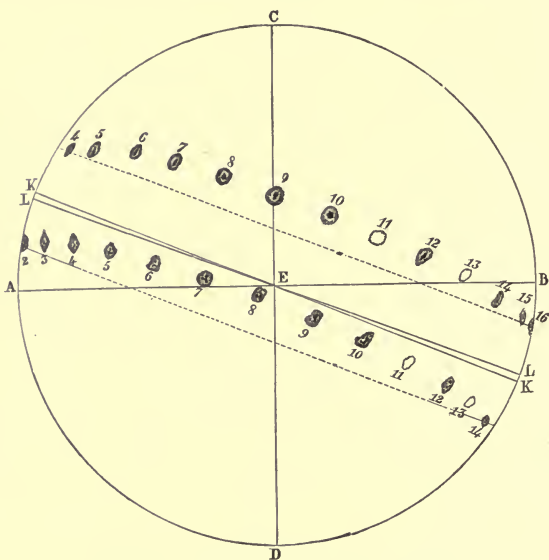
Fig. 14.—Scheiner's Observations on Sun-spots.
