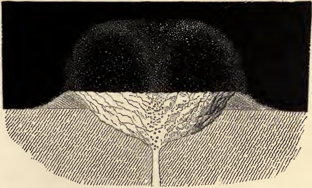
Fig. 28.—Volcano in Activity.
