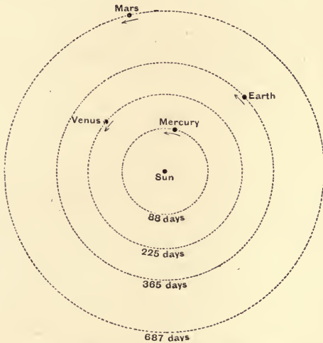
Fig. 31.—The Orbits of the Four Interior Planets.
