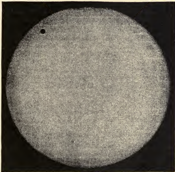
Fig. 45.—Venus on the Sun at the Transit of 1874.
