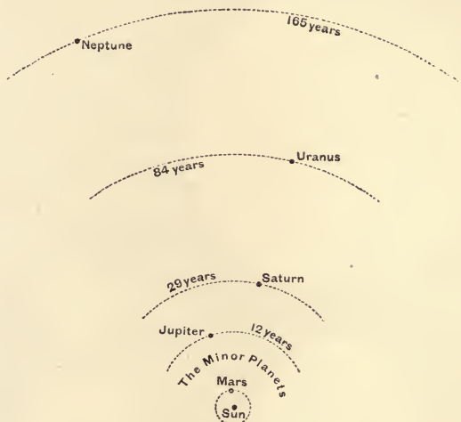
Fig. 33.—The Orbits of the Four Giant Planets.
