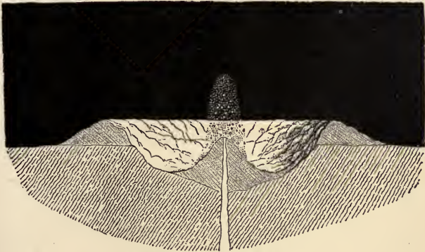
Fig. 29.—Subsequent Feeble Activity.
