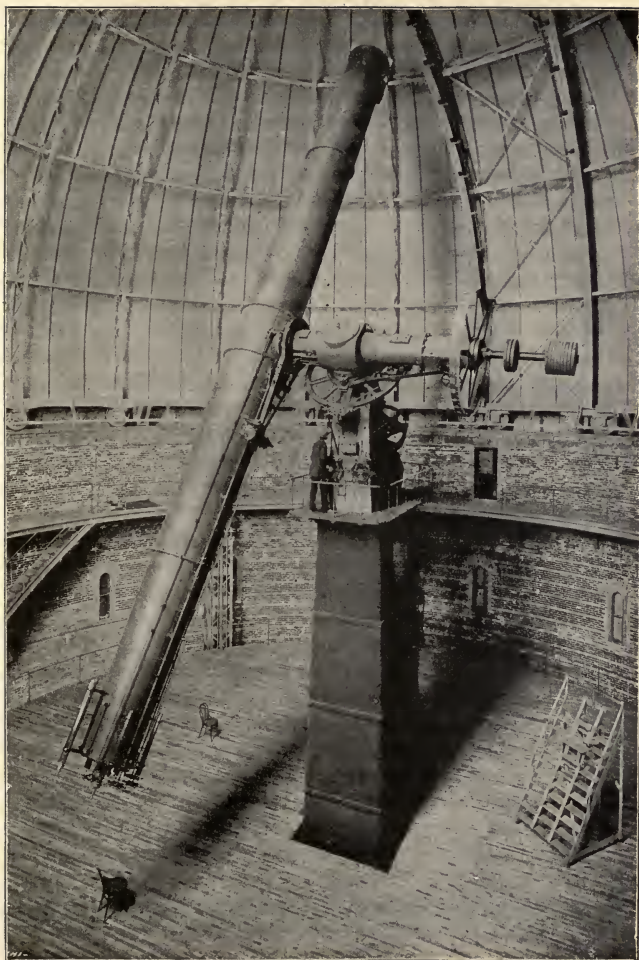
Fig. 4.—The Telescope at Yerkes Observatory, Chicago.
