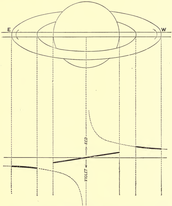
Fig. 66.—Prof. Keeler's Method of Measuring the Rotation of Saturn's Ring.
