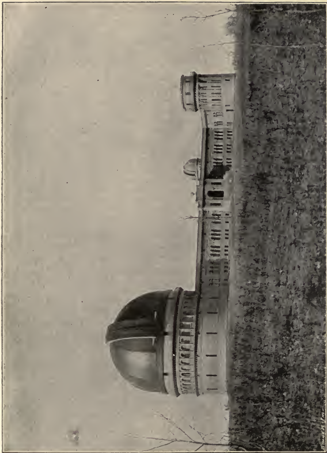
Fig. 6.—South Front of the Yerkes Observatory, Chicago. (From the Astrophysical Journal , Vol. vi., No. 1.)
