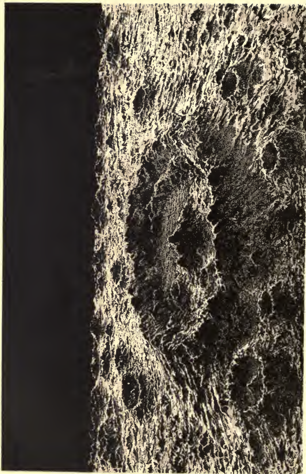
A NORMAL LUNAR CRATER.
