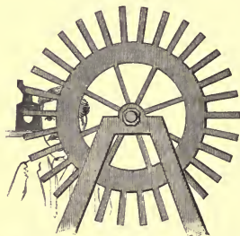
Fig. 63.—Mode of Measuring the Velocity of Light.
