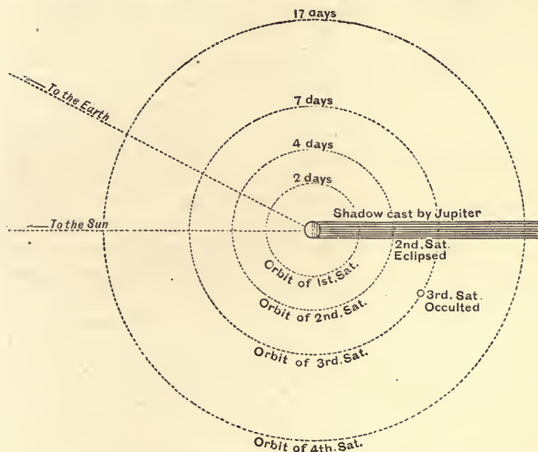
Fig. 62.—Disappearances of Jupiter's Satellites.
