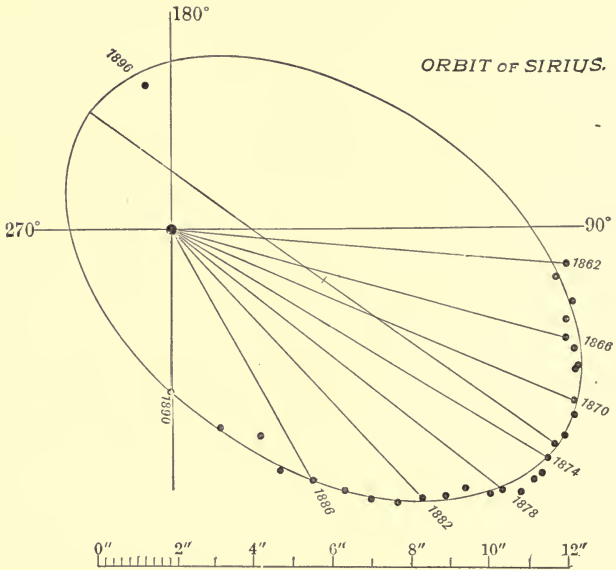
Fig. 92.—The Orbit of Sirius (Professor Burnham).
