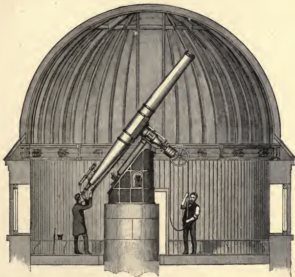
Fig. 3.—Section of the Dome of Dunsink Observatory.
