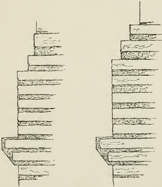
Brick plinths.
