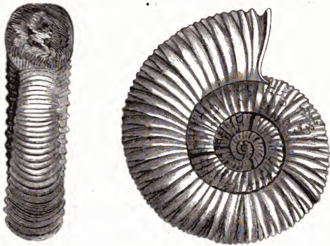
Ammonites bplex.
