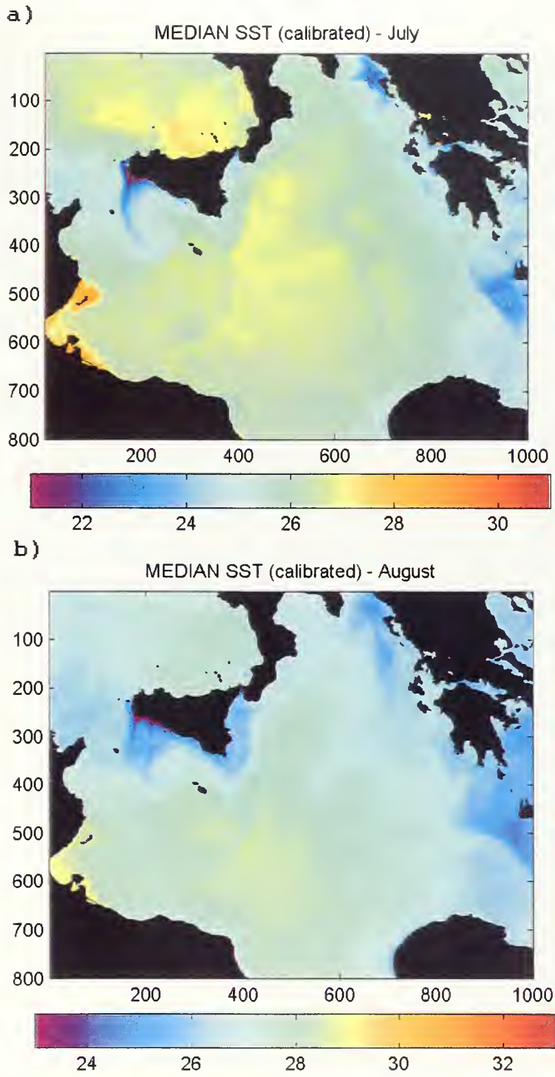
Figure IV-3. Median temperature composites for (a) July and (b) August, 1995.
