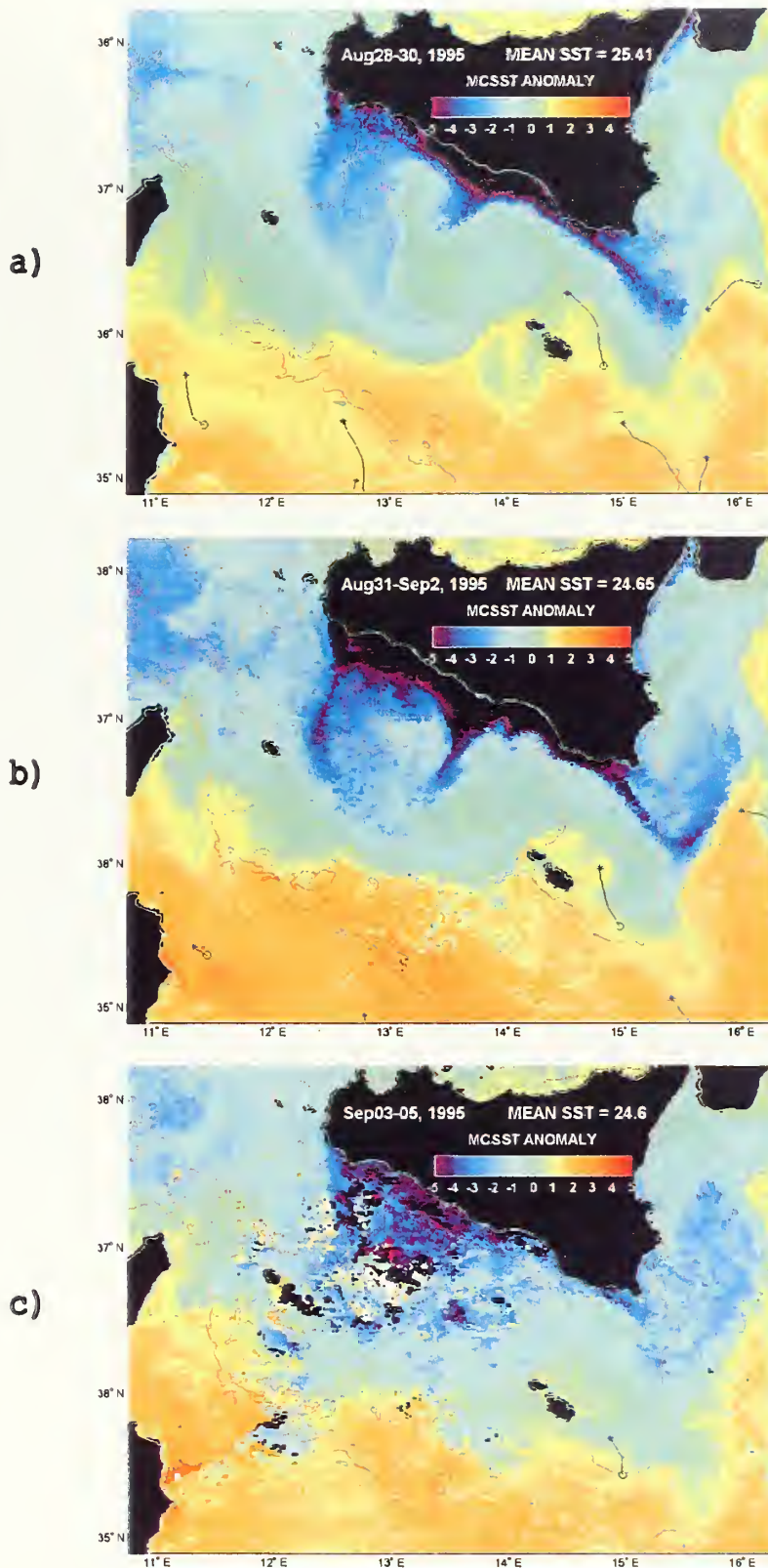
Figure IV-21. Three-day composites of SST anomaly for (a) 28-30 August, (b) 31 August-2 September and (c) 3-5 September, 1995. 5-day long drifter trajectories centered on the 3-day periods are overlaid on the images.
