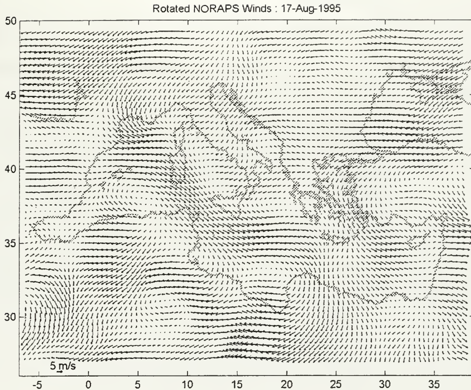
Figure III-4. Orographically steered NORAPS wind vectors for 17 August 1995.
