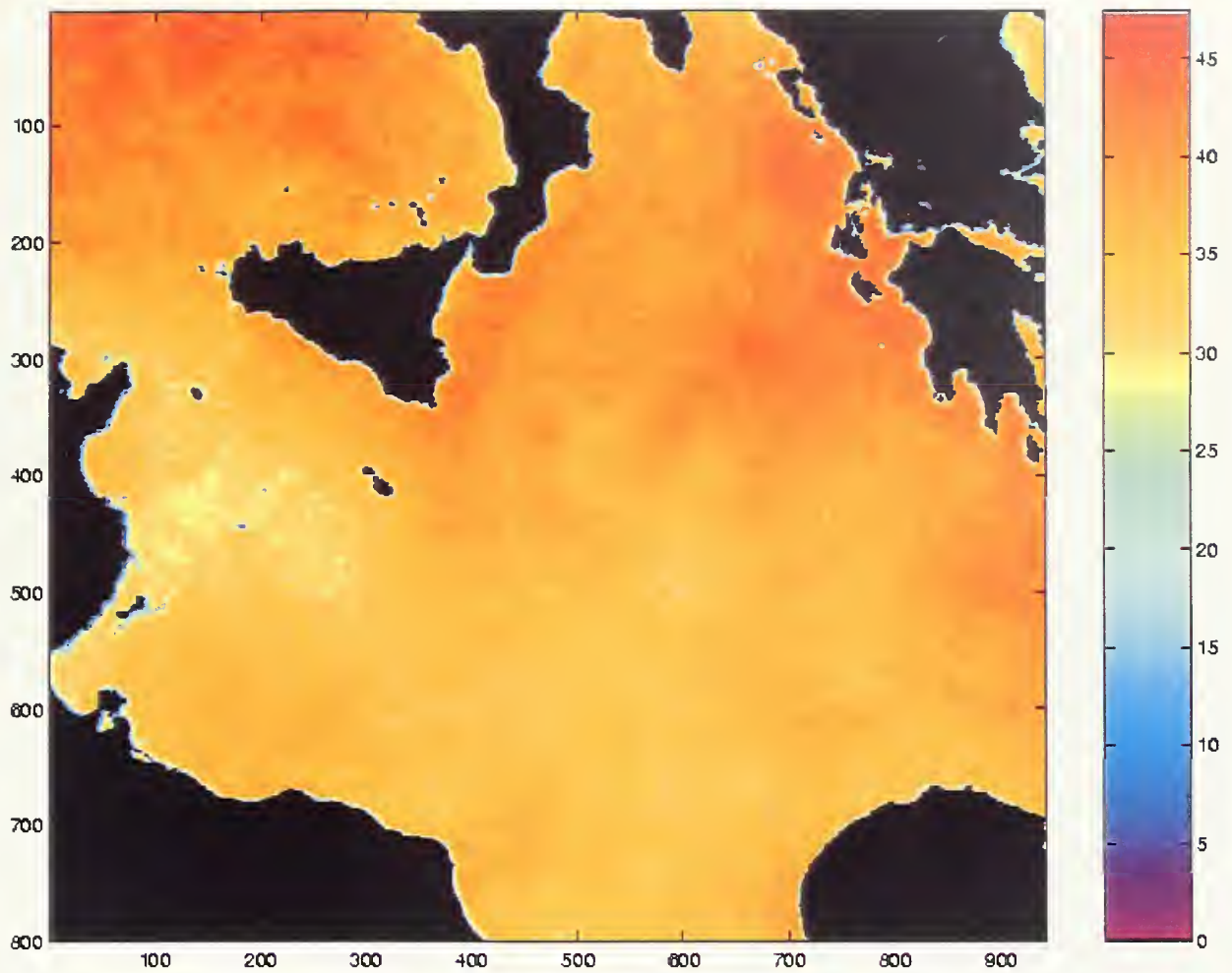
Percentage of clear pixels - 9 May to 22 Oct, 1995
