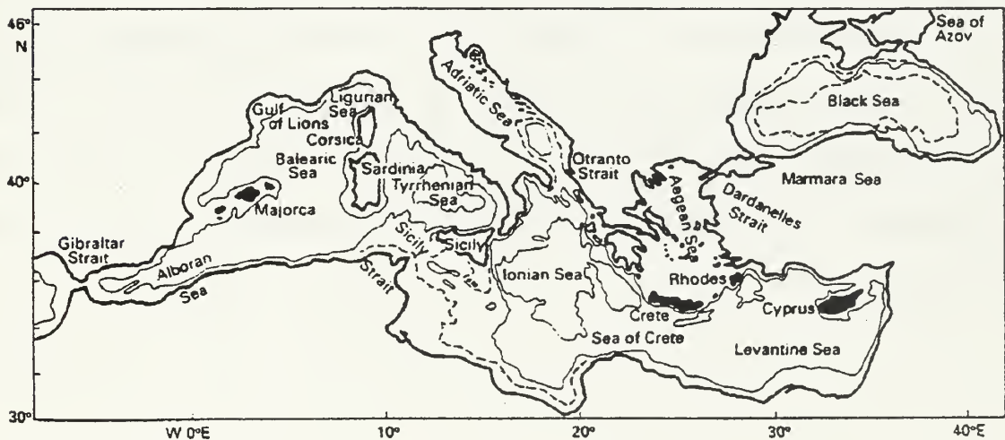
Figure II-1. Mediterranean Sea, showing nonmenclature of the major sub-basins and Straits (from Godfrey and Tomaczak, 1994).
