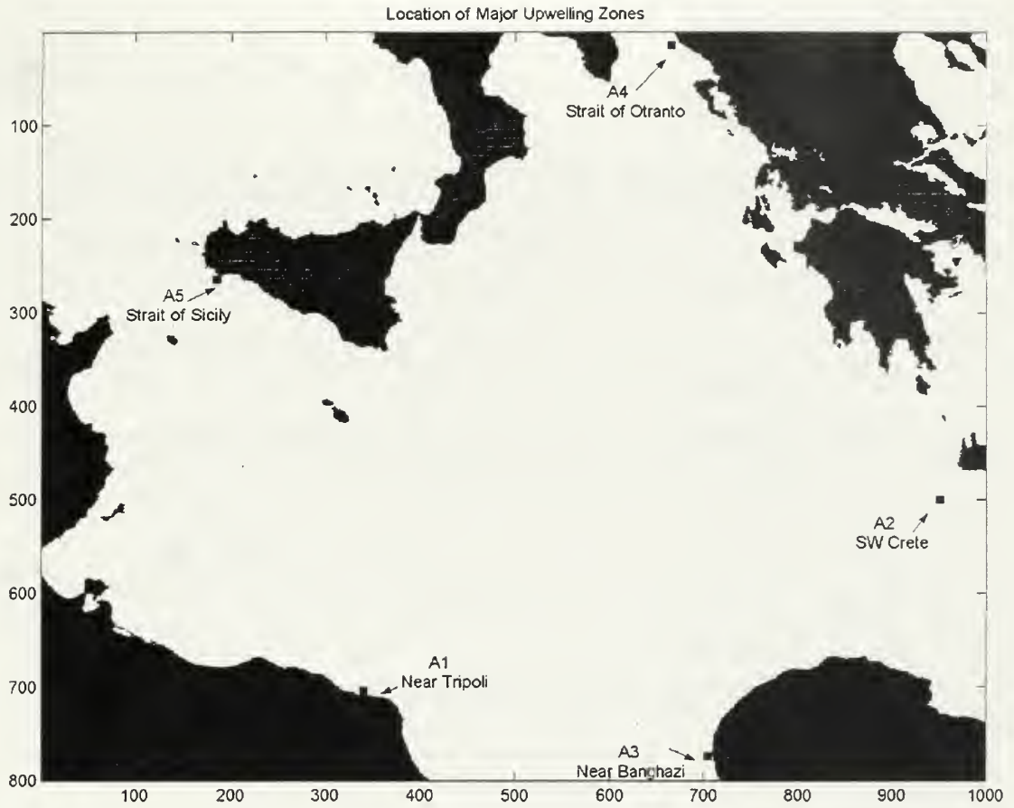
Figure IV-7. Location of major upwelling areas in the Ionian Sea.
