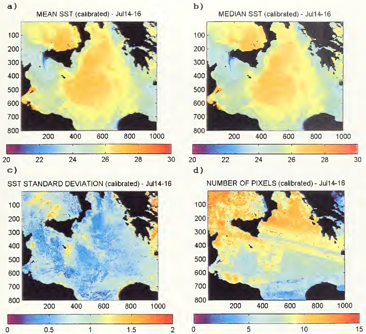
Figure III-19. Plot of composite image of (a) mean SST, (b) median SST, (c) standard deviation SST, and (d) number of pixels for July 14-16, 1995.
