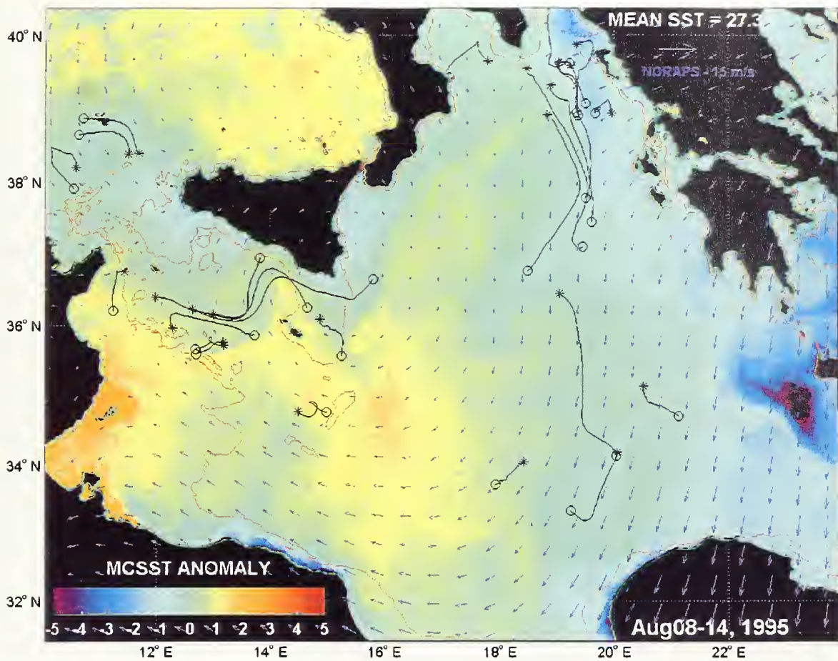
Figure IV-6. Composite map of mean SST anomaly of the median SST for the week of August 8 to 14, 1995. Overlaid is the weekly summary of rotated NORAPS winds showing surface direction and speed. Also shown are 10-day long drifter trajectory segments centered on the week considered.
