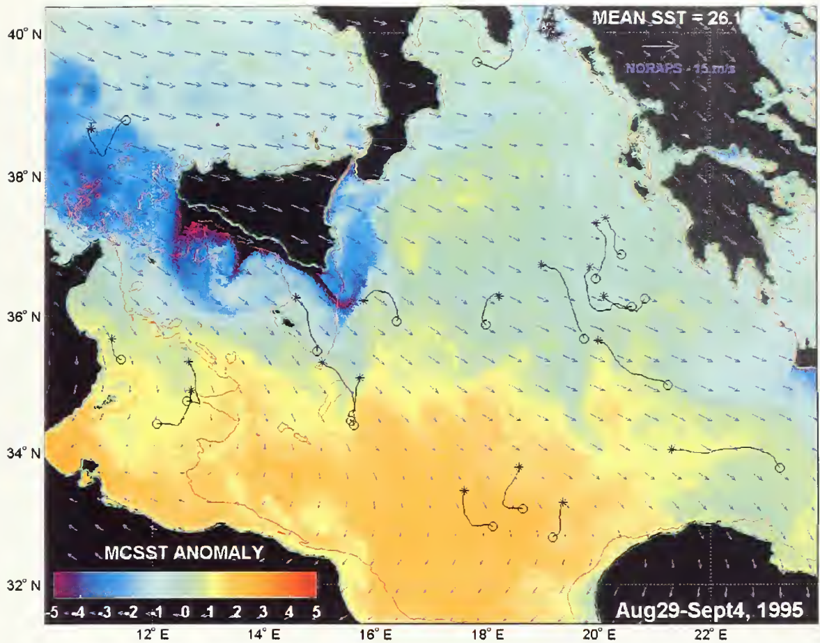
Figure IV-5. Composite map of mean SST anomaly of the median SST for the week of August 29 to September 4, 1995. Overlaid is the weekly summary of rotated NORAPS winds showing surface direction and speed. Also shown are 10-day long drifter trajectory segments centered on the week considered.
