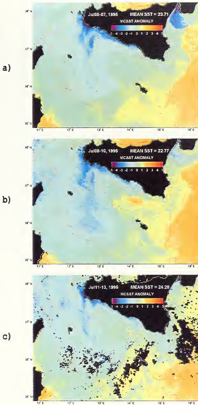
Figure IV-15. Three-day composites of SST anomaly for (a) 5-7 July, (b) 8-10 July and (c) 11-13 July, 1995. 5-day long drifter trajectories centered on the 3-day periods are overlaid on the images.
