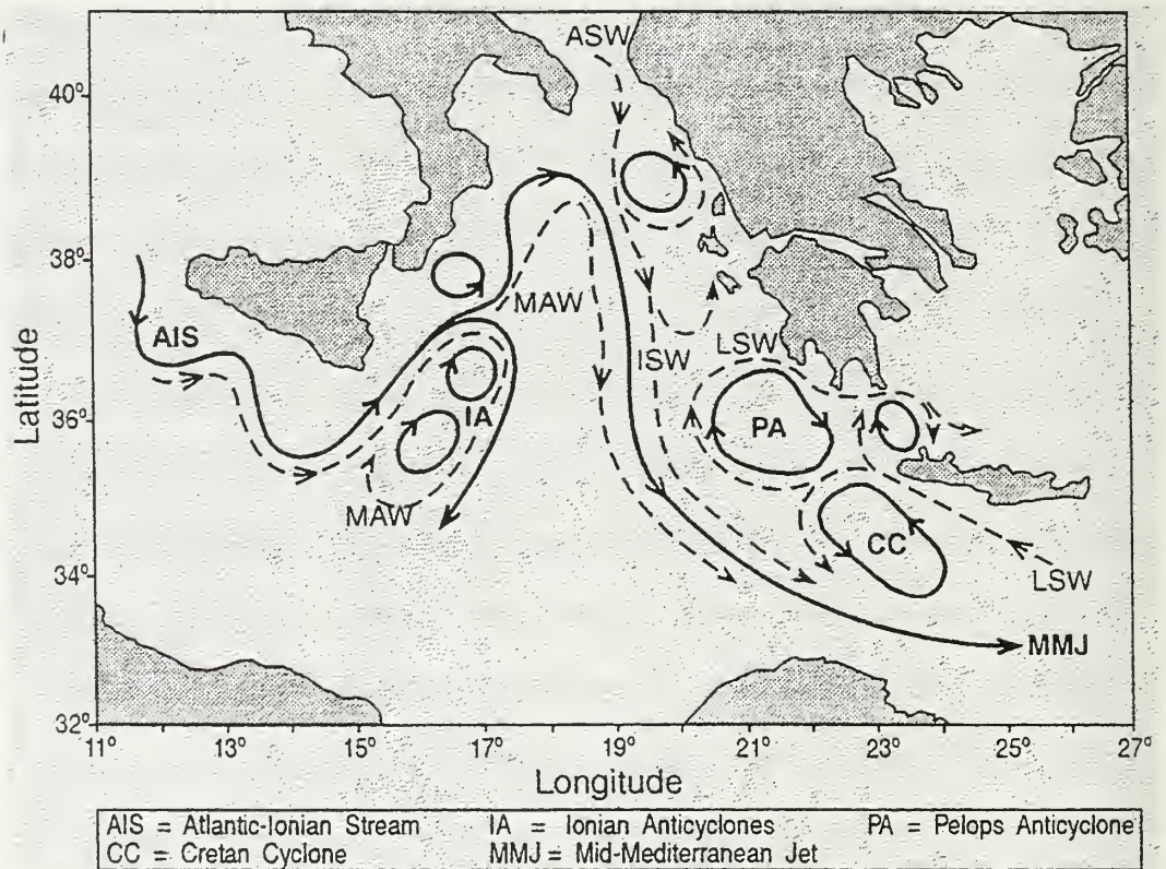
Figure II-3. Surface Mesoscale features of the Ionian Sea (from Malanotte-Rizzoli et al., 1997).
