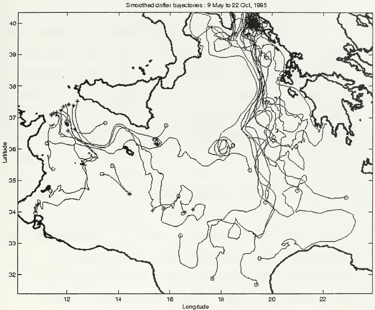
Figure III-3. Plot of drifter trajectories in the Ionian Sea from 9 May to 22 October, 1995. Star and open circle symbols denote the first (usually deployment) and last locations of the drifters, respectively.
