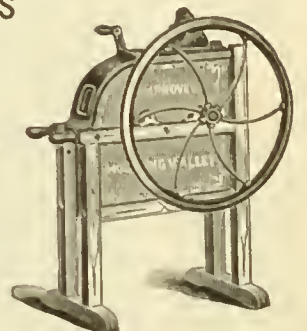
Hocking Valley Corn Sheller
