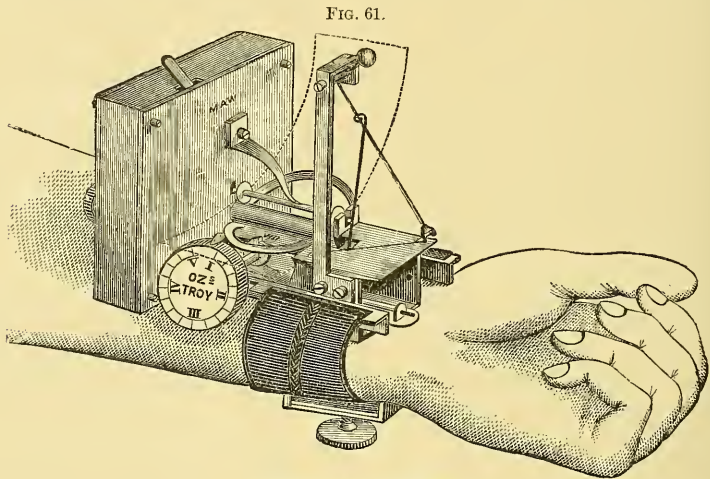
Dudgeon's sphygmograph.
