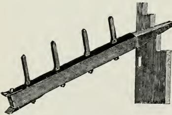
Fig. 71—PIPE JACK AND BOARD
