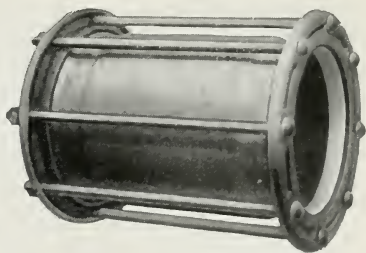
Fig. 85—ALL-STEEL LONG SLEEVES Sizes: 10 inches inside diameter to 18 inches outside diameter, inclusive. 16 inches long.
