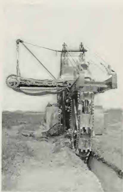
Fig. 67—REAR VIEW OF DITCHING MACHINE AT WORK
