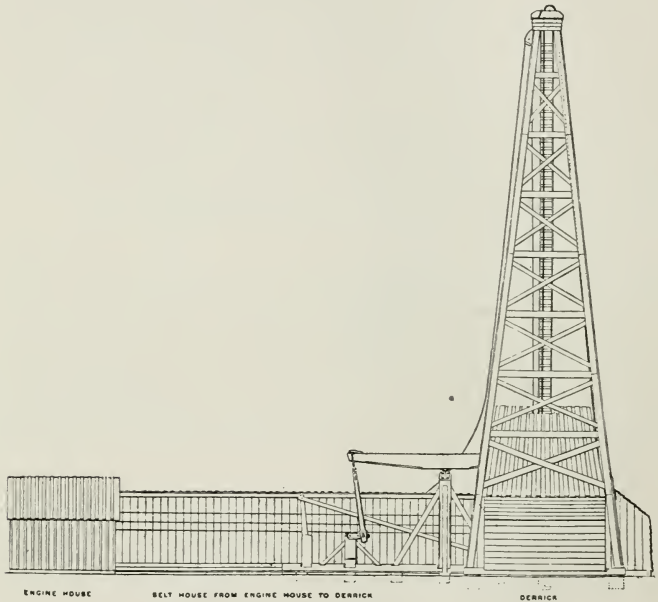
Fig. 10—CLOSED RIG
