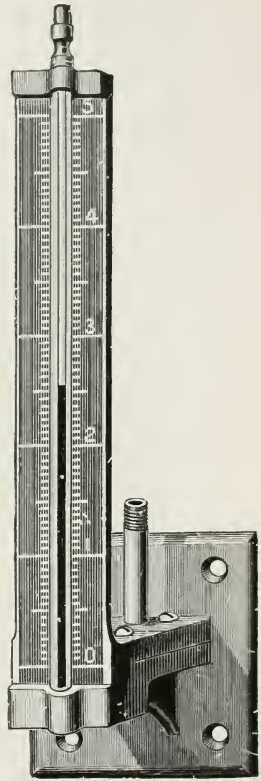
Fig. 173—MERCURY PRESSURE GAUGE
