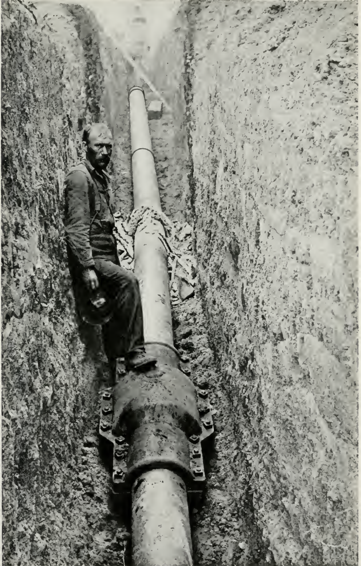
Fig 75—PIPE LINE ON RIVER BANK AT POINT OF LEAVING RIVER BED Note heavy cast iron river clamp and remains of fire where fire bend was made.
