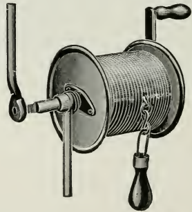
Fig. 33—STEEL LINE FOR MEASURING DEPTH OF WELL
