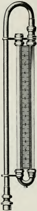
Fig. 174—SIPHON OR "U" GAUGE FOR LOW PRESSURE
