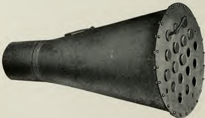
Fig. 148—FUNNEL METER WITH DETACHABLE HEAD
