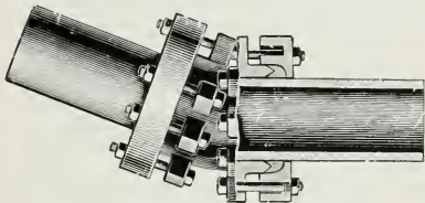
Fig. 95—ANGLE COUPLING
