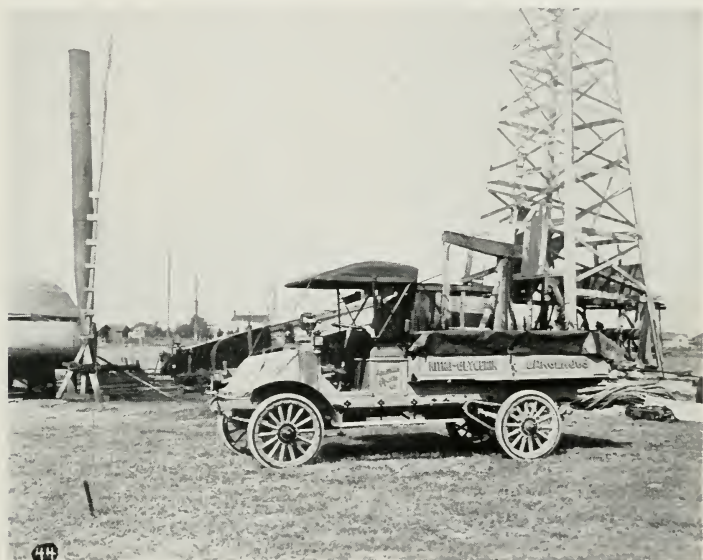
Fig. 34—A NITROGLYCERIN MOTOR TRUCK
