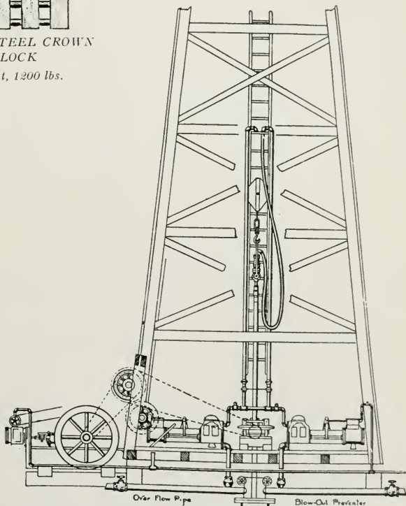
Fig. 16—HYDRAULIC ROTARY RIG
