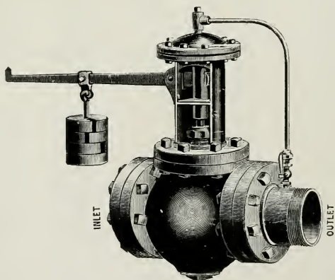
Fig. 157—HIGH PRESSURE OR REDUCING REGULATOR
