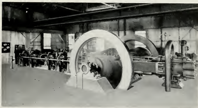
Fig. 180—INSTALLATION OF FAIRMONT GAS AND LIGHT CO., FAIRMONT, W. VA. Showing two 300 H. P. Single Tandem Gas Compressors
