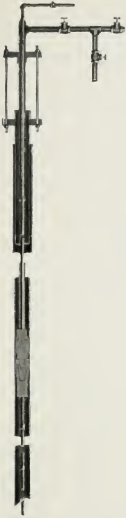
Fig. 44—Sectional View of Gas Well with 3-in. Tubing and 3/4-in. Water Siphon.
