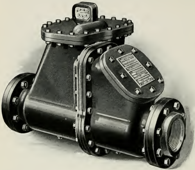
Fig. 226—A LARGE CAPACITY METER SPECIALLY BUILT TO MEASURE GASOLINE GAS
