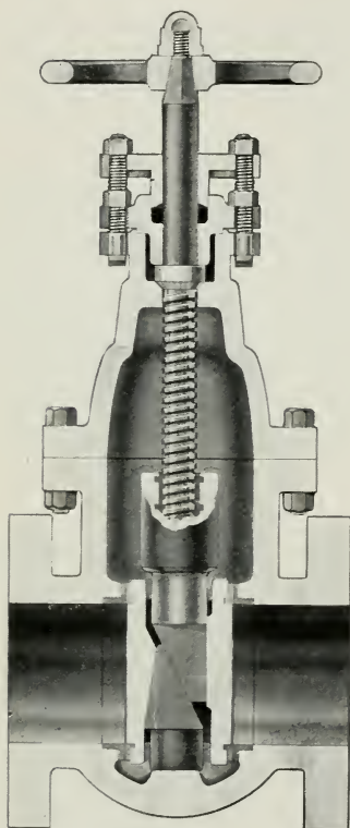
Fig. 107—SECTIONAL VIEW OF HIGH PRESSURE GATE VALVE
