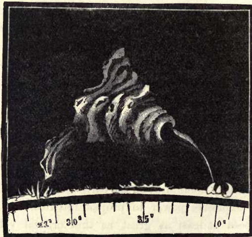
Fig. 40.—Solar Protuberance. April 6, 1892.
