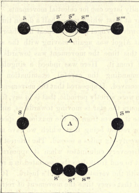
Fig. 29.—Orbit of the Companion of Algol.
