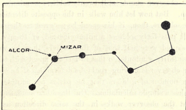
Fig. 27.—The Great Bear in 36,000 years.
