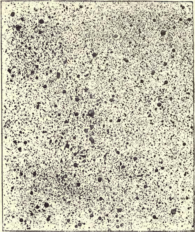
Fig. 25.—The Region of the Milky Way about \beta Cygni. Showing thousands of telescopic stars.
