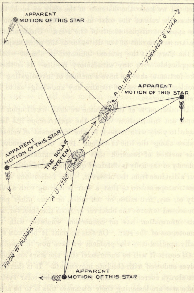
Fig. 2.—The Voyage of the Solar System.
