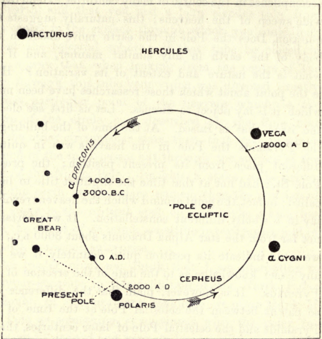
Fig. 9.—The Movement of the Celestial Pole.
