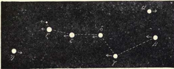
Fig. 26.—The Great Bear as it is.
