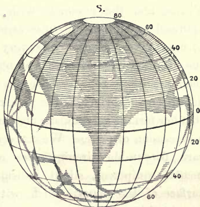
Fig. 16.—The Seasons in Mars. August 4, 1892.
