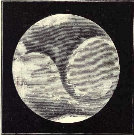
Fig. 19.—Mars through the telescope.
