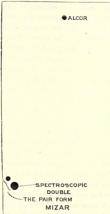
Fig. 30.—The System of Mizar.
