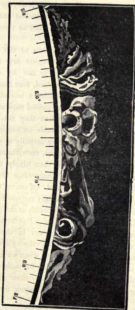
Fig. 41.—Solar Protuberance. April 15, 1892.
