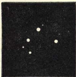
Fig. 31.—The Multiple Star (Theta Orionis) in the great nebula of Orion.
