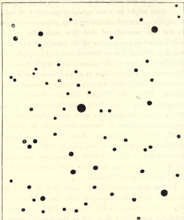
Fig. 24.—The Region of the Milky Way about \beta Cygni. Showing sixty stars.
