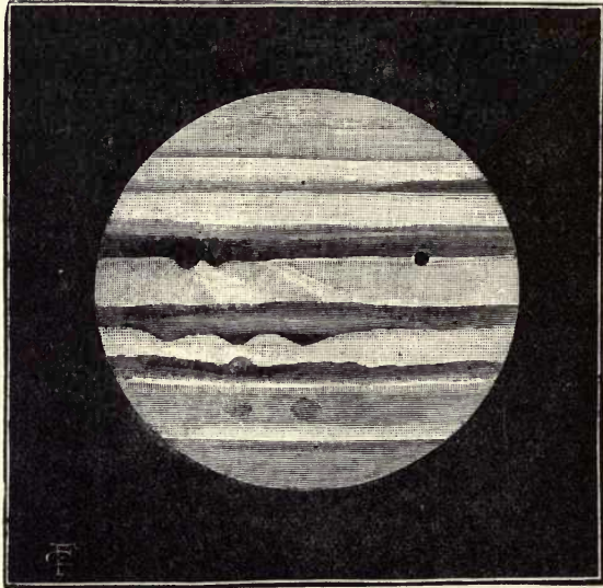
Fig. 7.—Jupiter, showing the shadow of a Satellite, October 15th, 1891.
