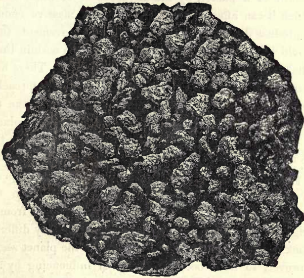
Fig. 36.—Crystals of Olivine, embedded in an iron meteorite. Found in the Desert of Atacama, South America.
