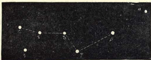
Fig 28.—The Great Bear as it will be 100,000 years hence.
