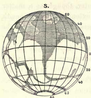
Fig. 15.—The Seasons in Mars. May 27, 1890.
