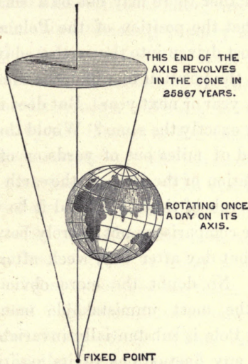
Fig. 10.—Rotation of the Pole.
