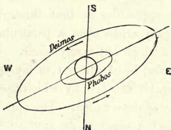
Fig. 13.—Orbits of the Satellites of Mars.
