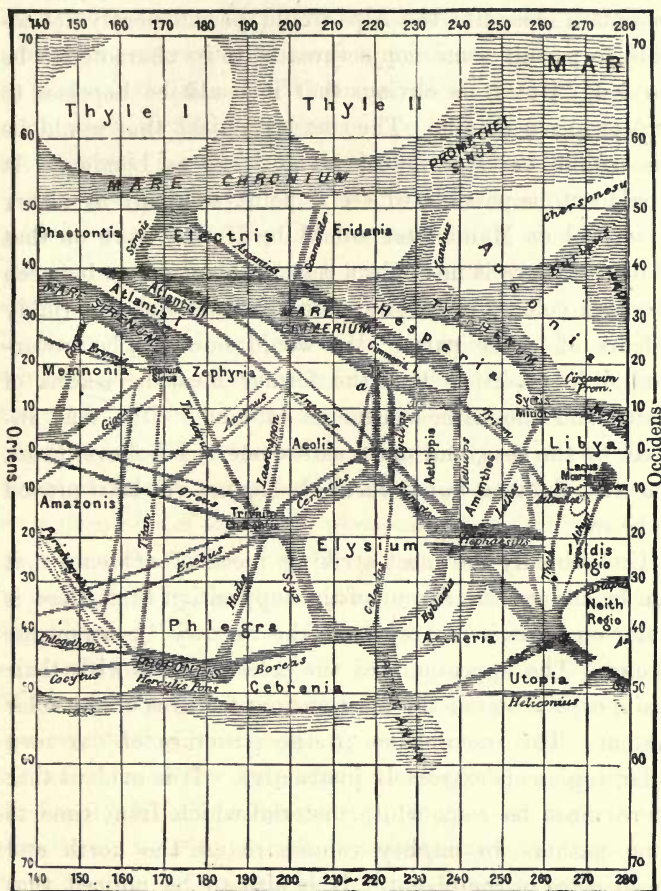
Fig. 21.—Part of a Map of Mars.
