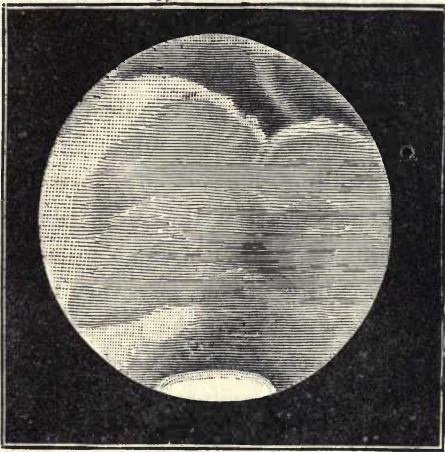
Fig. 20.—Mars through the telescope.
