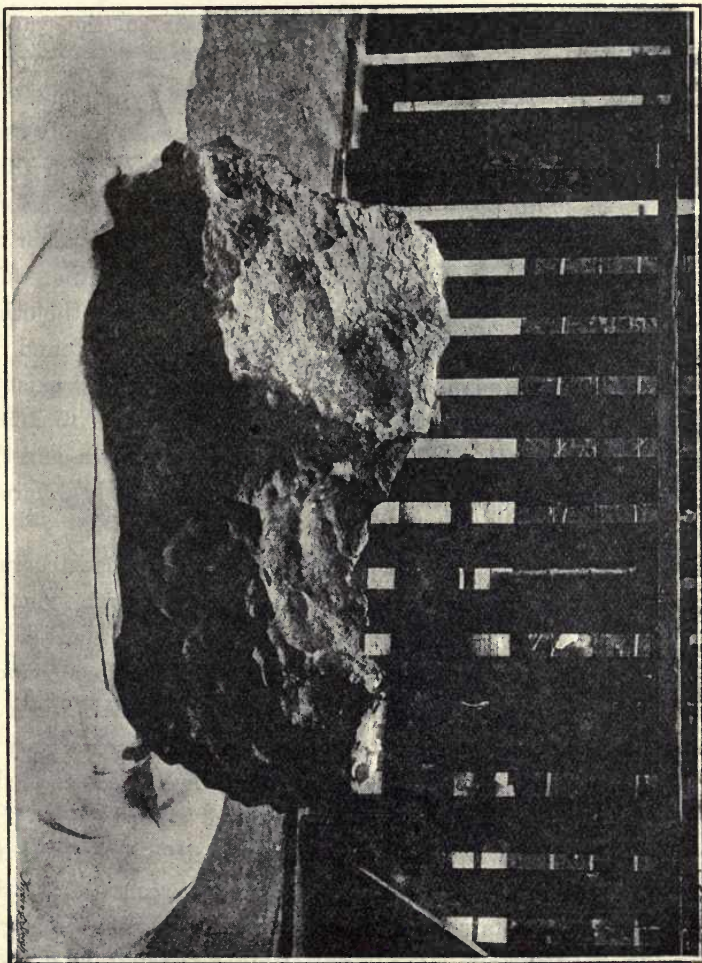
Fig. 35.—The large Yondeggin Meteorite. 4 feet 2 inches long, 2 feet 3 inches wide, 20 inches thick. Weight 2,044 lbs. (18½ cwt.).
