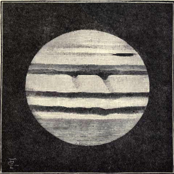
Fig. 6.—The Clouds on Jupiter, October 14th, 1891.
