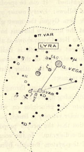
Fig. 1.—The Constellation Lyra.
