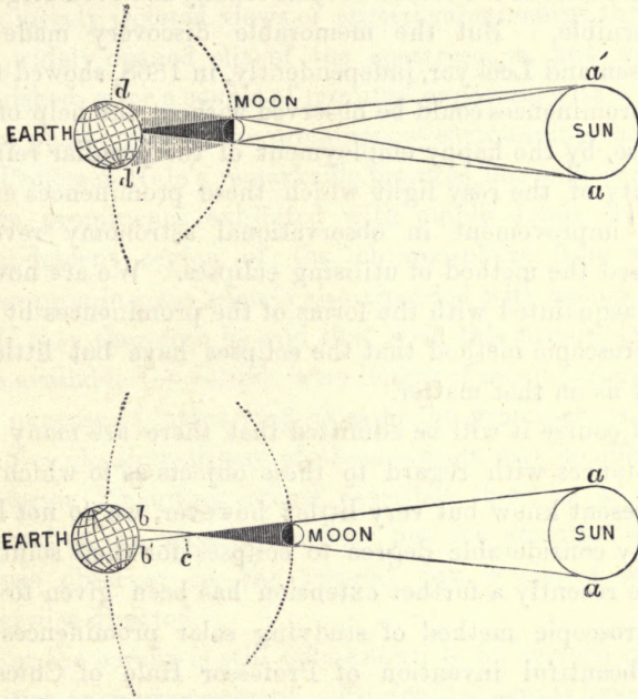
Fig. 12.—Total and Annular Eclipses.
