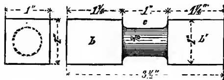
FIG. 73.—TEST-PIECE.
