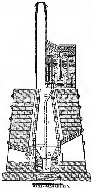
FIG. 6.—CHARCOAL FURNACE.
