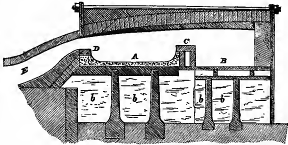
FIG. 14.—PUDDLING FURNACE—VERTICAL SECTION.
