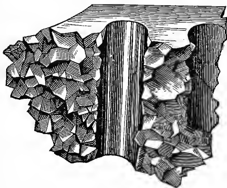
FIG. 122.—HAMMER-HEAD, MAGNIFIED.
