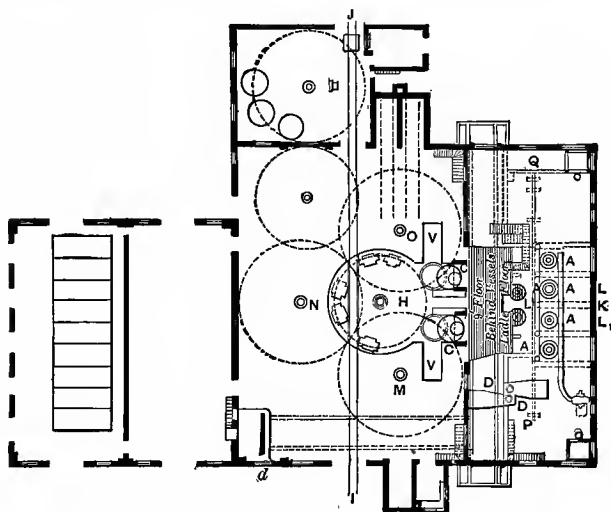
FIG. 43.—AMERICAN 5-TON BESSEMER PLANT.
