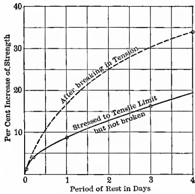
FIG. 137a.—EXALTATION OF ELASTIC LIMIT Wrought Iron—Successive Tests. U. S. Repts., 1881-82
