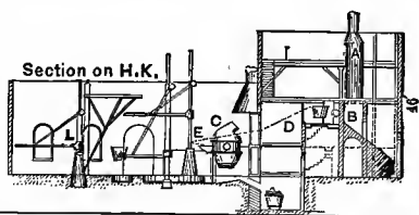
FIG. 44.—SECTION OF BESSEMER WORKS.
