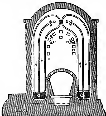
FIG. 11.—“PISTOL-PIPES.”
