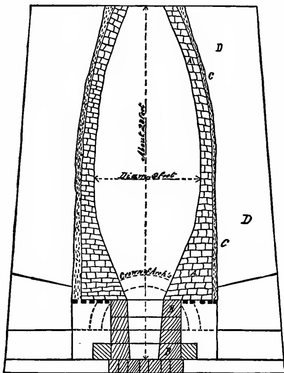
FIG. 5.—FURNACE SECTION.
