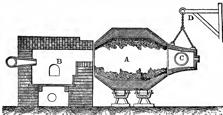
FIG. 15.—DANKS' FURNACE.
