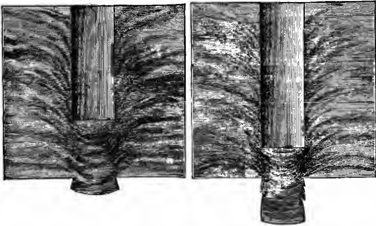
FIG. 133. PUNCHED NUTS ; FULL SIZE. FIG. 134.
