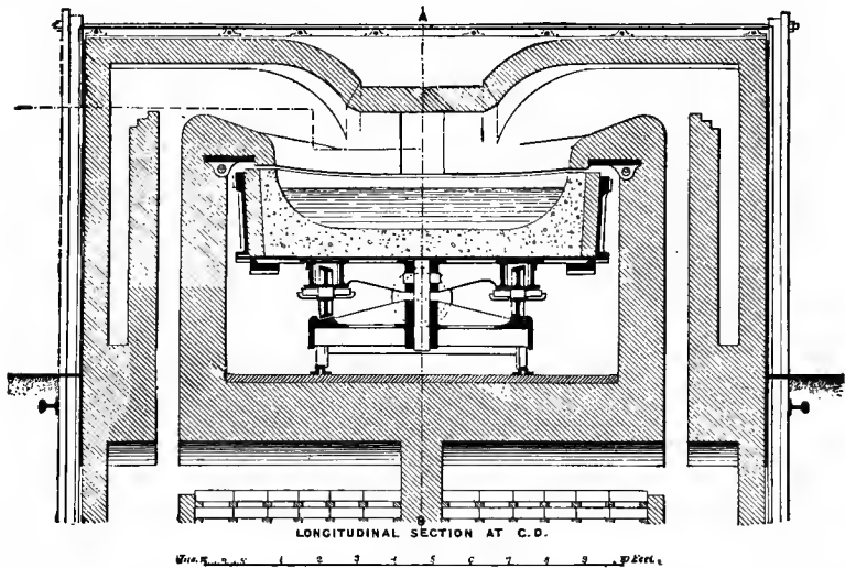
FIG. 17.—PERNOT'S FURNACE.
