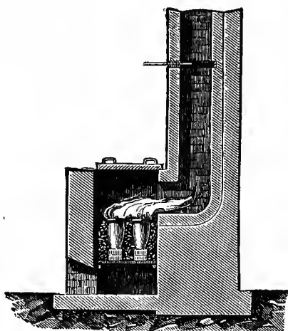
FIG. 42.—CRUCIBLE FURNACE.
