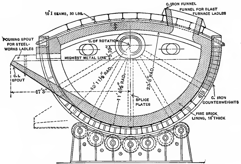
JONES' MIXER.—SECTION.
