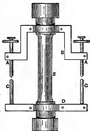
FIG. 64.—MEASURING INSTRUMENT.
