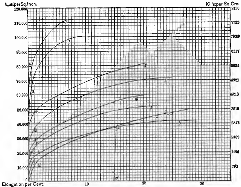
FIG. 62.—STRAIN-DIAGRAMS OF IRON AND STEEL.
