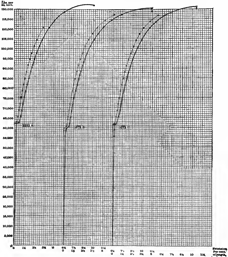
FIG. 61.—STRAIN-DIAGRAMS OF INGOT-STEEL.
