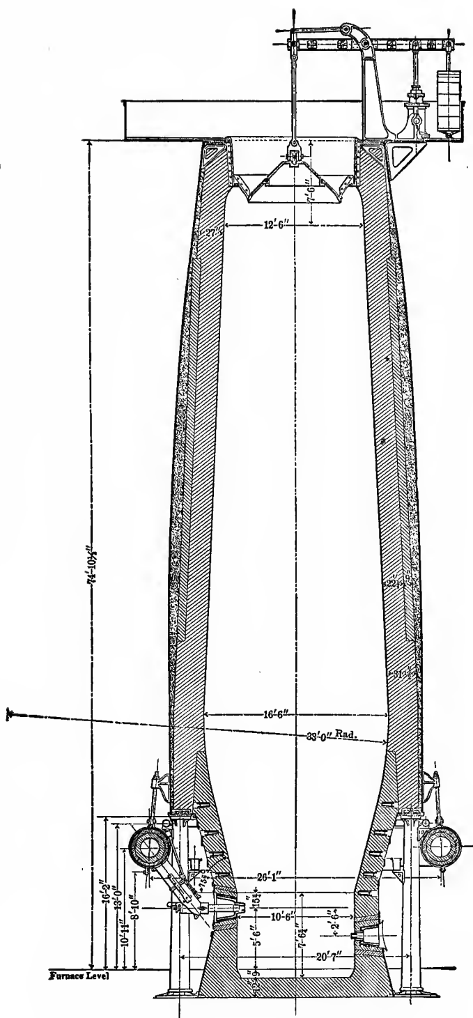
FIG. 6a.—ELEVATION DOVER (U. S.) COKE-FURNACE.
