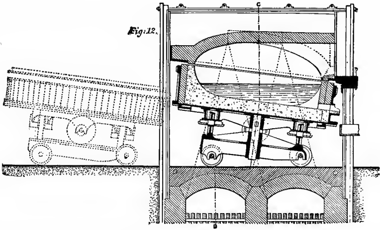
FIG. 18.—PERNOT'S FURNACE.
