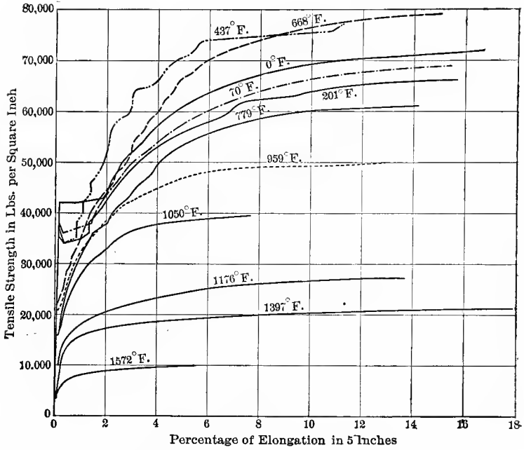
FIG. 1186.—TEMPERATURE AND TENACITY.
