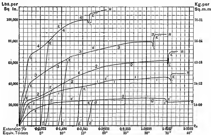
FIG. 139.—AUTOGRAPHIC STRAIN DIAGRAMS.
