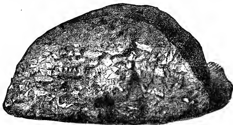
FIG. 120.—FRACTURED SURFACE OF CONNECTING ROD.
