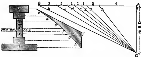
FIG. 85.—MOMENT OF INERTIA.
