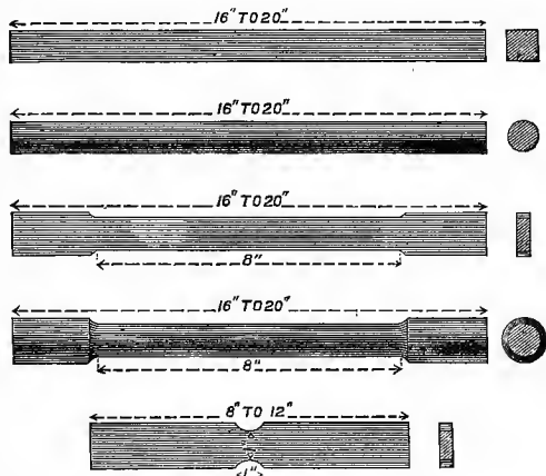
FIG. 79.—SHAPES FOR TEST PIECES.
