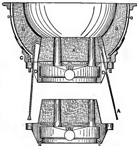
FIGS. 51, 52.—CONVERTER BOTTOM.
