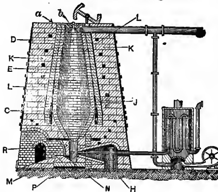
FIG. 4.—CHARCOAL FURNACE.
