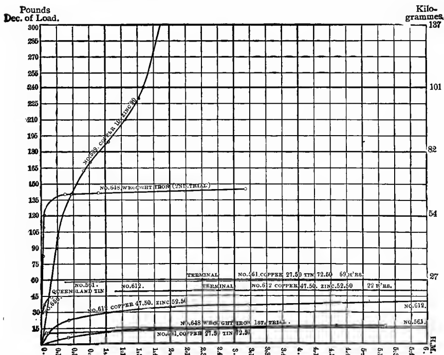
FIG. 135.—DECREASE OF RESISTANCE WITH TIME.
