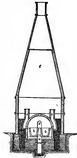
FIG. 38.—CONVERTING FURNACE.
