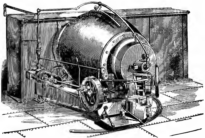
FIG. 16.—SELLERS' PUDDLER.
