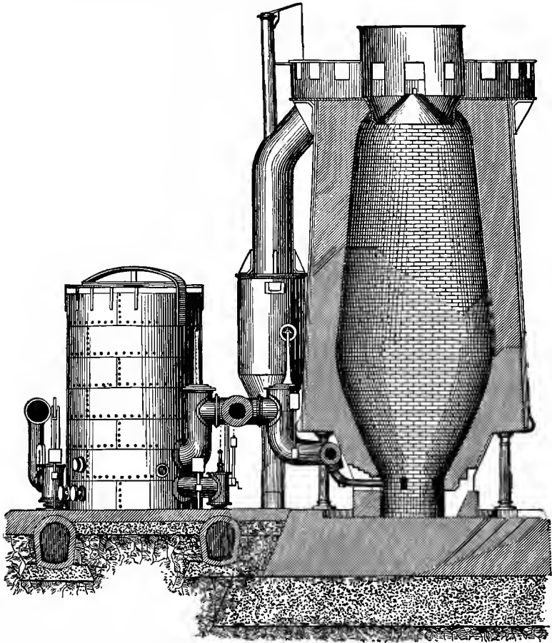
FIG. 13.—ANTHRACITE BLAST FURNACE, GAS TUBING, HOT-BLAST MAIN, AND STOVES.
