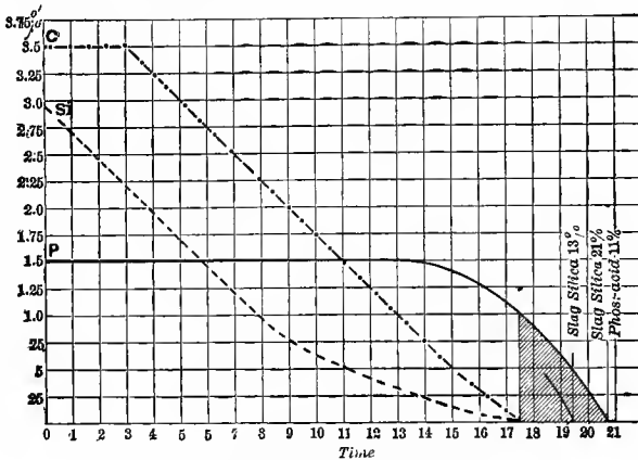
FIG. 53.—ELIMINATION OF ELEMENTS.
