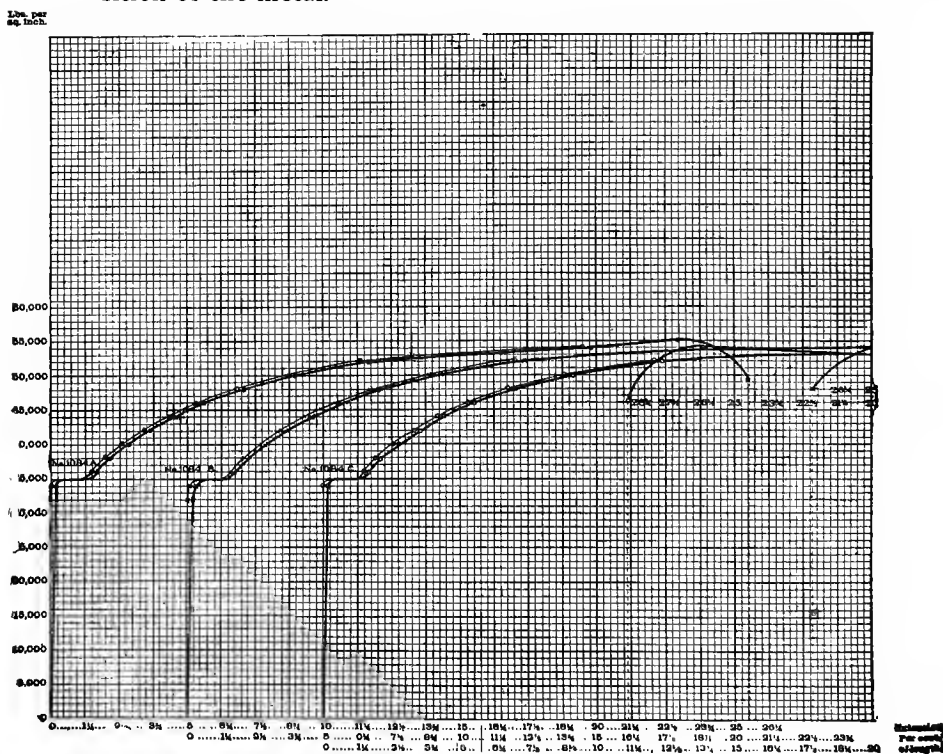
FIG. 60.—STRAIN-DIAGRAMS OF INGOT-IRON.
