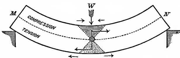
FIG. 86.—FLEXED ELASTIC BEAM.
