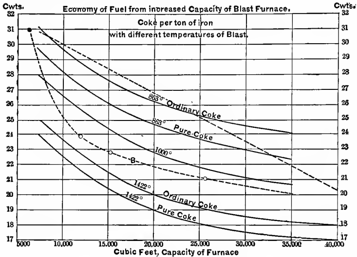
FIG. 8.—ECONOMY OF FURNACE.
