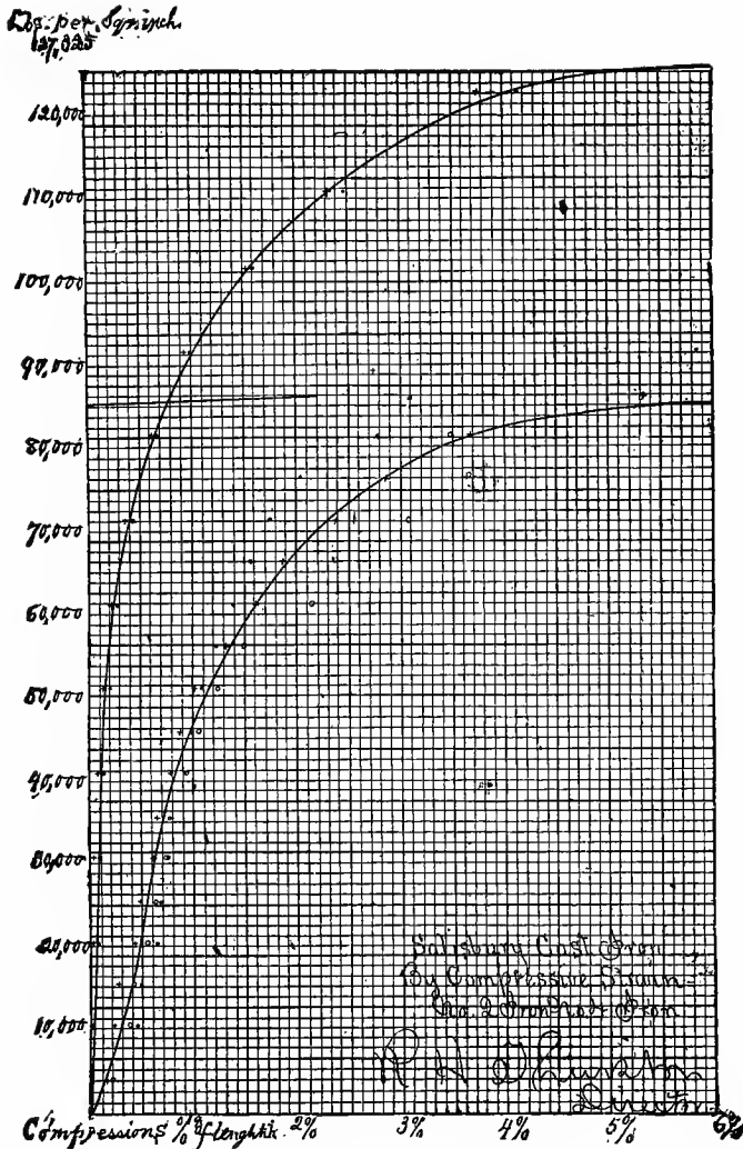
FIG. 83.—CAST IRON IN COMPRESSION.
