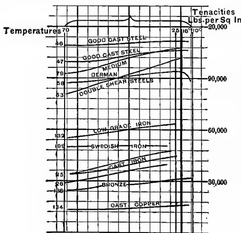
FIG. 117.—EFFECT OF COLD.
