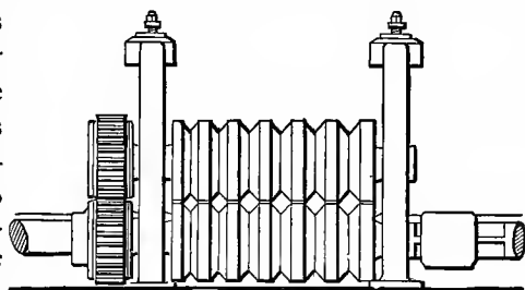
FIG. 23.—ROLLS.
