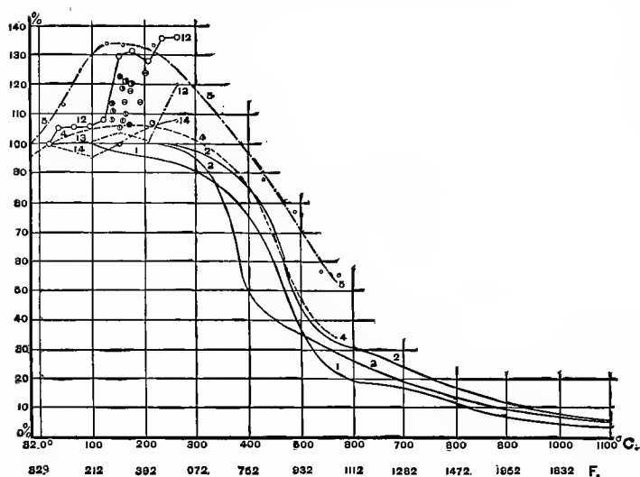
FIG. 114.—HEAT VS. TENACITY.
