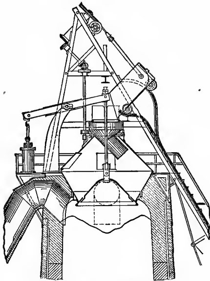
COPYRIGHTED BY GASSIEN'S MAGAZINE, NEW YORK BLAST-FURNACE TOP.
