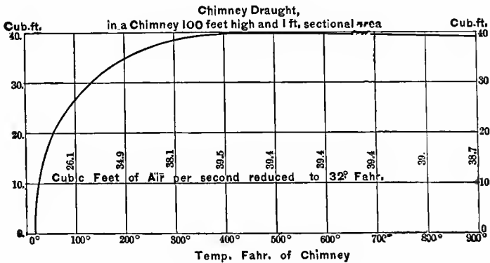
FIG. 9.—TEMPERATURE OF CHIMNEY.
