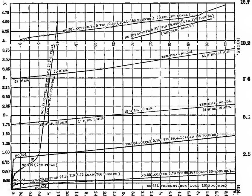
FIG. 136.—INCREASE OF DEFLECTION WITH TIME.
