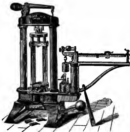
FIG. 63.—TENSION TESTING MACHINE.
