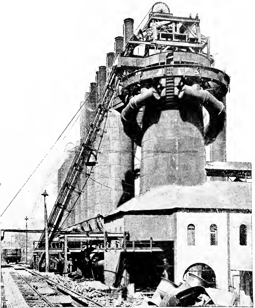
BLAST-FURNACE WITH STOVES AND BUILDINGS.
