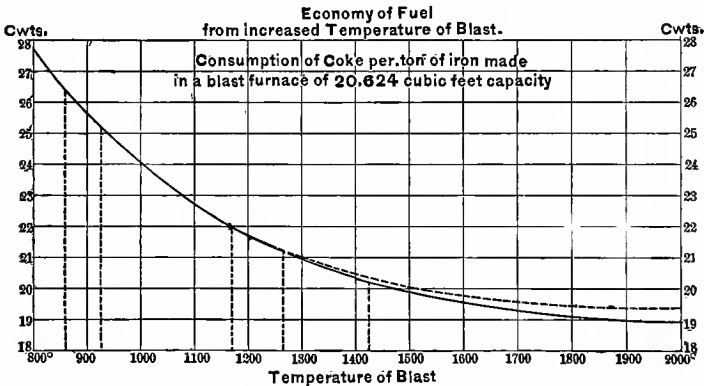
FIG. 10.—ECONOMY OF HIGH TEMPERATURES.
