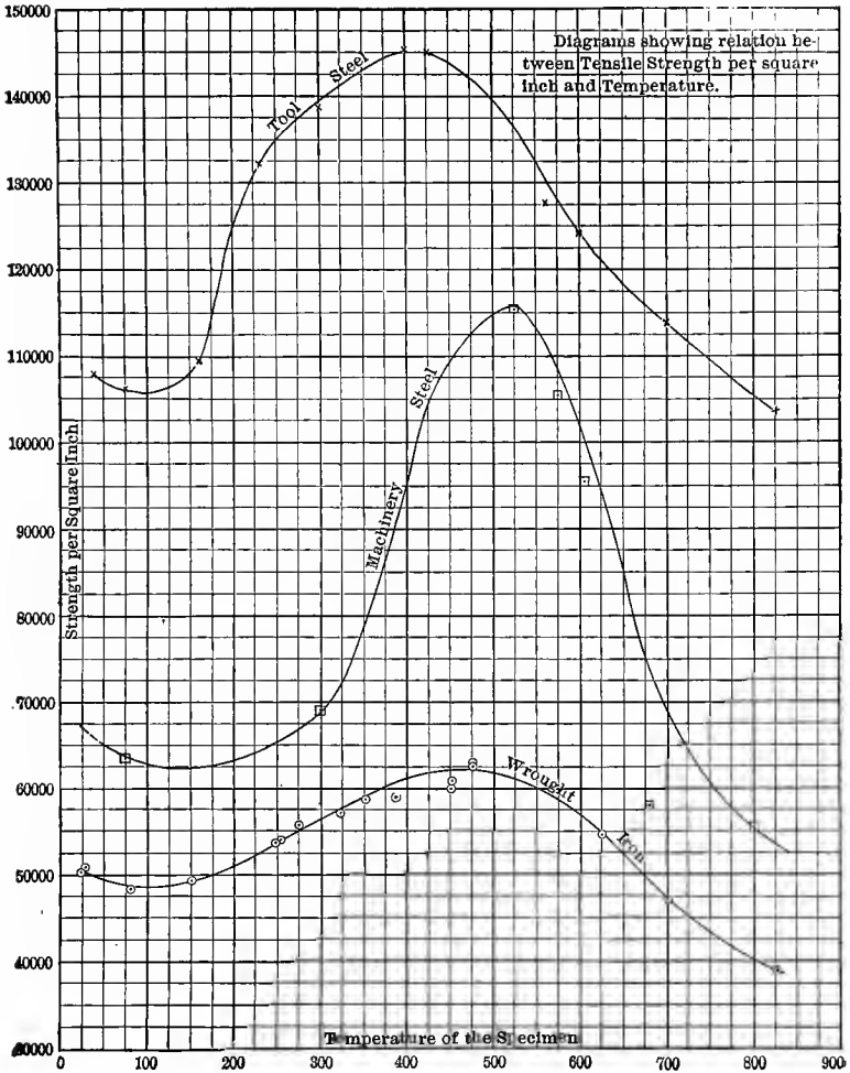
FIG. 118a.—TEMPERATURE AND TENACITY. SIBLEY COLLEGE; CORNELL UNIVERSITY.
