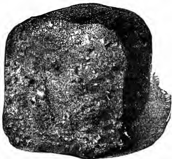
FIG. 121.—FRACTURED SURFACE OF LINK OF TESTING MACHINE.
