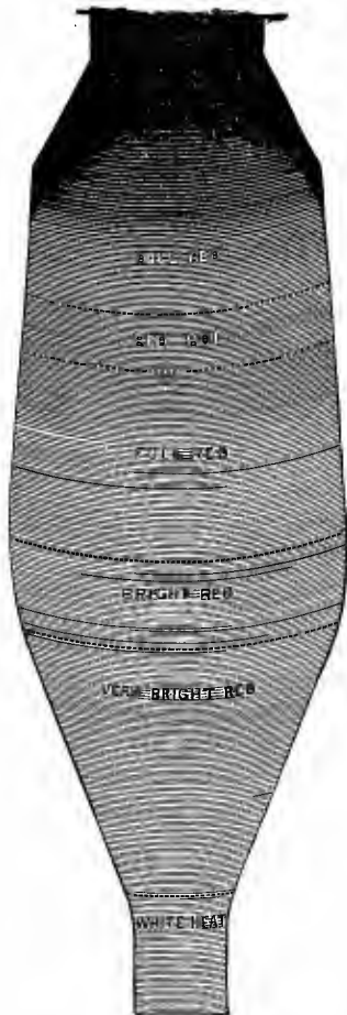
FIG. 7.—TEMPERATURES OF FURNACE.
