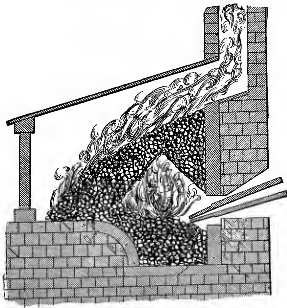
FIG. 3.—THE CATALAN FORGE.
