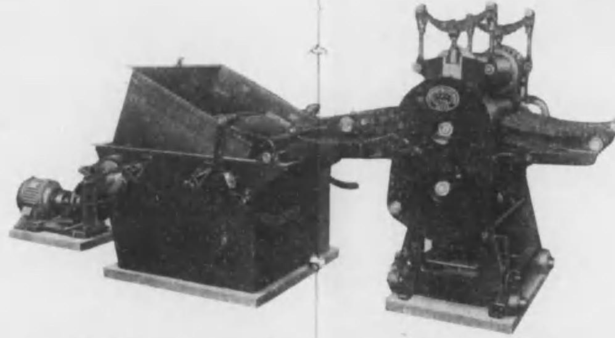
Helington Type, Dying Machine for Staple Fibre.
