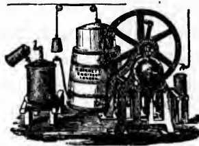
DIRECT-ACTION MACHINE.
