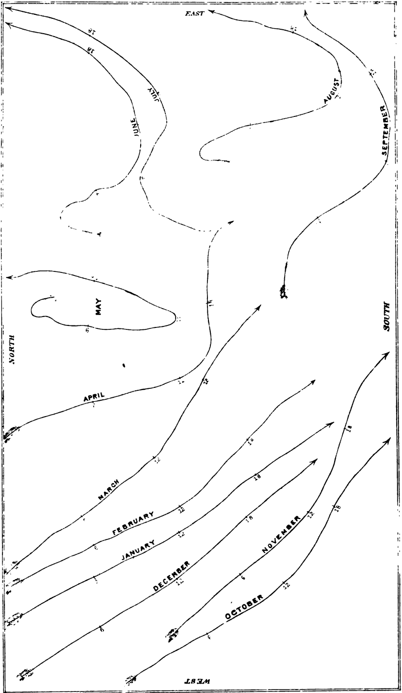
Plate VIII. DIURNAL CHANGE IN THE DIRECTION OF THE WIND AT A POINT IN THE SEA
