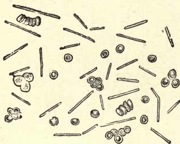
Fig. 69.— Bacillus anthracis , produced in guinea-pig by inoculation: corpuscles of blood and bacilli.
