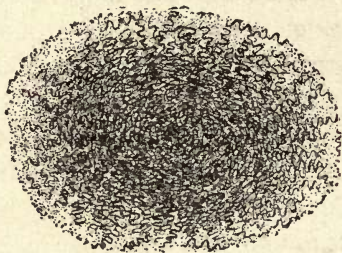
Fig. 62.—Zoogloea of Spirillum tenue .
