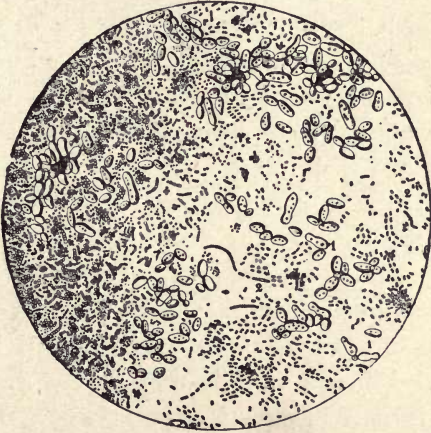
Fig. 53.—The disease acescence , which sours wine. Deposit seen in the microscope; 1, 1, Mycoderma vini ; 2, 2, Mycoderma aceti , still young; 3, the same older, when the mischief is at an advanced stage.
