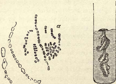
Fig. 82.—Bacterium of dental caries: a , b , different forms obtained in gelatine culture.
