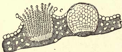
Fig. 6.—Section of a barberry-leaf bearing two œcidiospores, more or less developed, of Puccinia graminis (much magnified).
