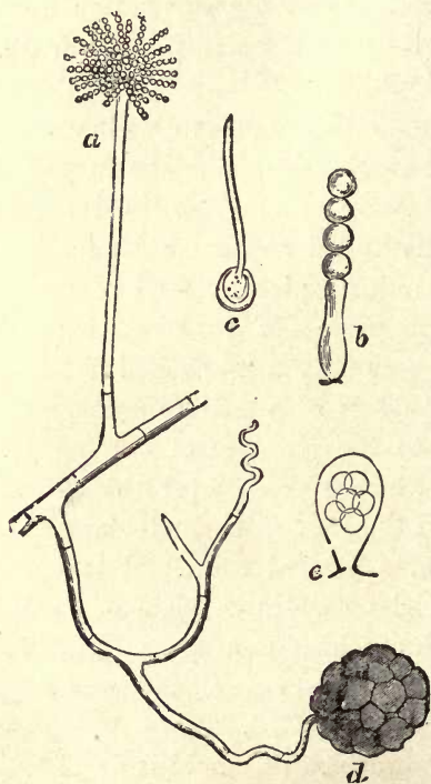
Fig. 13. — Aspergillus glaucus , mould on leather and rotten fruits : a , hypha bearing the chaplet of spores b ; c , a germinating spore; d , ball of Eurotium; e , ascus enclosing the endogenous spores (magnified).
