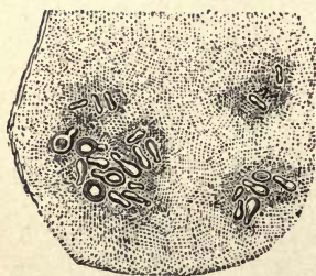
Fig. 32.—Epidermic cell of skin covered with hair, affected by Pityriasis simplex , and covered with spores ( \times 1000 diam.).
