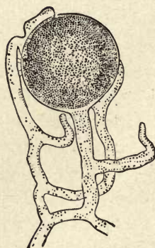
Fig. 22.—Oogonium of Saprolegnia surrounded by Antheridia (much magnified).
