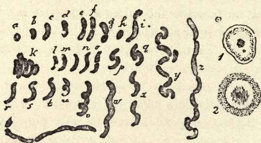
Fig. 87.—Cholera microbe, or Bacillus comma (Koch): a-z, the different forms which it presents in its growth and division into cells (greatly magnified); 1, 2, cultures of bacillus, under a simple lens.
