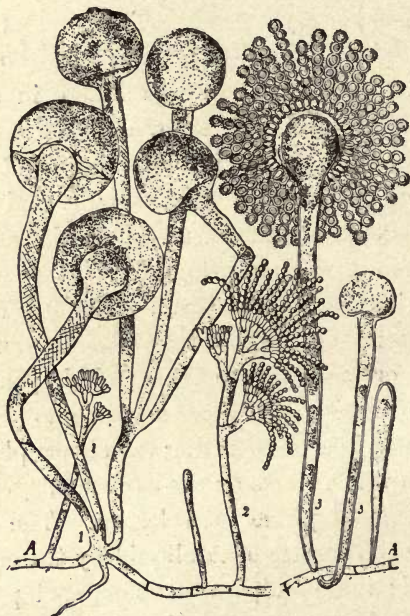
Fig. 107.—The penicillium ferment (Cocardas). Aerial fructification in extract of liquorice: the three forms, Mucor (1), Penicillium (2), Aspergillus (3), borne by a single hypha A ( \times 225 diam.).
