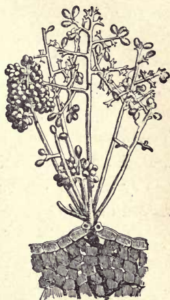
Fig. 18.—Group of tufts of Peronospora infestans , issuing from a stoma on the lower surface of the leaf and bearing the summer spores ( \times 120 diam.).
