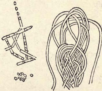
Fig. 68.— Bacillus anthracis of splenic fever in different stages of development: bacilli, spores, and curled filaments (much enlarged).
