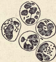
Fig. 94.—Cells of gonorrhœal pus 24 hours after its discharge. Within may be seen several forms of fission of their nuclei, and micrococci moving in the protoplasm ( \times 600 diam.)
