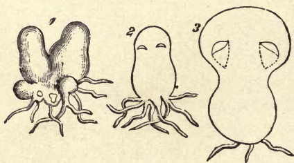
Fig. 1.— Agaricus in different stages of development : 2, 3, a vertical section showing the formation of the head. The hyphae of the mycelium are shown in the lower part of the figure.
