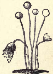
Fig. 14.— Mucor caninus , the mould on dog's excrement (magnified).
