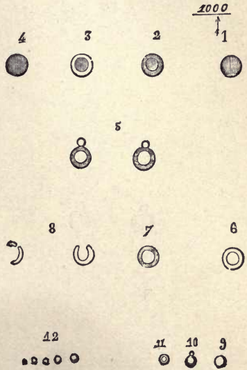
Fig. 31.—Isolated spores, taken from patches of pelade: 1, 2, 3, 4, large spores; 5, budding spores; 6, 7, 8, empty spores; 9 to 12, small spores ( \times 1000 diam.).
