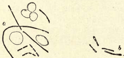
Fig. 71.— Septic vibrio , bacillus of malignant œdema (Koch): a , taken from spleen of guinea-pig; b , from a mouse's lung.
