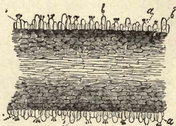
Fig. 3—Spores of the hymenium , greatly magnified, and resting on their supports or basides , a.
