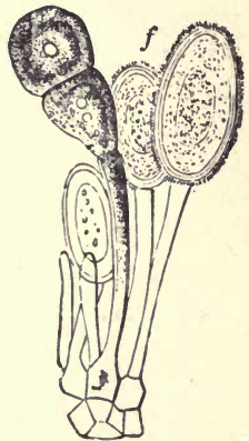
Fig. 5.—Part of a patch of Puccinia graminis , taken from a blade of wheat, and displaying several uredospores and one teleutospore (much magnified).
