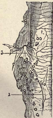
Fig. 30.—Hair affected by the rapid progress of Pelade décalvante . It is surrounded by epidermic cells charged with spores ( \times 208 diam.).
