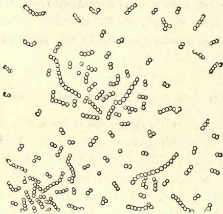
Fig. 59.— Micrococcus ureæ (Von Tieghem). Microbe of ammoniacal fermentation. It may be observed that the bacterium is in the figure 8, or in chaplets. (Much magnified.)
