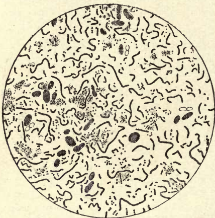
Fig. 55.—Disease of ropiness in wine, affecting champagne, and caused by a bacterium which assumes two forms: the figure 8, and chaplets.
