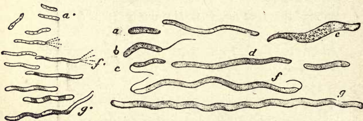
Fig. 79.— Vibrio rugula (Warming) in different stages of development: b, c, f , individuals with vibratile cilia ( flagellum ); f' , ciliated spores. Found in the human mouth and intestines.
