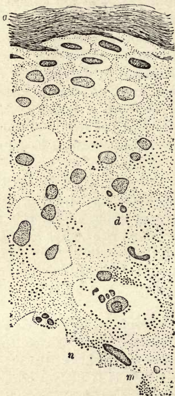
Fig. 91—Section of skin covering a small-pox pustule. a , horny layer of the epidermis; d , adenoid tissue; m , m , micrococci stained with methyl violet ( \times 850 diam.).
