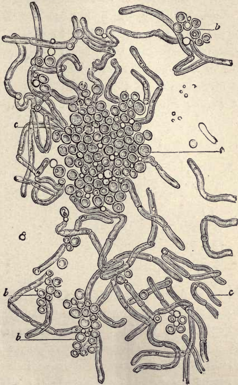
Fig. 28.— Microsporon furfur : a, b, groups of spores ; c, mycelium with long, transparent, and curved articulations.
