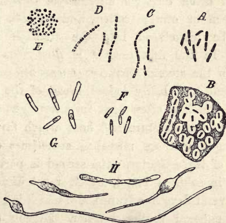
Fig. 67.— Bacterium cyanogenum , microbe of blue milk (Neelsen). It is probable that several different forms are here confused under this name. B, zoogloea.
