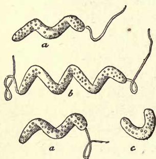
Fig. 65.— Ophidomonas sanguinea of stagnant water (slightly magnified).
