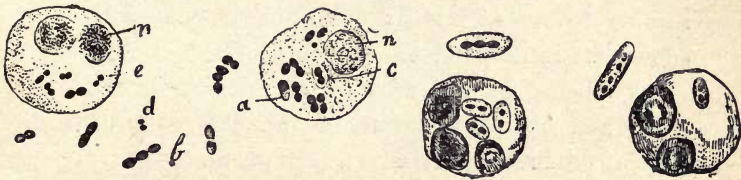
Fig. 93.—Micrococci in sputum of pneumonia: b, d , free, or encysted in the lymphatic cells a, c ; n , nuclei of cells (much enlarged).
