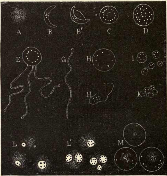
Fig 84.—Parasite of intermittent fever (Laveran): A, normal hæmatin; B, B', corpuscle No. 1; C, corpuscle No. 2, motionless; D, corpuscle No. 2, containing mobile pigmented grains; E, corpuscle No. 2, provided with mobile filaments; G, detached mobile filament; H, H', corpuscle No. 3; I, K, corpuscle No. 2, of small size, red and agglomerated; L, L', hæmatins to which the small corpuscles No. 2 are attached; M, pigmented leucocytes, their nuclei made visible by carmine.
