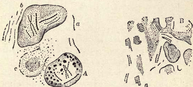
Fig. 91A.—Bacilli in the sputum of a consumptive patient: A, bacilli, either isolated (a) or in the epithelial (b) and pigmented (c) cells of the lung; B, numerous bacilli, massed together in the sputum. Stained by Ehrlich's process with methyl violet (much enlarged).
