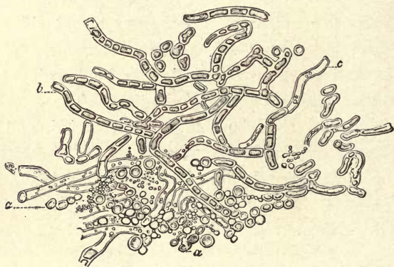
Fig. 24.— Achorion Schœnlenii , fungus of ringworm ( \times 400 diam): a, spores; b, chains of spores; c, mycelium.
