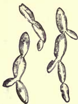
Fig. 43.— Sacch. mycoderma , or wine-flowers ( \times 350 diam.).
