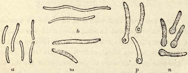
Fig. 63.— Vibrio rugula in different stages of development (anaërobic), much enlarged.
