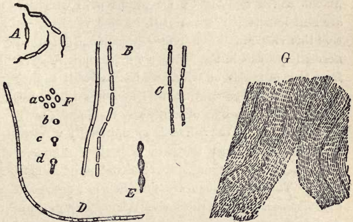
Fig. 80.— Bacterium (Bacillus) subtilis (Zopf), in different stages: A , ciliated rods; E , F , spores; G , Zoogloea. In infusions of hay, and in the human mouth (much magnified).
