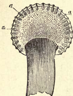
Fig. 11.—One of the heads or organs of fructification in ergot, still more magnified. a , peritheces.
