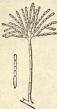
Fig 19.— Chaetonium chartatum , mould on paper.
