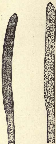
Fig. 21.—Two filaments of Saprolegnia containing spores (greatly magnified).
