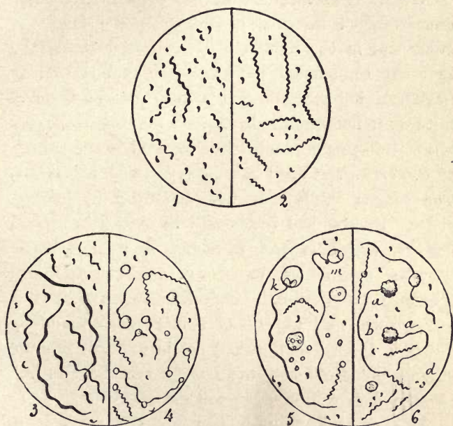
Figs. 88, 89, 90.—Evolution of cholera microbe ( Peronospora Ferrani ; Ferran): 1. Cholera microbe ( Bacillus komma ), discovered by Koch. 2. Spiral form of bacillus, transferred from gelatine to an infusion. 3. Degeneration of spiral form after a series of successive cultures. 4. Cholera microbe ( Peronospora Ferrani ): development of oogonium on the spirilla and straight filaments. 5. The oogonium is filled with granules which centre in a point k , and it is then converted into an oosphere; m , pollinidium on fertilizing organ. 6. The oosphere is converted into mulberry-shaped and comma-shaped bodies.
