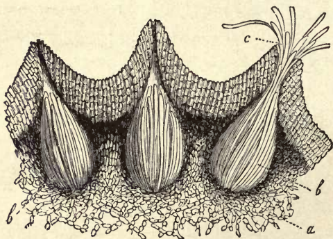
Fig. 12.—Portion of preceding figure under a very high magnifying power, showing at b the asci, and at c the spores issuing from the asci or peritheces.
