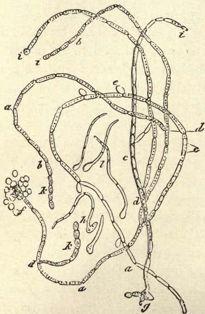
Fig. 34.— Oidium albicans , or Saccharomyces mycolerma : d . much-branched mycelium; g , chaplet or torula of spores, giving birth at f , k to the mycelium.
