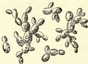
Fig. 36.— Saccharomyces ellipsoïdeus , wine ferment, in process of budding ( \times 600 diam.).
