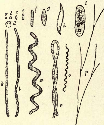
Fig. 51.—Different forms of microbes, or bacteria: a, b, c, d , Micrococcus of various forms; e , the short Bacterium ; f , the short Bacillus ; k , Leptothrix or long bacillus; l , Vibrio , dividing by fission; m , Spirillum ; n , Spirillum ; o , Spirochæte ; p , Cladotrichia , etc. (from Zopf: highly magnified).
