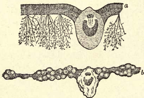
Fig. 17.—Mildew: a , vertical section of a leaf, bearing tufts of Peronospora viticola on its lower surface; b , a withered leaf, bearing the winter spores ( oospores ) ( \times 20 diam.).
