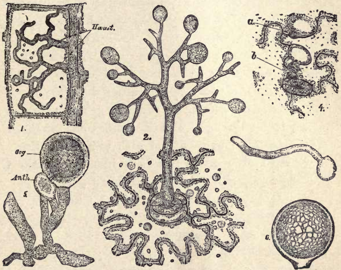
Fig. 16.—Reproductive organs of Peronospora calotheca (much magnified).
