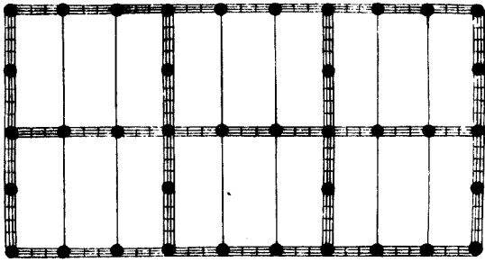
殿間身地盤九間分心斗底槽
