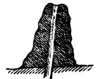
Fig. 2 Crayfish mound
