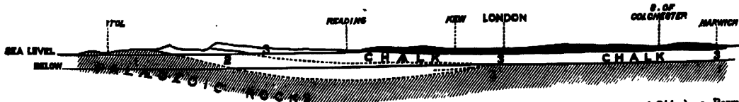
Section from Bristol to Harwich, showing the probable range of the Palaeozoic Rocks. 1, Palaeozoic Rocks (Carboniferous and Older); 2, Permian to Upper Greensand; 3, Chalk.
