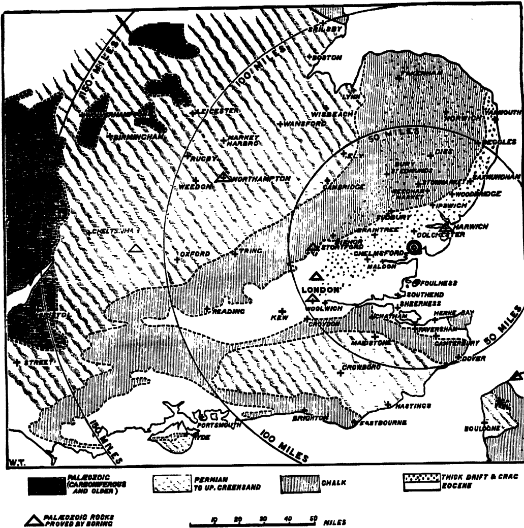
Map of the Earthquake of April 22, 1884. N.B.—The places marked are those at which the shock was felt. In the East of England only the more important of such places are marked.
