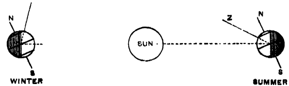
FIG. 46.—Diagram showing the variation of the sun's zenith distance from solstices to solstices. N, north pole of the earth; S, south pole; Z, zenith of Greenwich.
