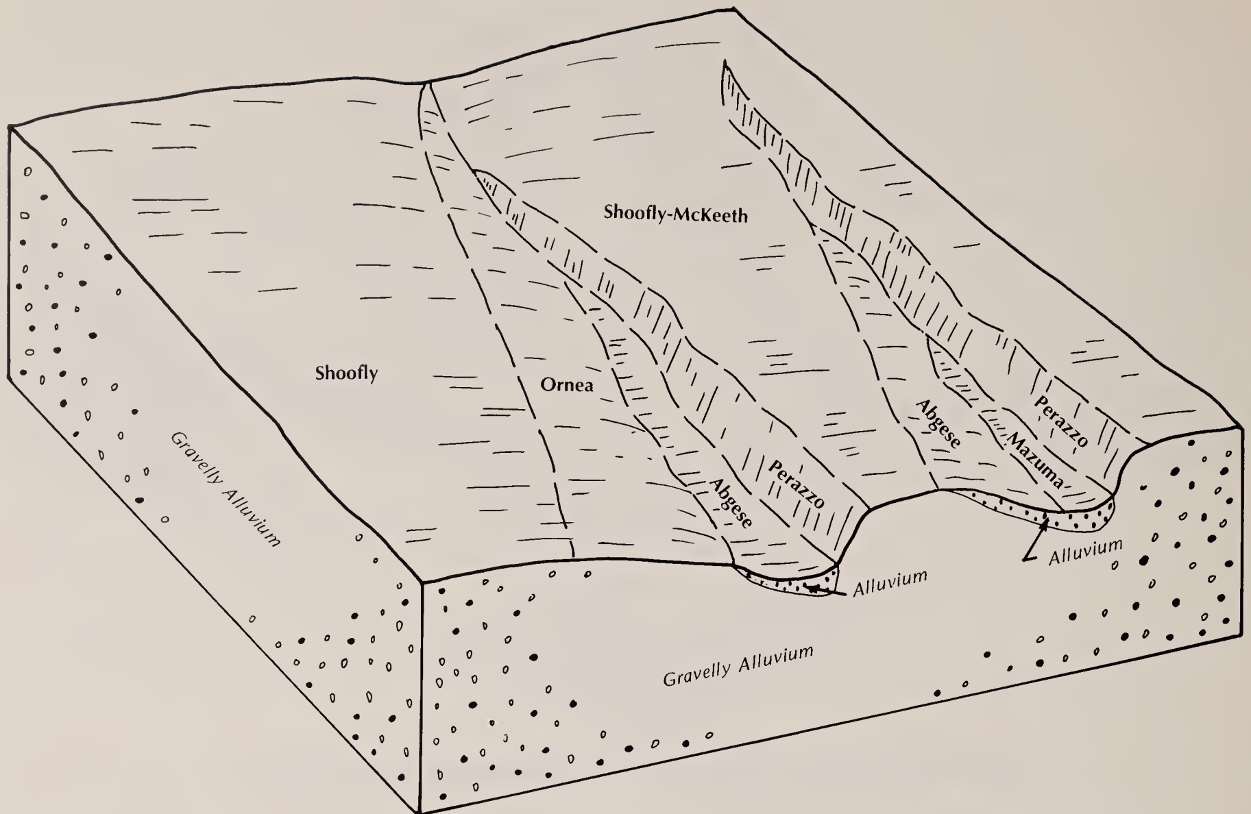
Figure 3.—Typical pattern of soils and underlying material in general soil map unit 5.
