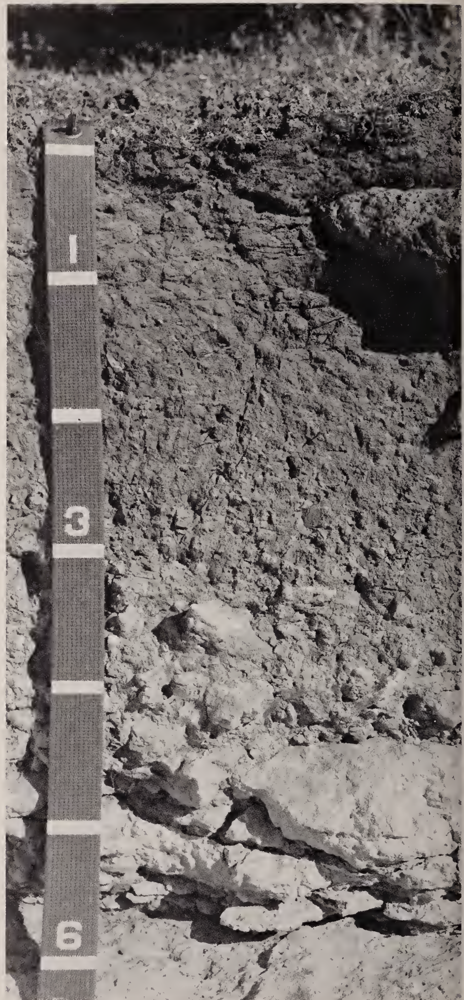
Figure 11.—Profile of Colthorp stony silt loam in an area of Colthorp-Kunaton complex, 0 to 8 percent slopes (numerals on tape indicate decimeters). A hardpan at a depth of 12 inches (3 decimeters) overlies basalt.
