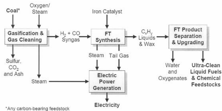
Figure 4. Process Flow Diagram for CTL facility.
