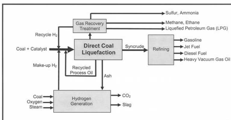
DCL Process Block Flow Diagram
