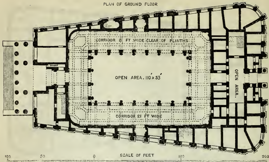
GROUND PLAN OF ROYAL EXCHANGE.
