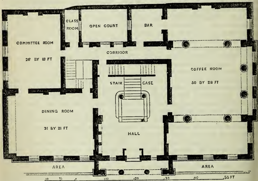
UNIVERSITY CLUB-HOUSE, ELEVATION AND PLAN.
