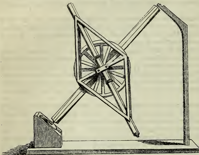
PROPOSED MOUNTING OF MR. READE'S EQUATORIAL.
