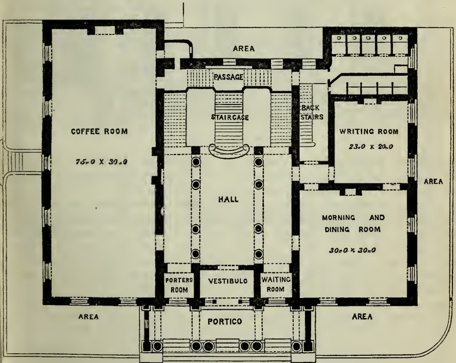
ATHENÆUM CLUB-HOUSE, ELEVATION AND PLAN.
