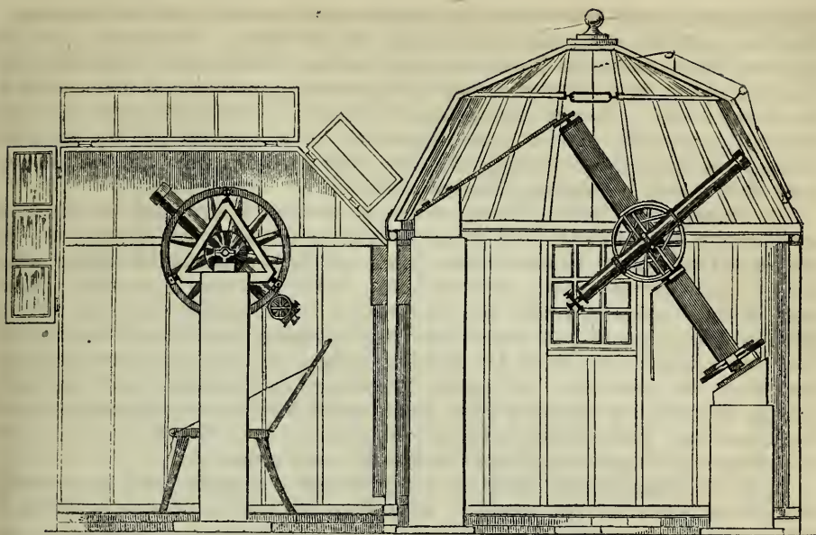
SECTIONAL VIEW OF MR. DREW'S OBSERVATORY.
