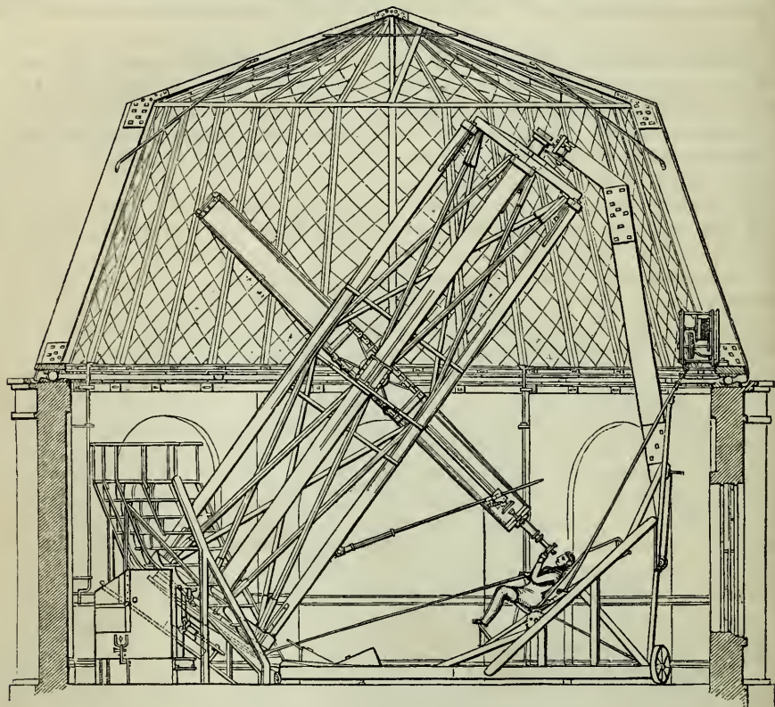
THE NORTHUMBERLAND TELESCOPE.
