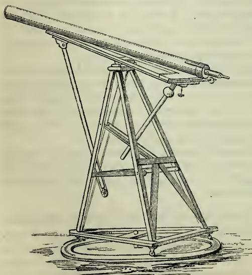
MOUNTING OF MR. READE'S 12-FT. TELESCOPE.
