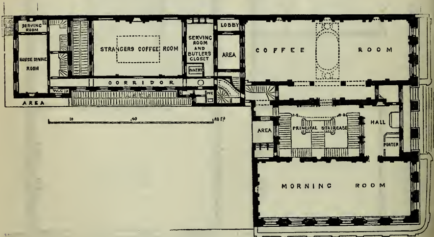
PLAN OF ARMY AND NAVY CLUB-HOUSE.
