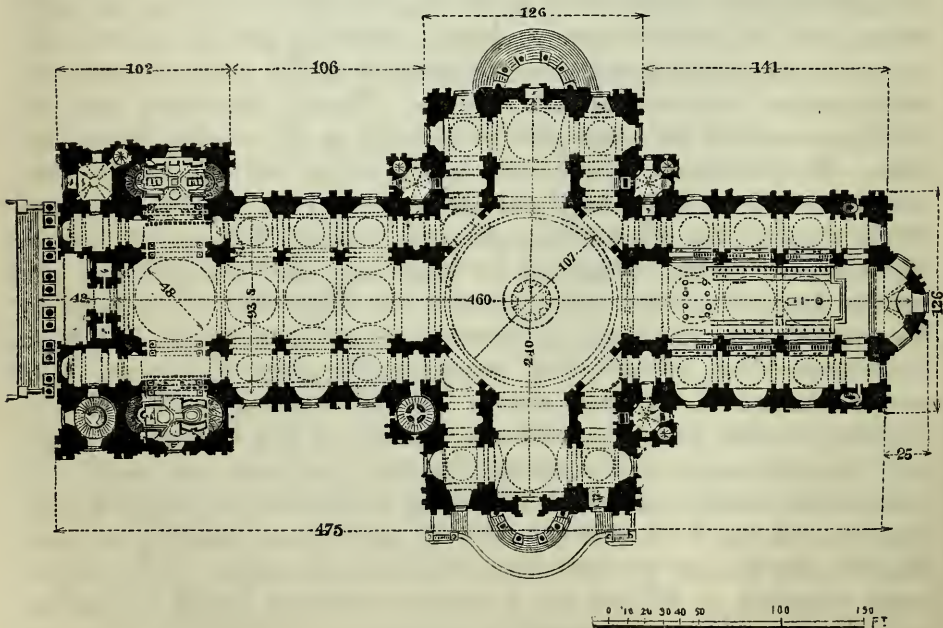
PLAN OF ST. PAUL'S.
