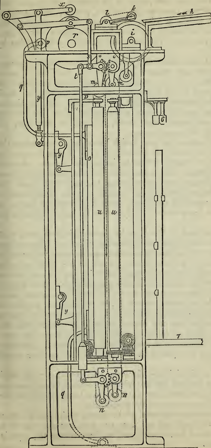
Plate 4.—END VIEW OF FEEDING APPARATUS.
