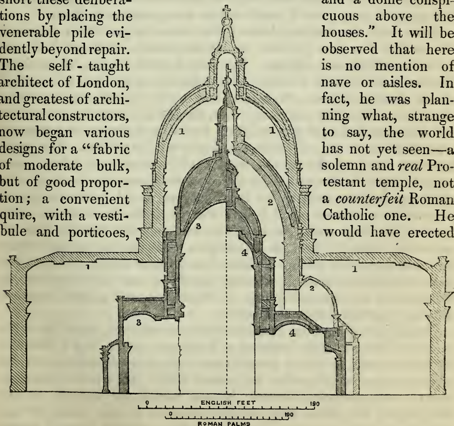
Sections through the transept and dome of St. Peters (1 1 1 1), Florence Cathedral (2 2), London ditto (3 3), and St. Genesève, Paris (4 4), showing their comparative widths and heights.
