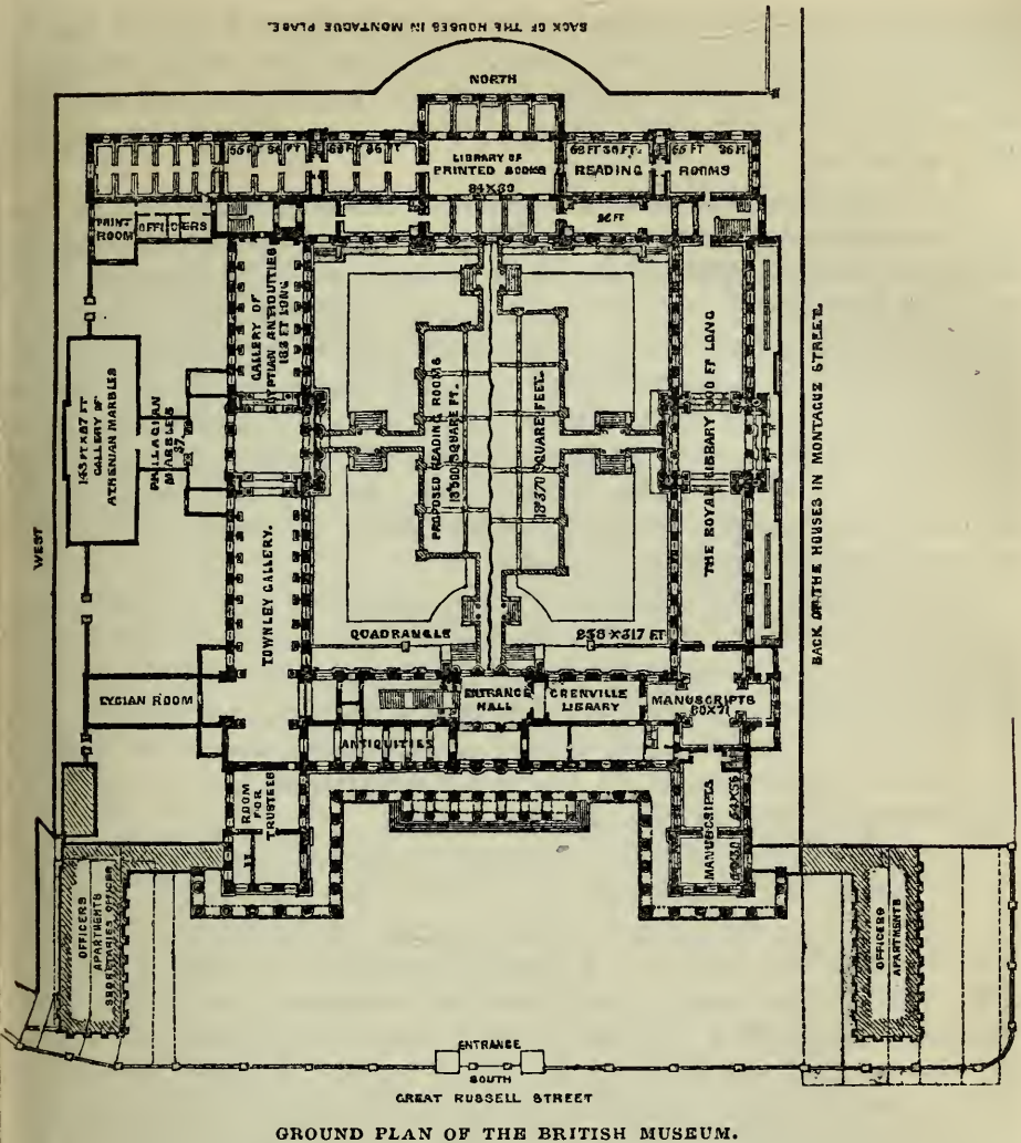
GROUND PLAN OF THE BRITISH MUSEUM.
