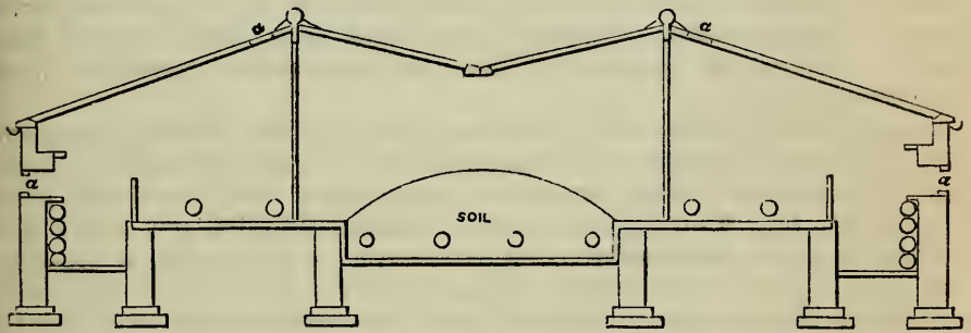
SECTION OF THE FORCING HOUSE.
