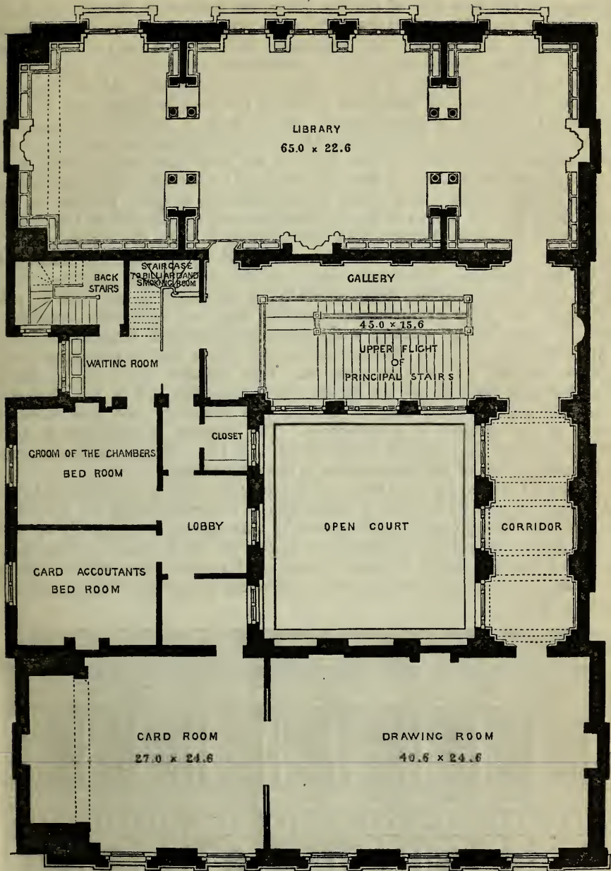
PLAN OF TRAVELLERS' CLUB-HOUSE.
