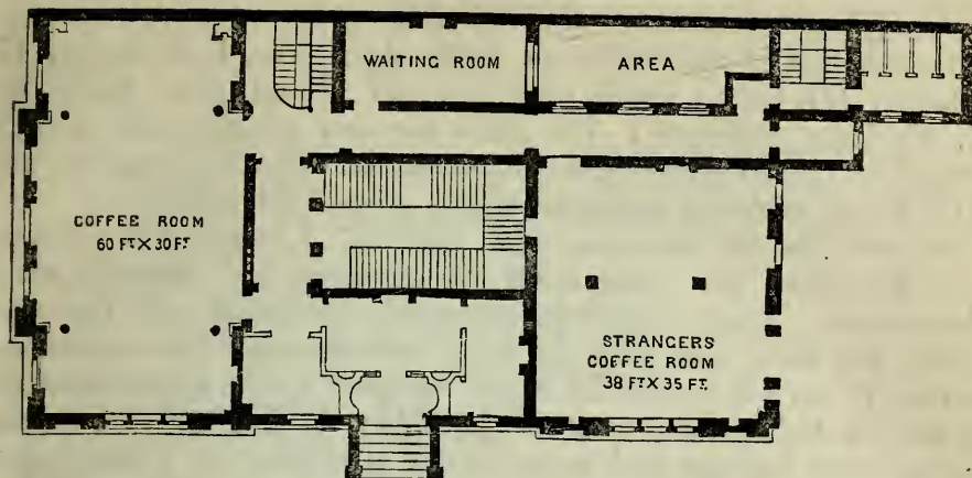
PLAN OF ORIENTAL CLUB-HOUSE.
