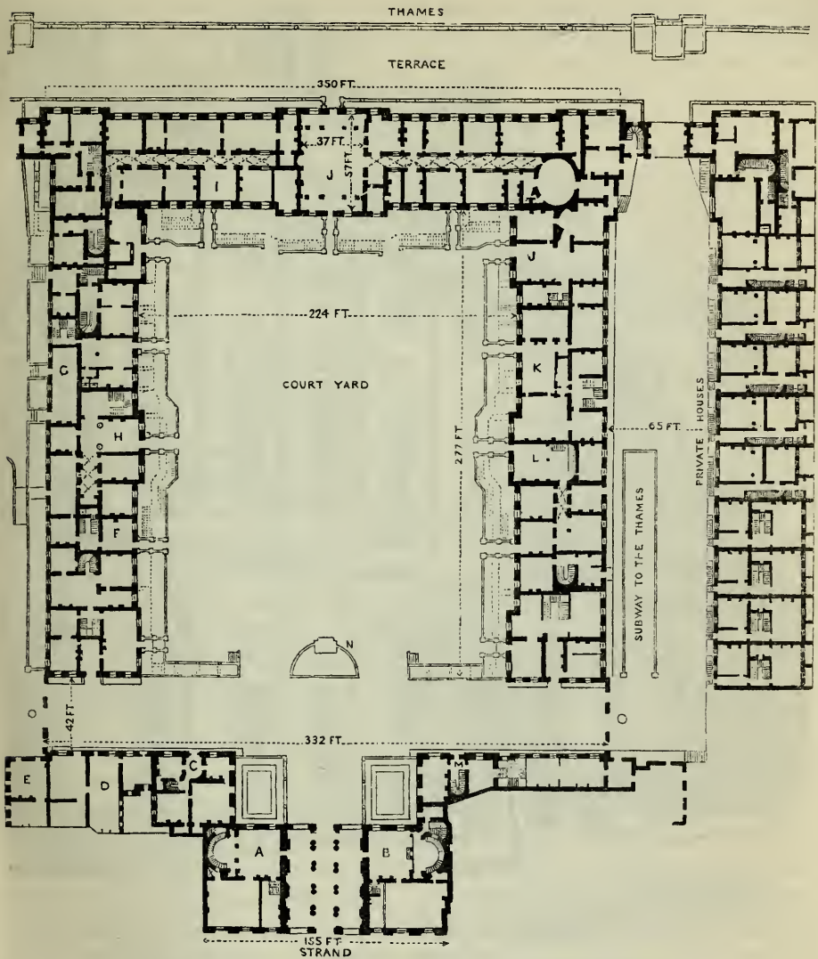
PLAN OF THE CENTRE STRAND AND WEST WING OF SOMERSET HOUSE.
