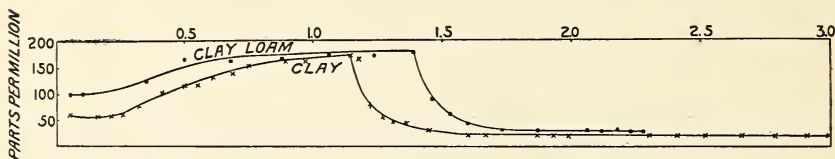
FIG. 5.—Solution curves. Absorption of potassium by soils from a solution of potassium chloride and the removal of the absorbed potassium by water.
