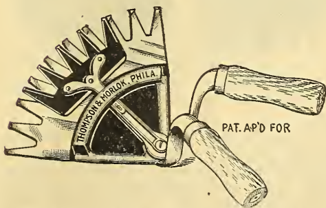
Showing the Little Wonder Hedge Trimmer working in a horizontal position
