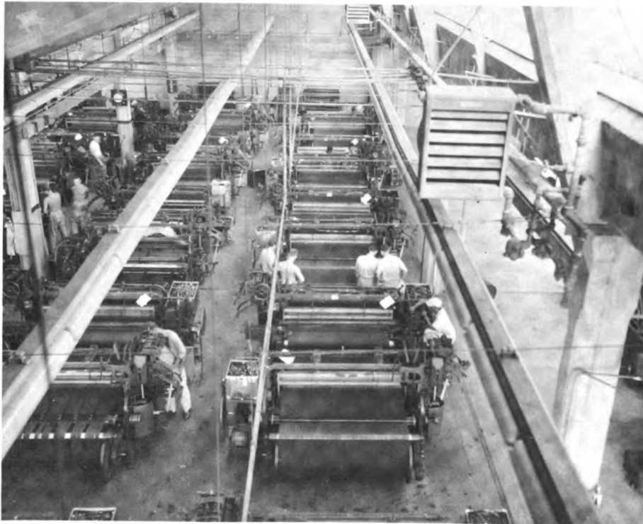
FIGURE 3. Looms in Terre Haute woolen mill.
