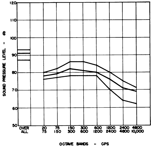
FIGURE 34. Octave band analyses, showing the median, 25th, and 75th percentile values for all departments in the printing plant at Leavenworth.
