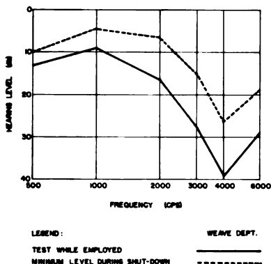
FIGURE 16. Average maximum recovery of temporary threshold shift, for stated frequencies, during 8-day period without noise exposure, of 30 employees from the weave department of the Atlanta cotton mill.
