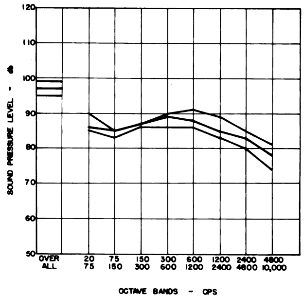
FIGURE 23. Octave band analyses, showing the median, 25th, and 75th percentile values for the twist department in the cotton mill at Atlanta.
