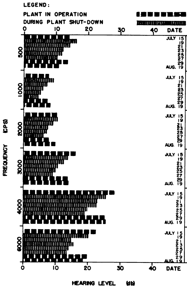
FIGURE 14. Average day-by-day recovery of temporary threshold shift, for stated frequencies, with time away from noise exposure, of 15 men after working 3 to 6 months in the spin, twist, and beam departments at the Atlanta cotton mill.
