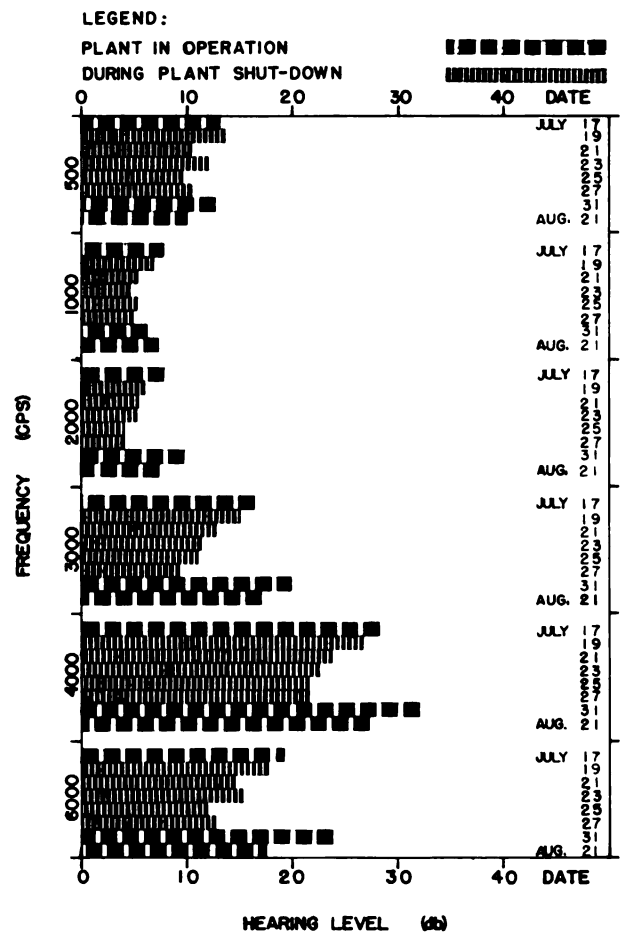
FIGURE 15. Average day-by-day recovery of temporary threshold shift, for stated frequencies, with time away from noise exposure, of 15 men after working 12 to 24 months in the spin, twist, and beam departments at the Atlanta cotton mill.
