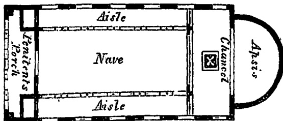
Plan of the Sessorian Basilica, afterwards the Church of the Holy Cross of Jerusalem.
