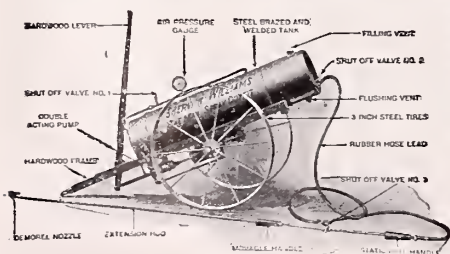
One-Man Compressed-Air Hand-Power Spray Pump
