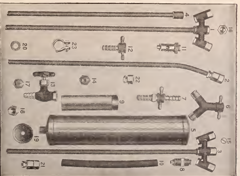
FITTING FOR PARAGON SPRAYERS. These fittings can be obtained from any dealer.
