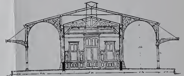
DWARSDOORSENE
