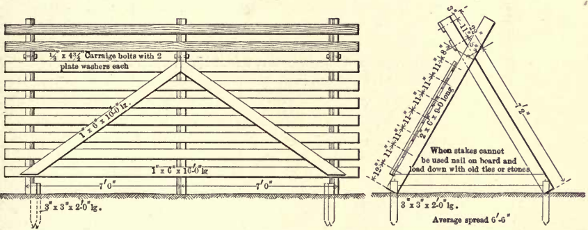
Fig. 14. Portable Snow Fence.
