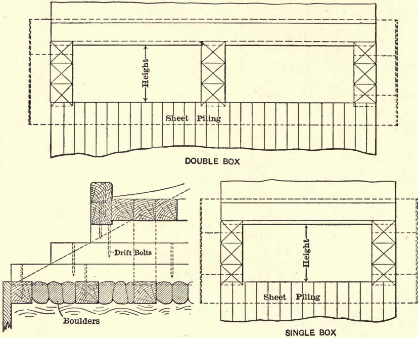
Fig. 23. Wood Box Culverts.
