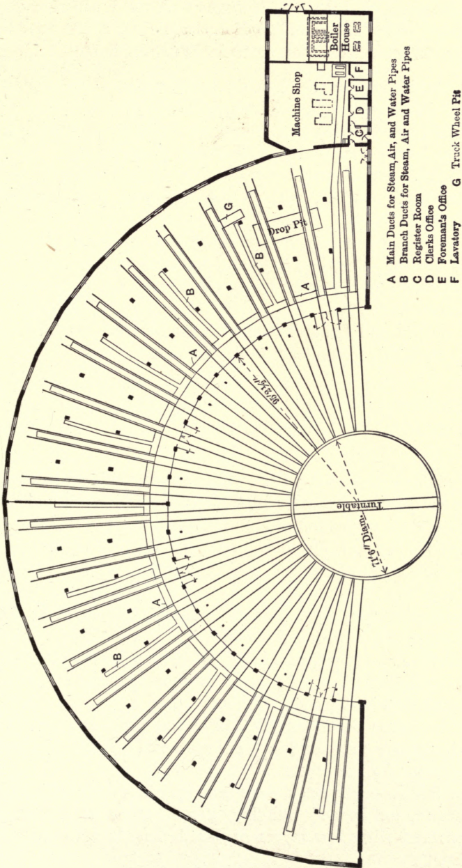
Fig. 58. General Layout, Engine House, etc.
