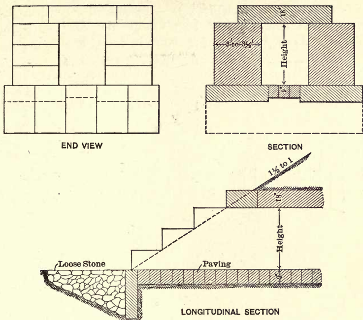
Fig. 22. Stone Box Culverts.
