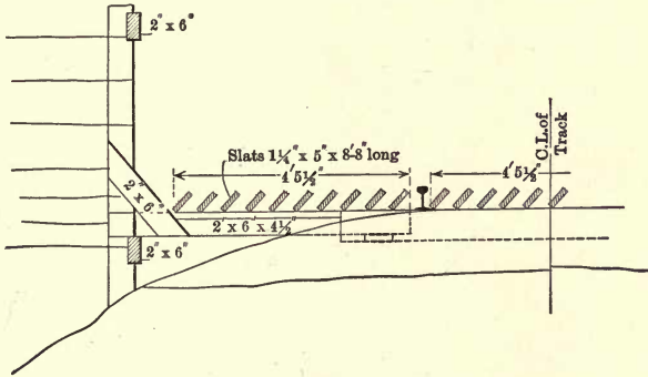
Fig. 18. Wood Cattle Guard.
