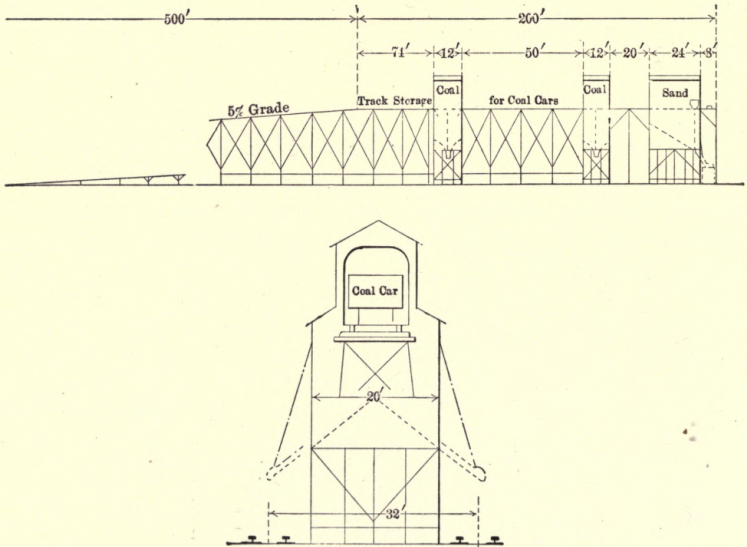
Fig. 72. Trestle Type Coaling Plant.
