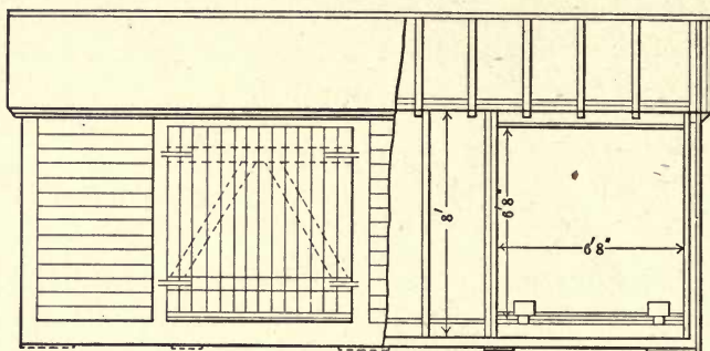
Double Tool House.
