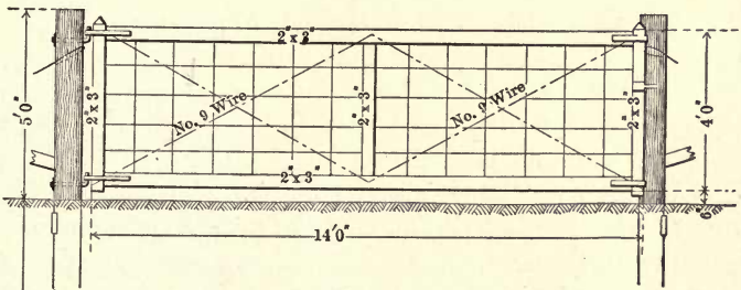
Fig. 16. Swing Wire Gate.
