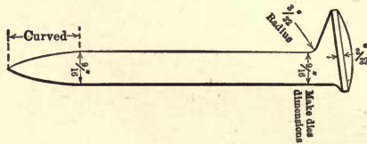
Fig. 4. Track Spike.
