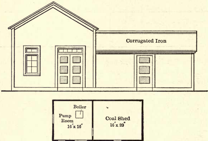
Fig. 89. Pump House.
