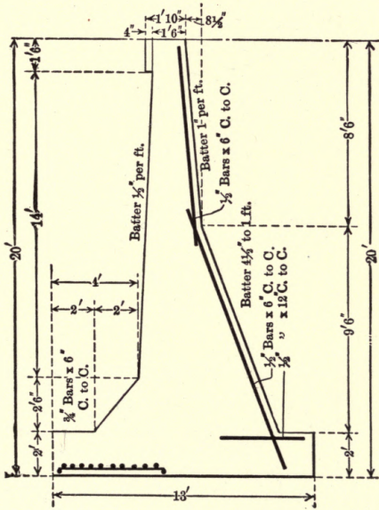
Fig. 38. Retaining Wall, C. B. & Q. Ry.
