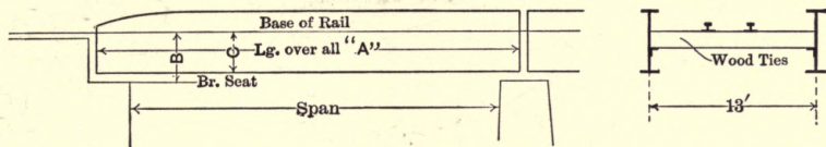
Fig. 25. Half Deck Plate Girders, 13 ft. centers.
