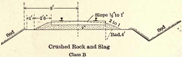
Fig. 5. Ballast Sections.
