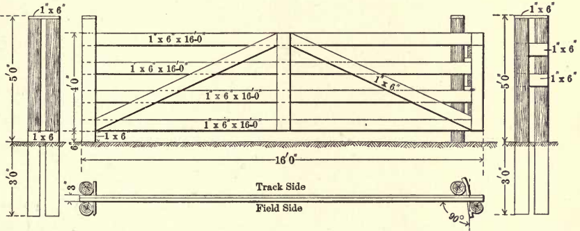
Fig. 15. Swing Board Gate.
