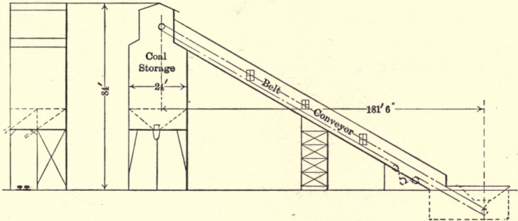
Fig. 70. Belt Conveyor Type of Coaling Plant.
