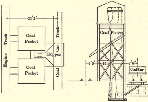
Fig. 66. Two-Pocket McHenry Coaling Plant.
