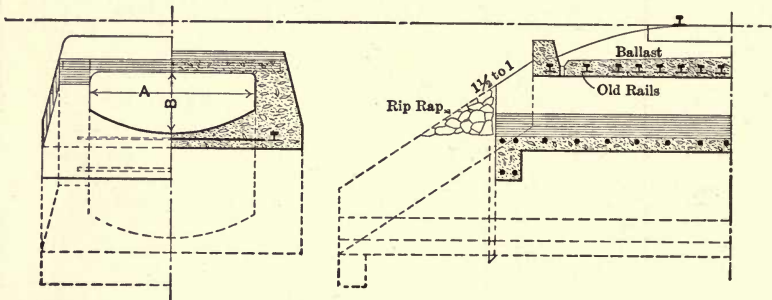
Fig. 21. Rail Concrete Culvert.
