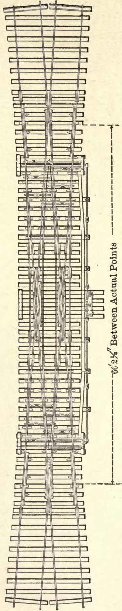
Fig. 11. Double Slip Switch.
