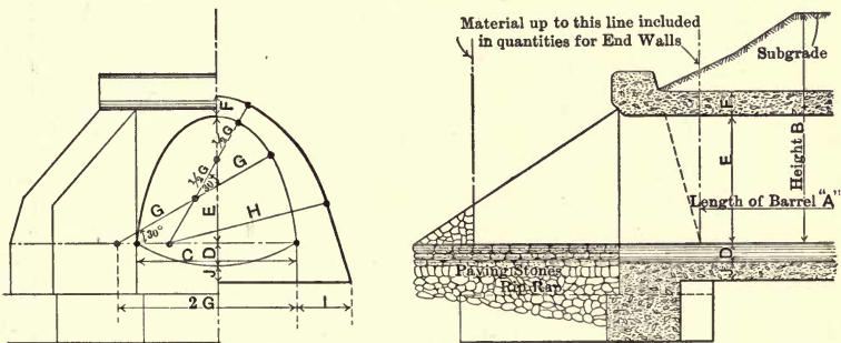
Fig. 20. Concrete Arch Culvert.
