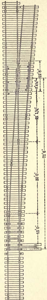
Fig. 6. Split Switch Turnout.
