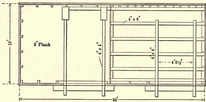
Double Tool House.
