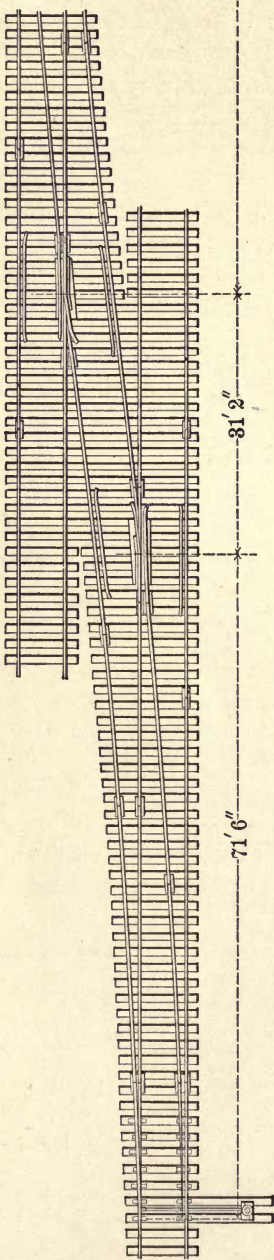
Fig. 10. Crossover.
