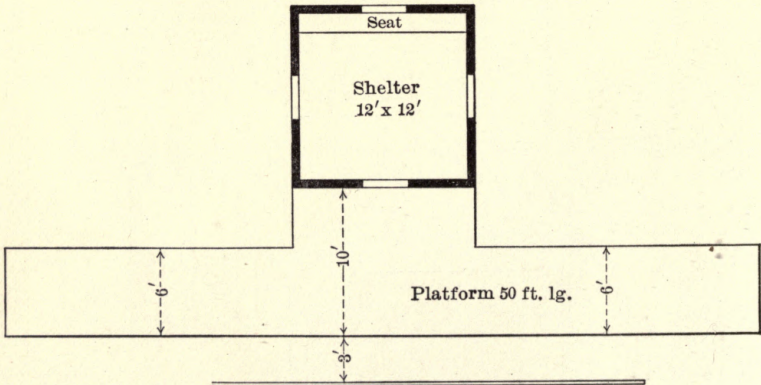
Fig. 48. Shelter Station.
