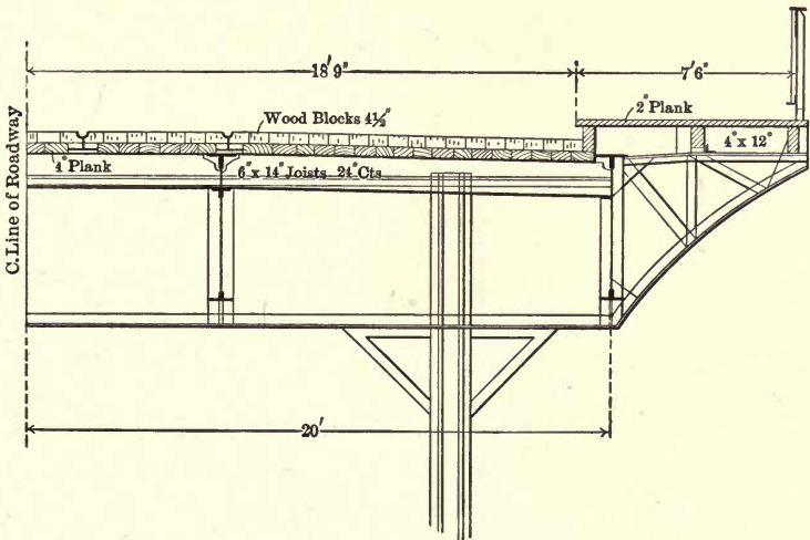
Fig. 33. Cross-Section Overhead Bridge.
