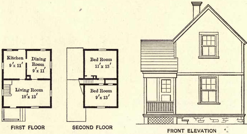
Fig. 45. Single Section House.
