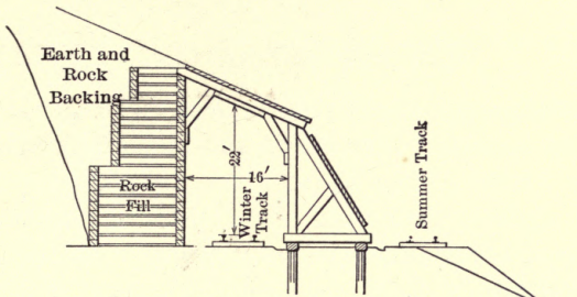
TYPICAL SHED Fig.83
