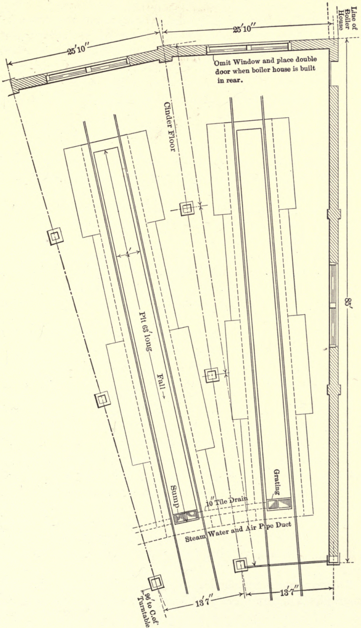
Fig. 58a. Engine House Plan.
