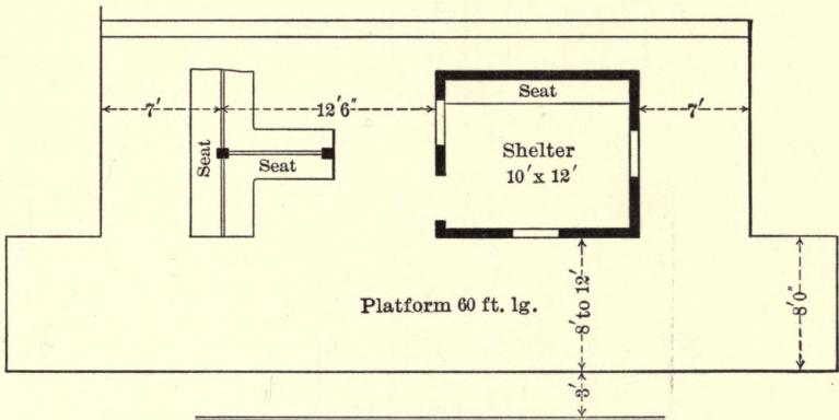
Fig. 49. Shelter Station.
