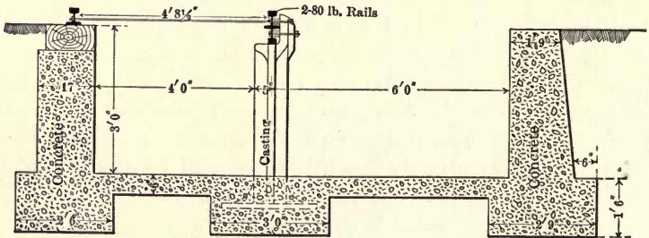
Fig. 76. Deep Open Ash Pit.
