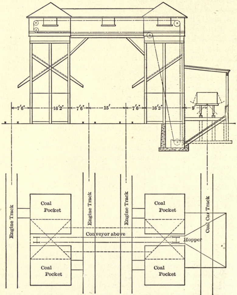
Fig. 68. Three-Track Coaling Plant.
