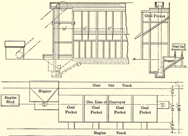
Fig. 67. Four-Pocket McHenry Coaling Plant.
