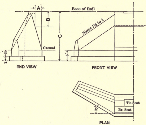
Fig. 29. Bridge Abutments.
