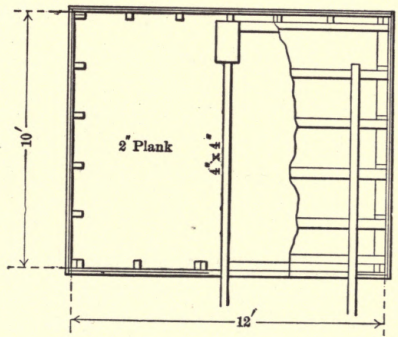
Plan Single House.
