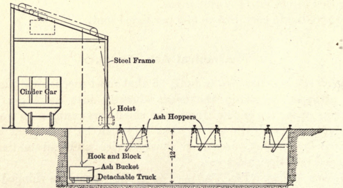
Fig. 80. Dump Bucket and Hoist.
