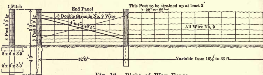
Fig. 12. Right of Way Fence.
