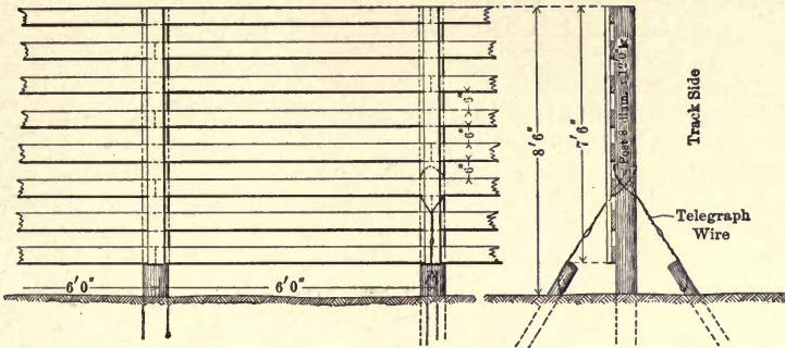
Fig. 13. Permanent Snow Fence. (Open Board.)
