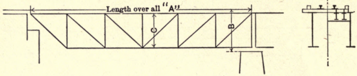
Fig. 26. Deck Lattice Rivetted Trusses.
