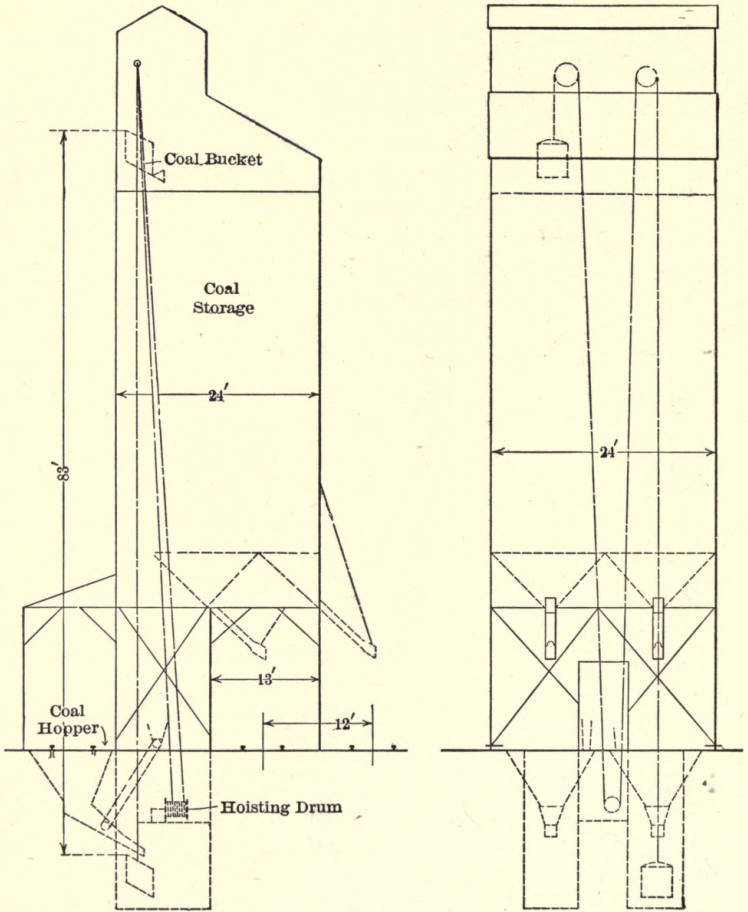
Fig. 69. Balanced Bucket Type Coaling Plant.
