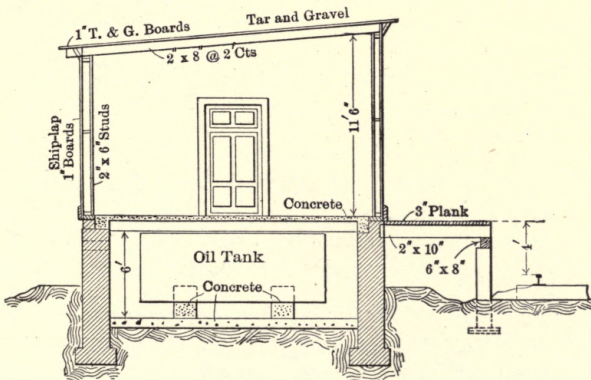
Fig. 63. Oil House.
