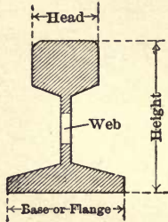
Fig. 1. Rail Section.
