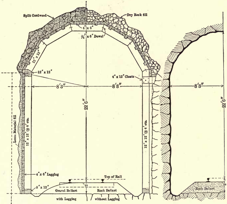
Figs. 41 and 42. Tunnels.
