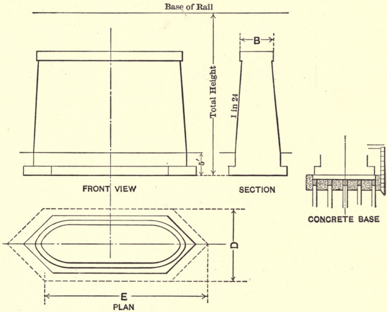
Fig. 29a. Bridge Piers.
