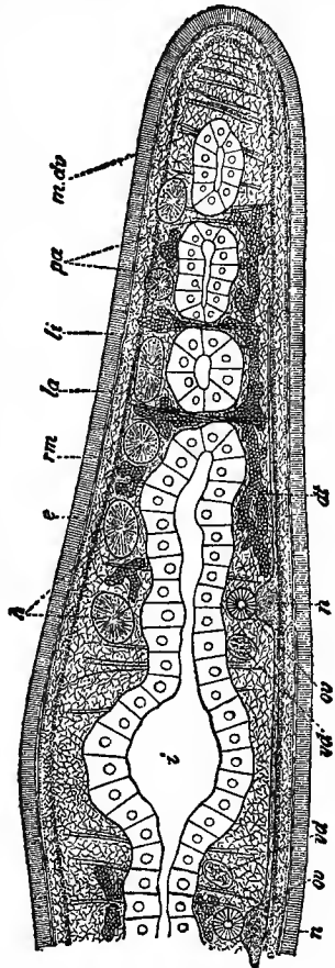
6. CROSS-SECTION OF TURBELLARIAN. HATSCHKE, FROM JIJIMA.
